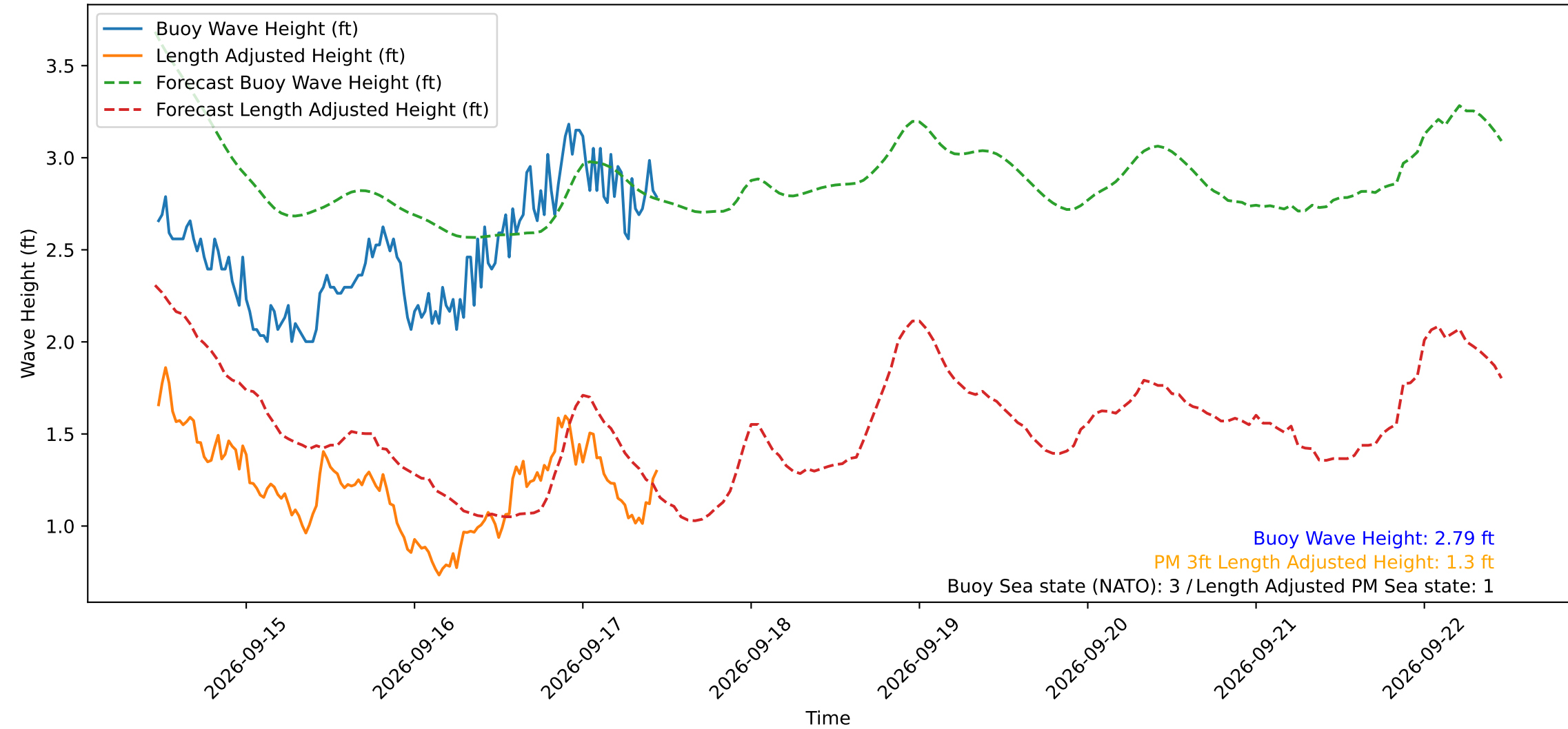
Wave Heights over Time for Red Beach at 2026-09-17 11:10:49
