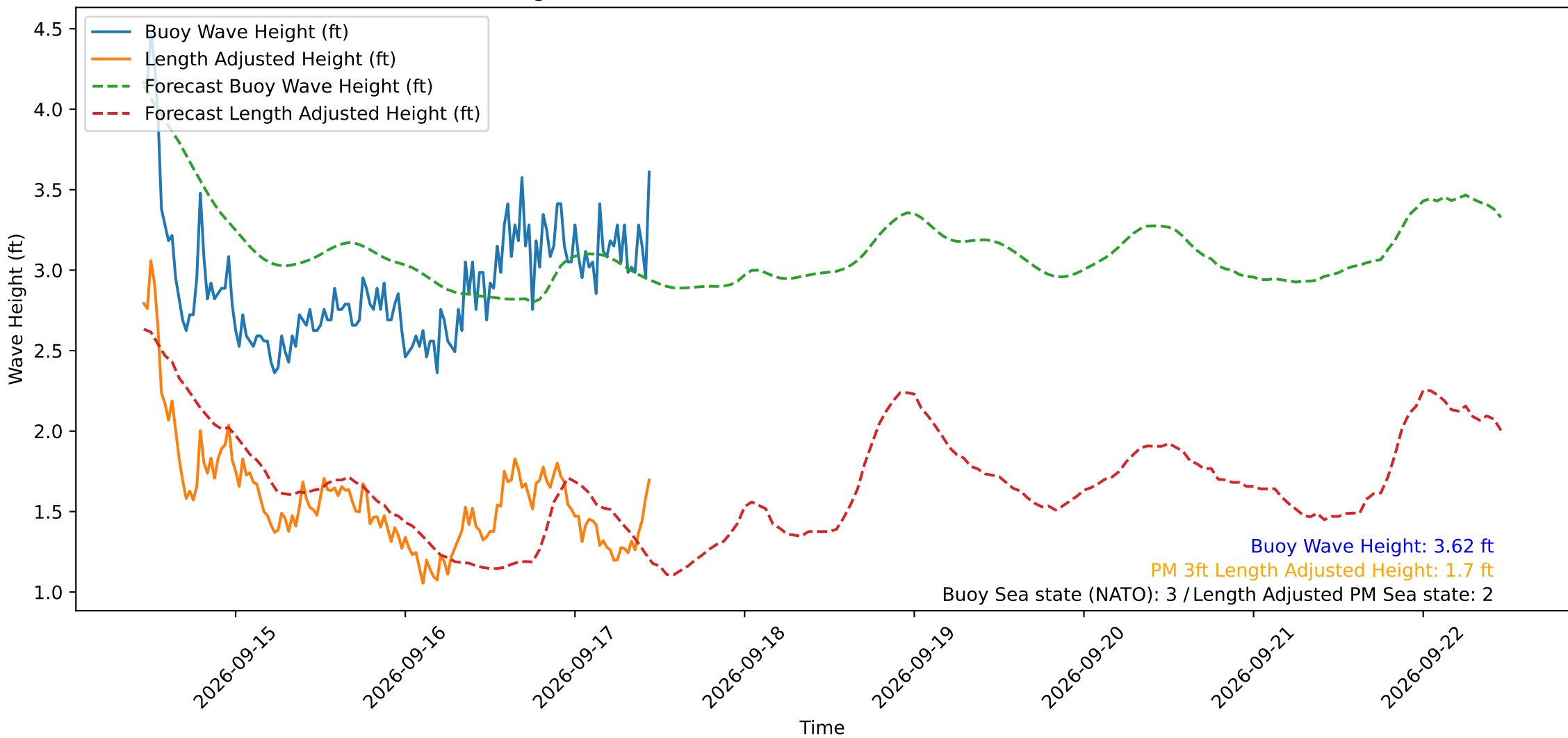
Wave Heights over Time for Oceanside Harbor at 2026-09-17 11:10:30
