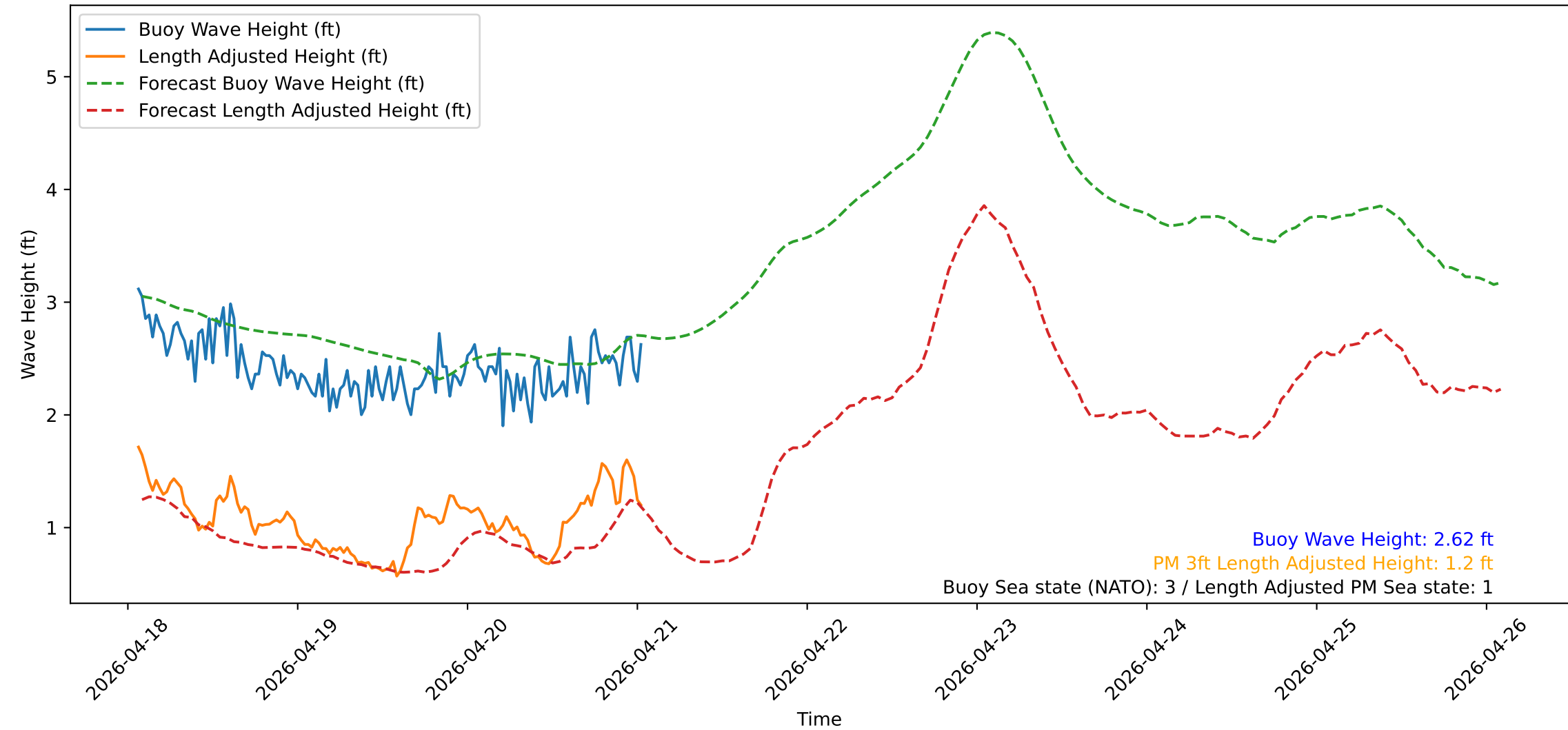
Wave Heights over Time for Oceanside Harbor at 2026-04-21 01:30:31
