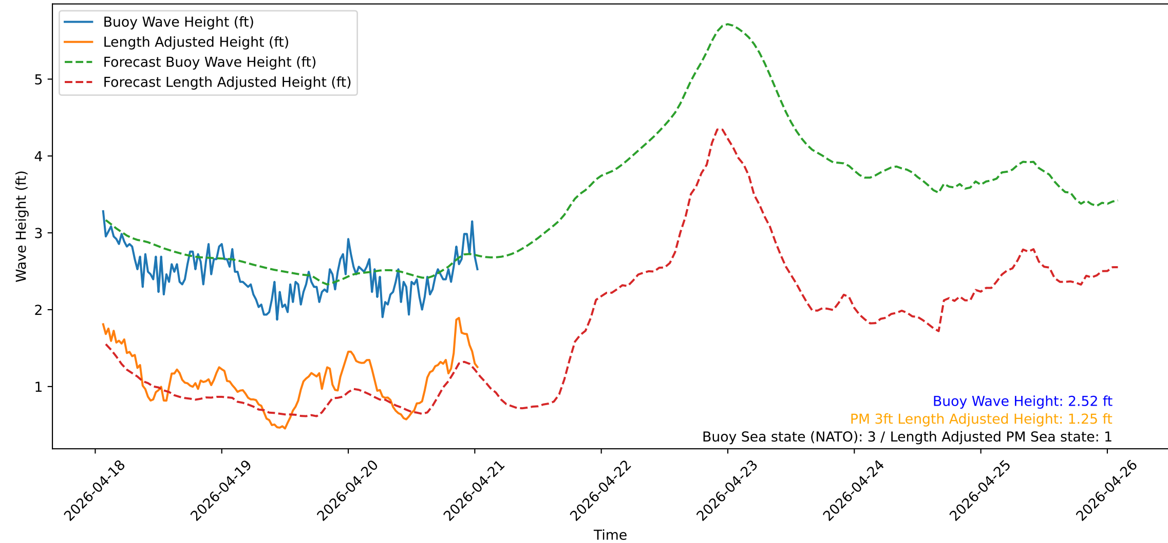
Wave Heights over Time for Green Beach at 2026-04-21 01:31:13
