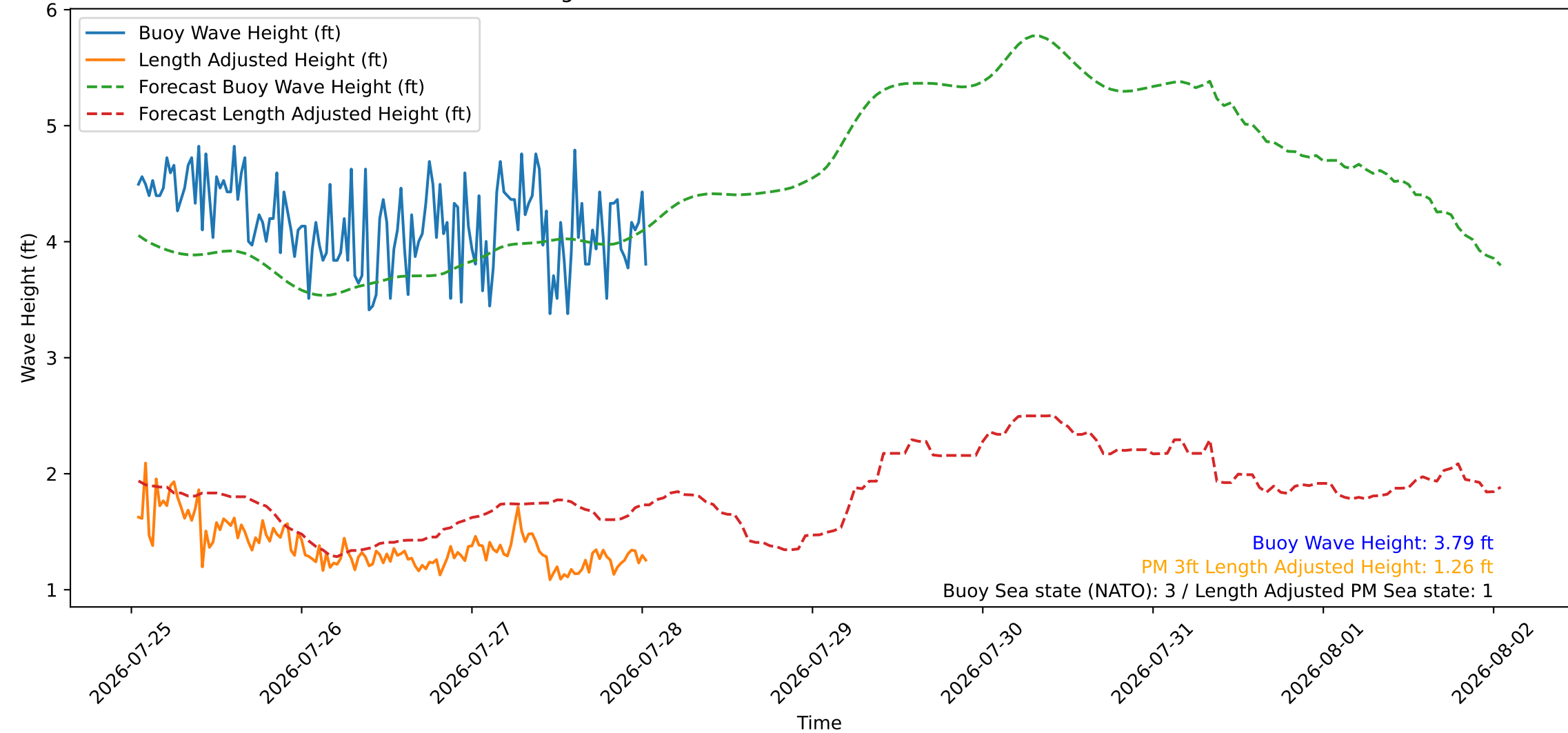
Wave Heights over Time for Green Beach at 2026-07-28 01:11:09
