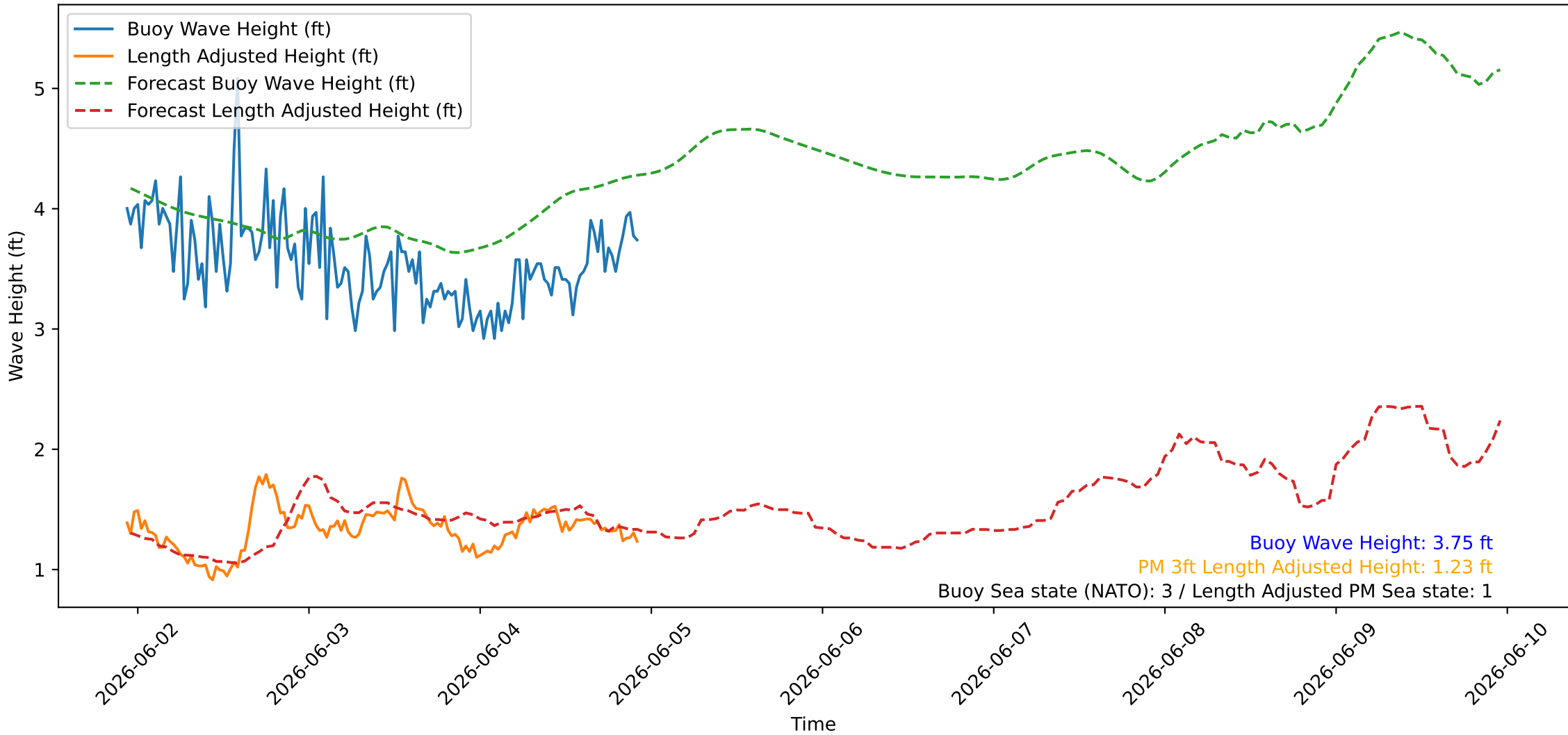
Wave Heights over Time for Oceanside Harbor at 2026-06-04 22:40:26
