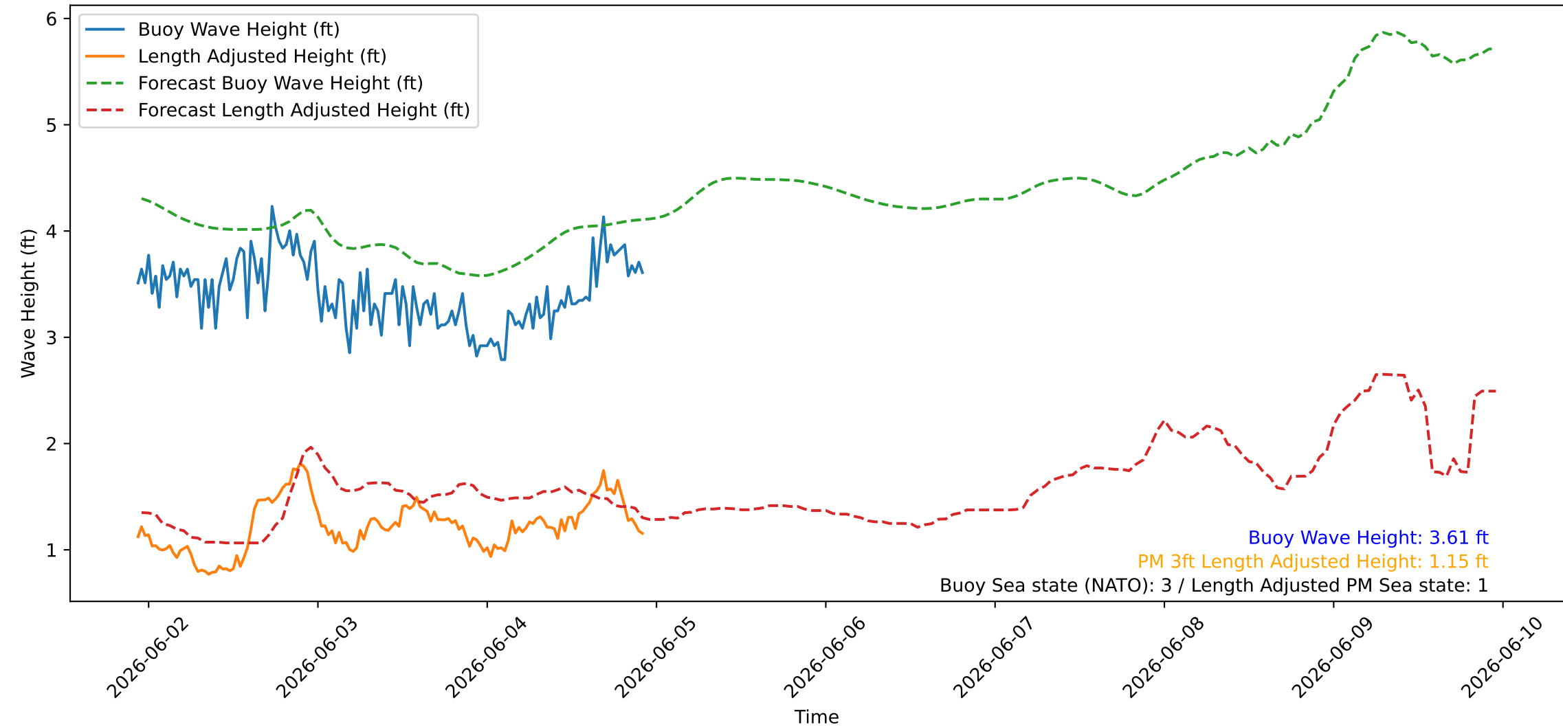
Wave Heights over Time for Green Beach at 2026-06-04 22:41:08
