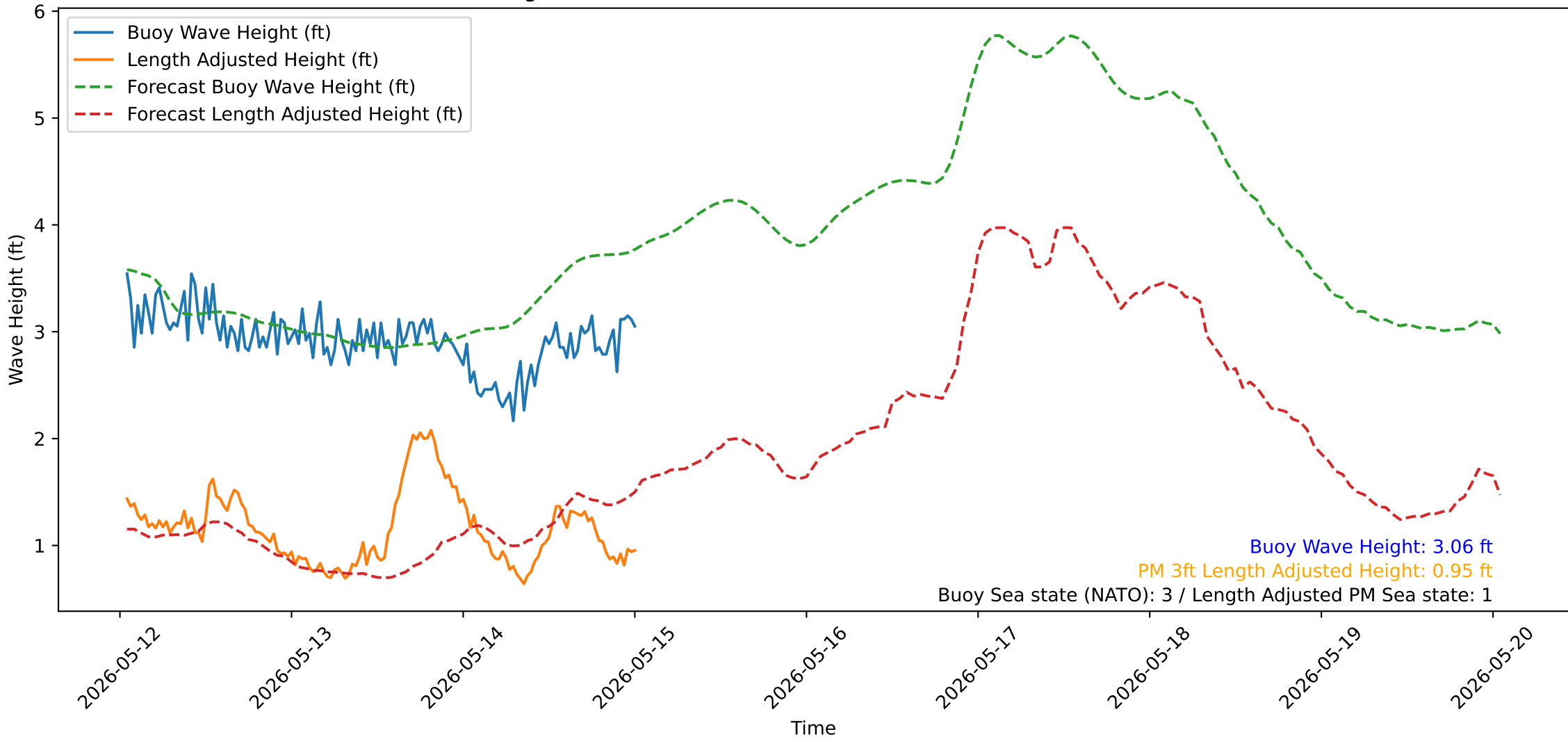
Wave Heights over Time for Oceanside Harbor at 2026-05-15 00:50:31
