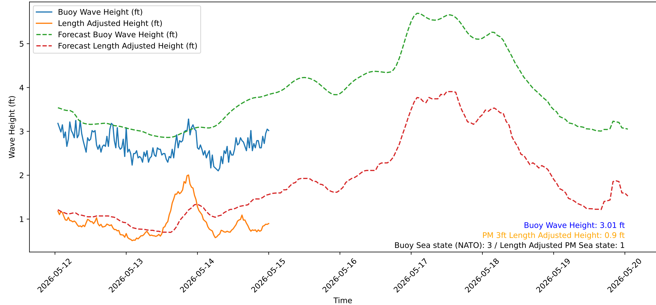
Wave Heights over Time for Green Beach at 2026-05-15 00:51:14
