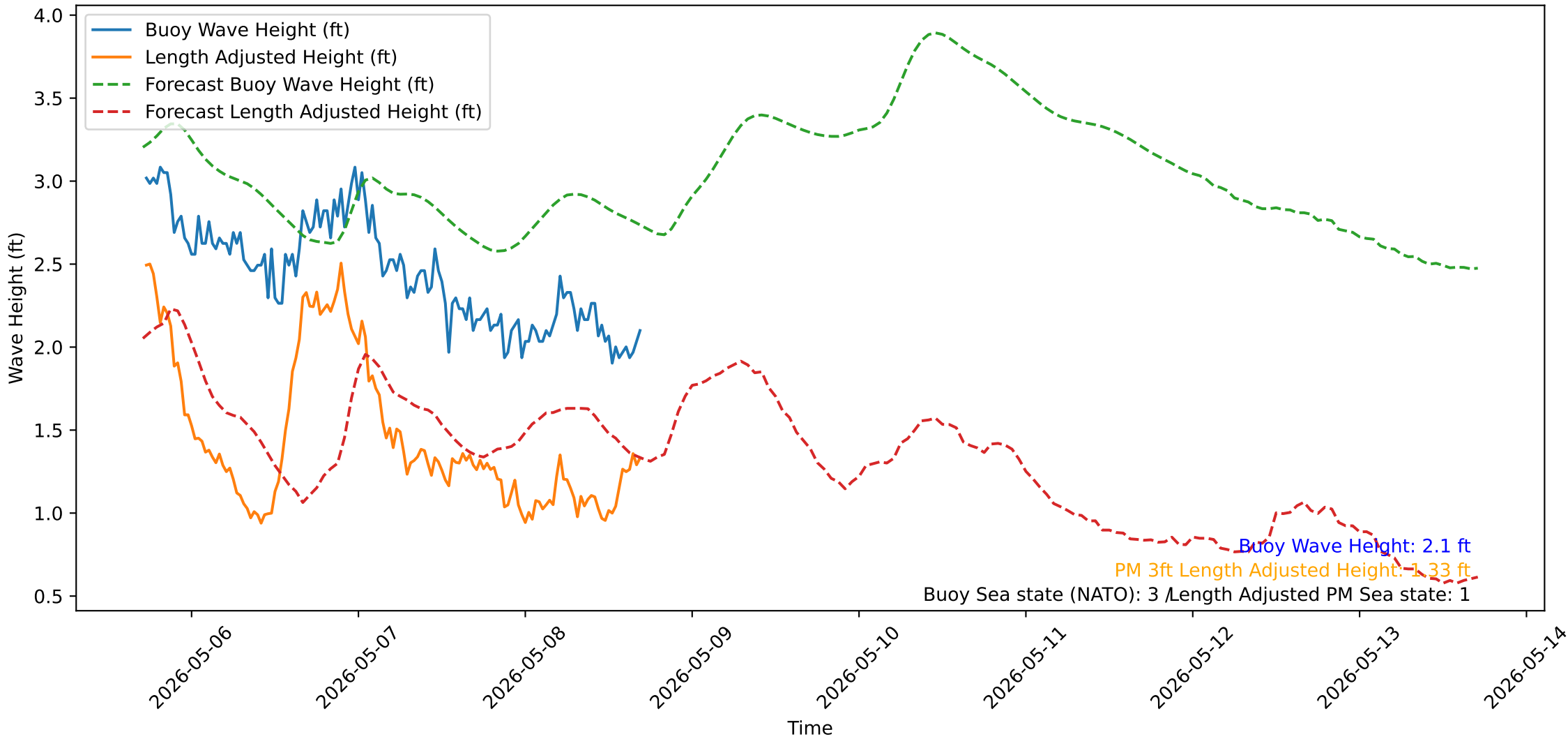
Wave Heights over Time for Red Beach at 2026-05-08 17:20:52
