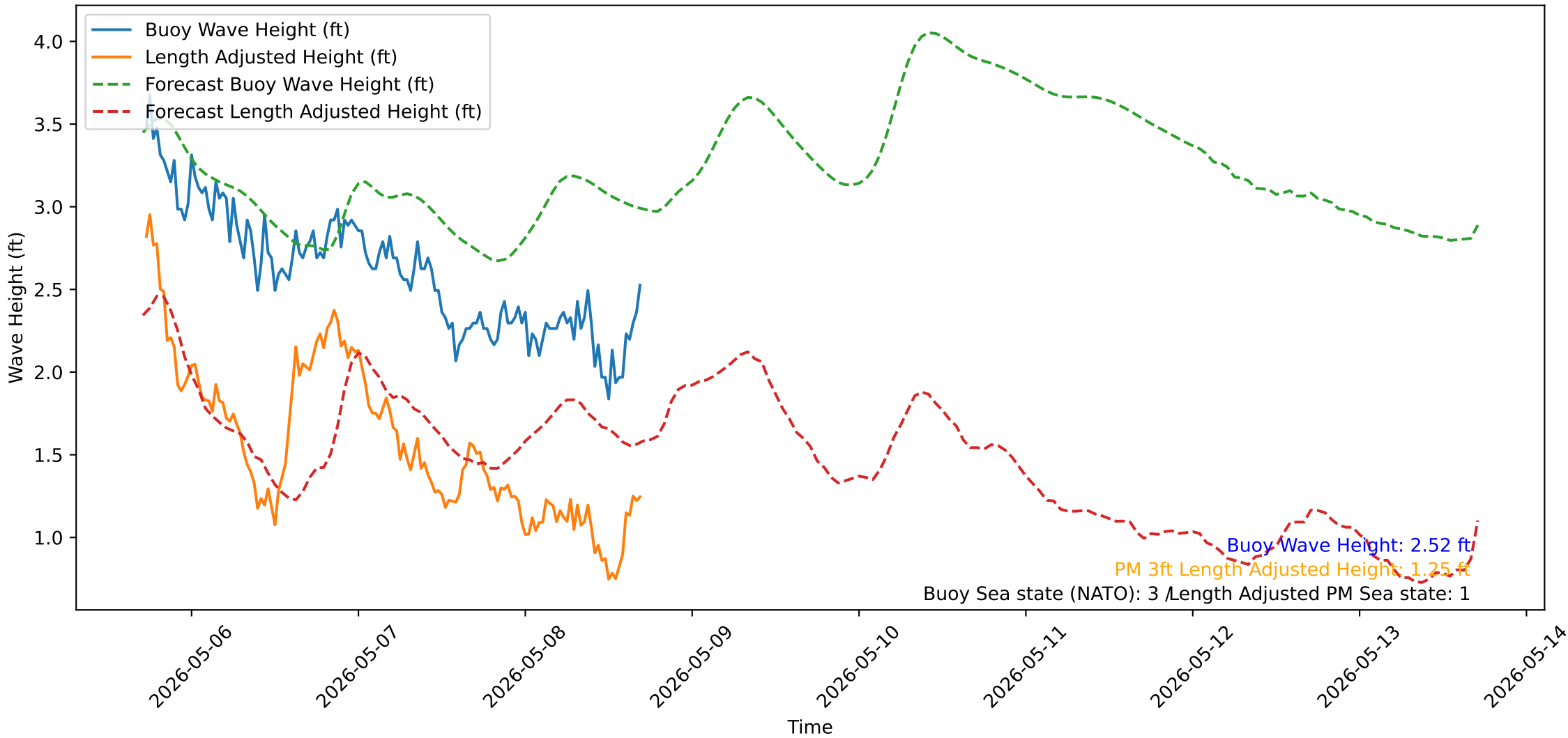
Wave Heights over Time for Green Beach at 2026-05-08 17:21:14
