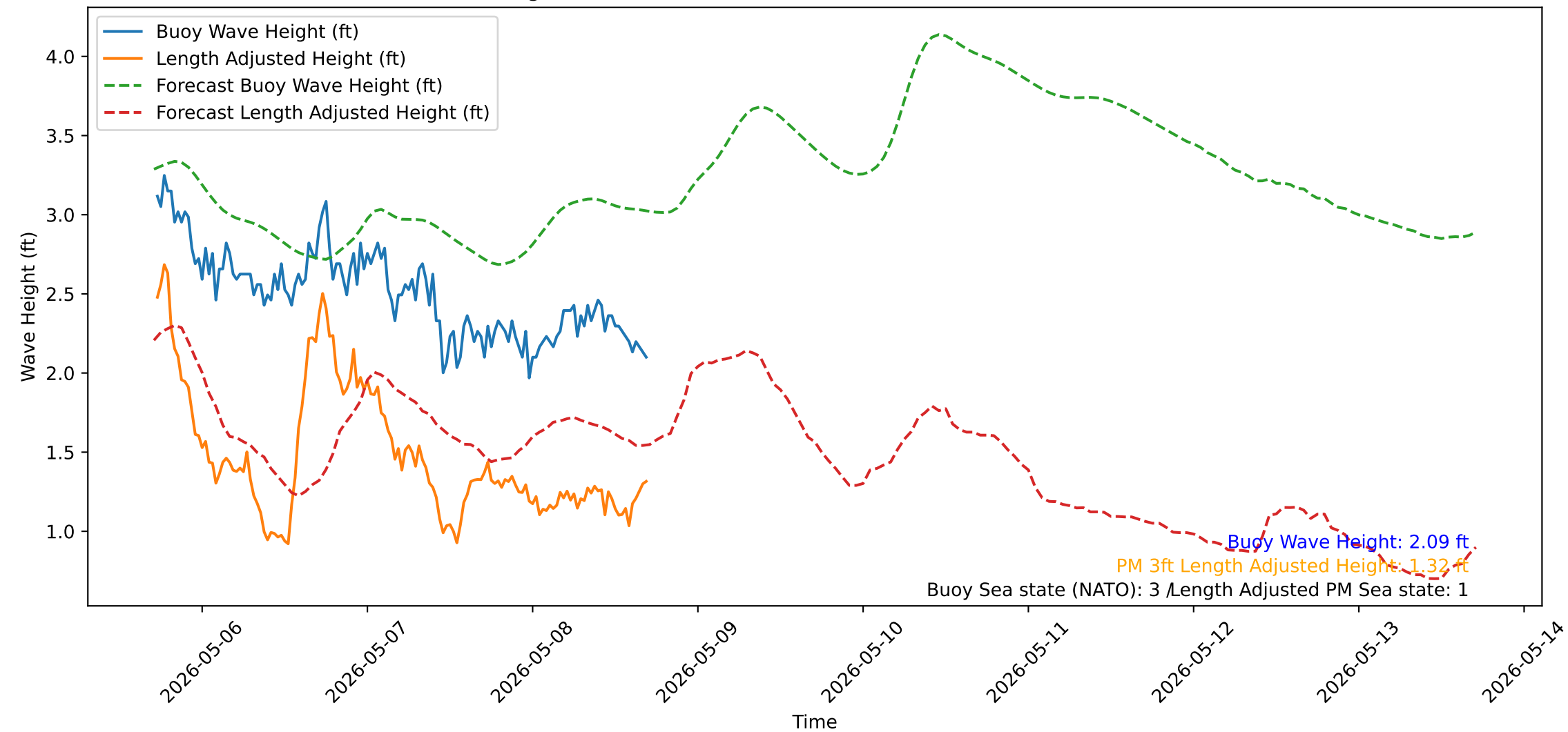
Wave Heights over Time for Oceanside Harbor at 2026-05-08 17:20:31
