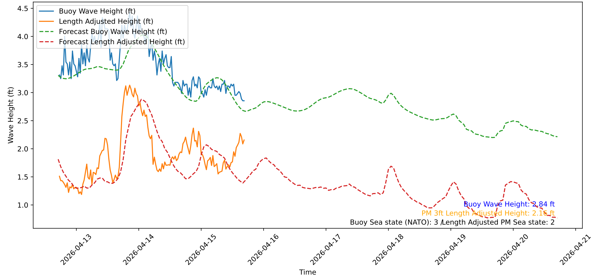
Wave Heights over Time for Red Beach at 2026-04-15 17:10:51
