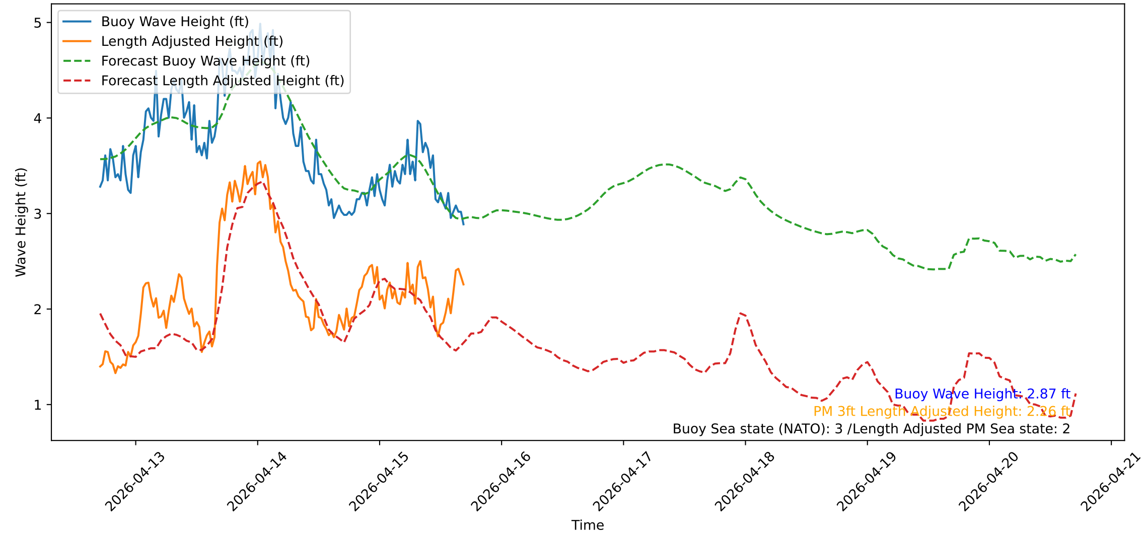
Wave Heights over Time for Green Beach at 2026-04-15 17:11:13
