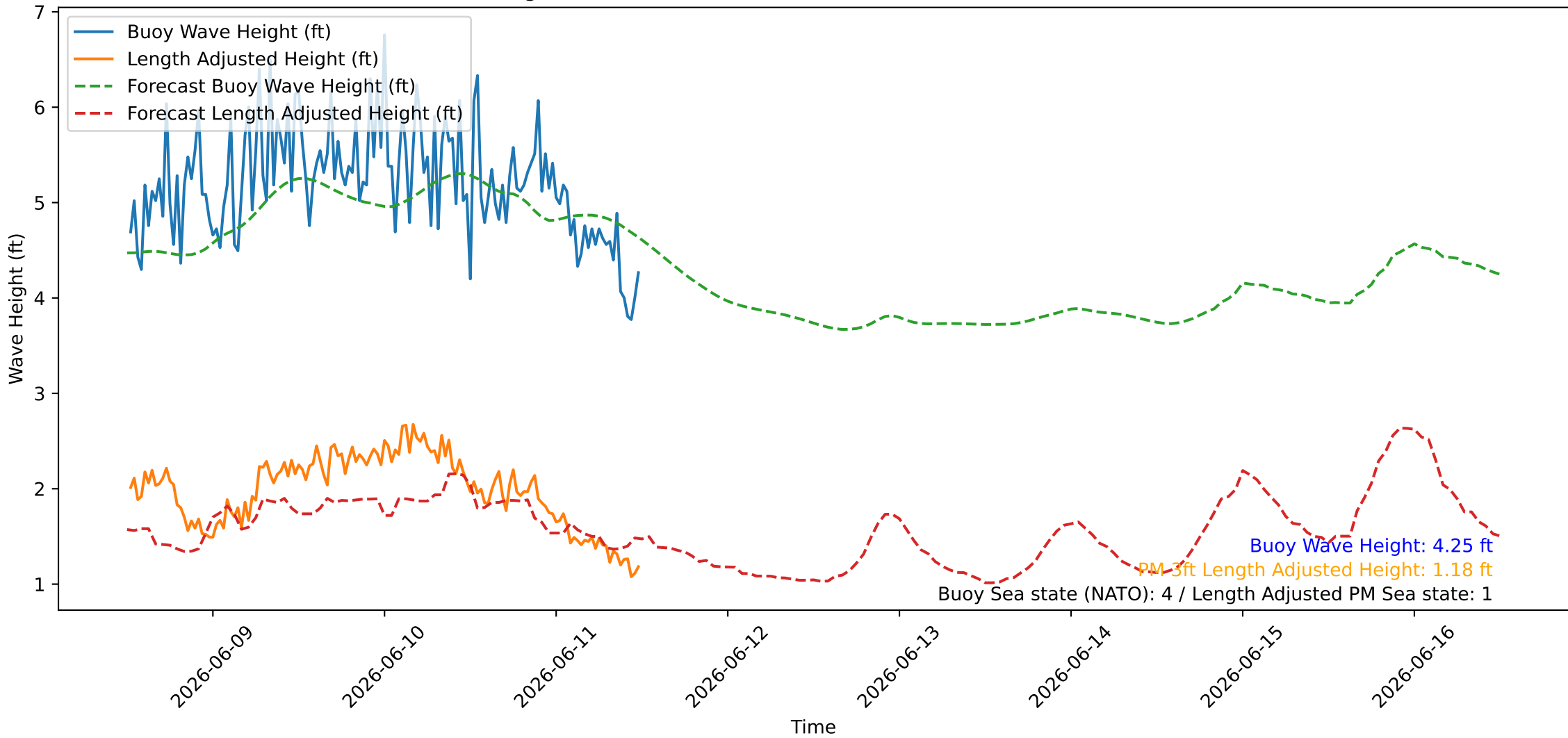
Wave Heights over Time for Oceanside Harbor at 2026-06-11 12:20:26
