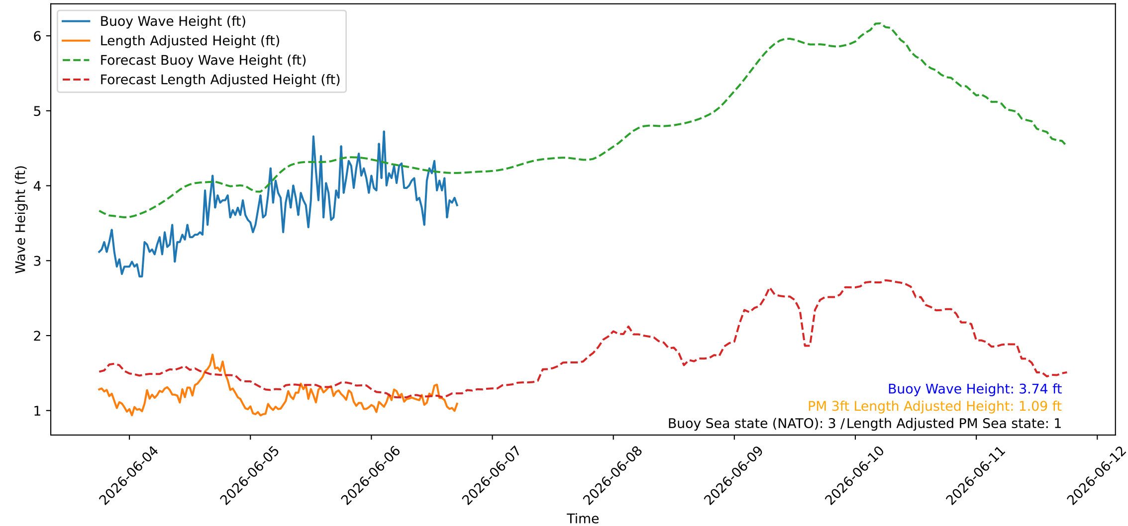
Wave Heights over Time for Green Beach at 2026-06-06 17:51:10
