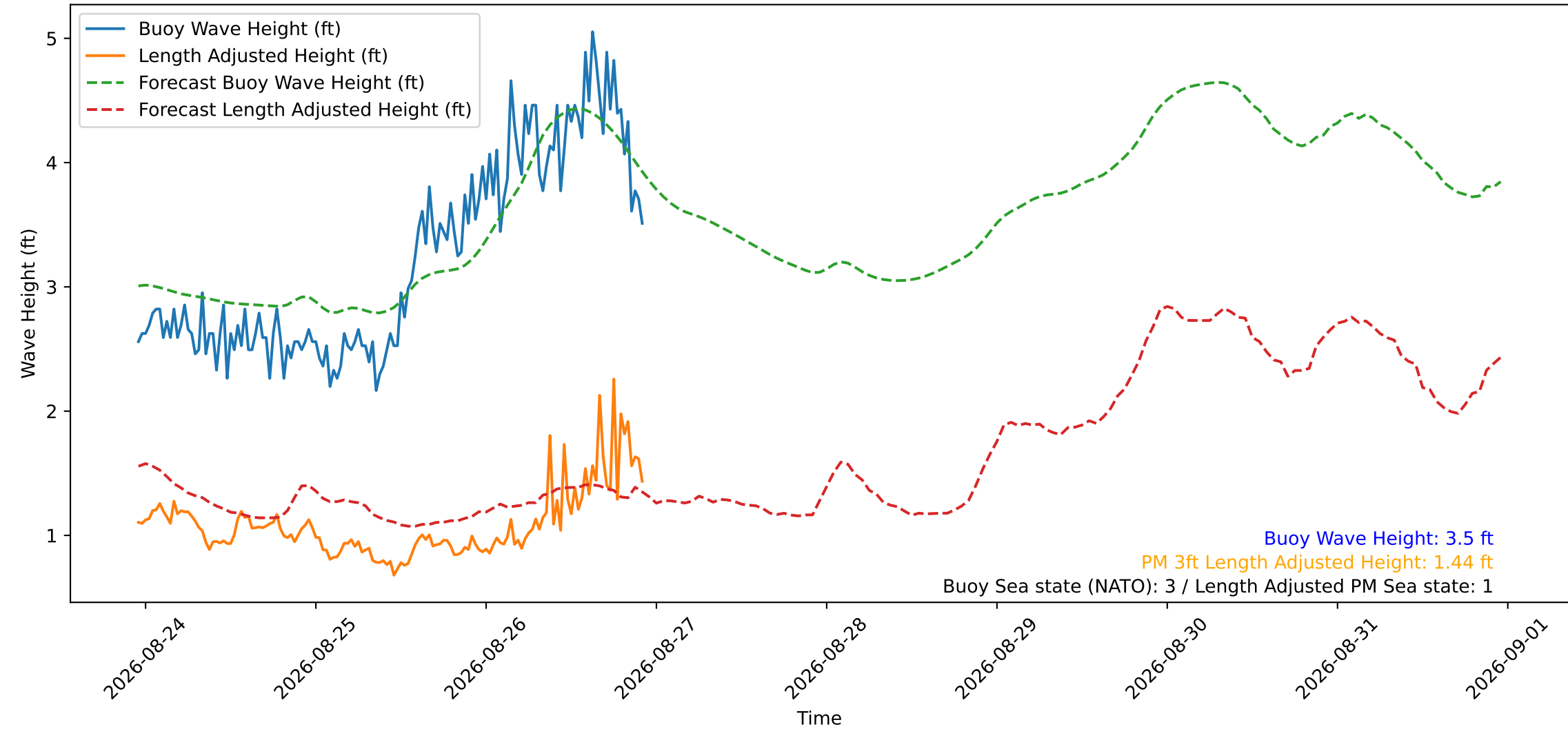
Wave Heights over Time for Red Beach at 2026-08-26 22:40:49
