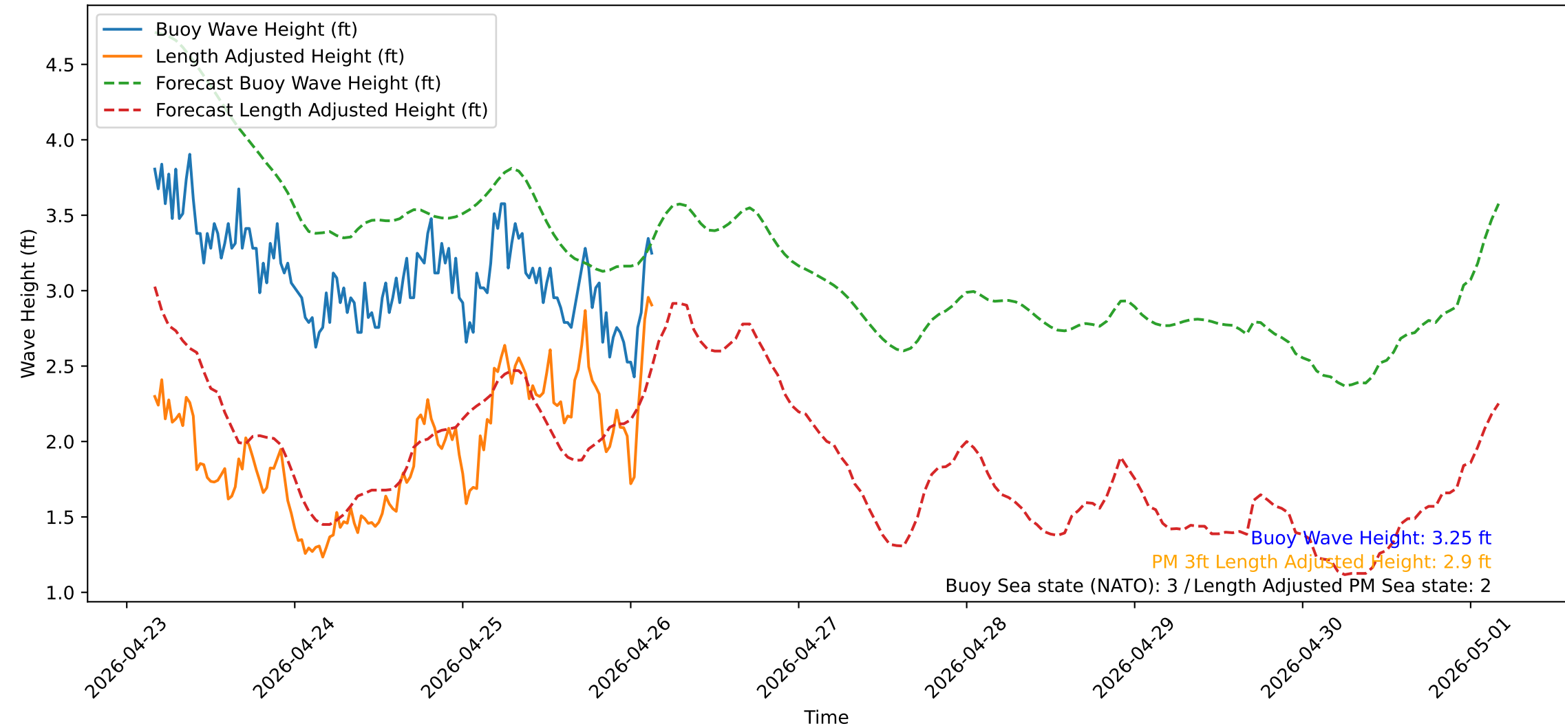
Wave Heights over Time for Green Beach at 2026-04-26 03:51:13
