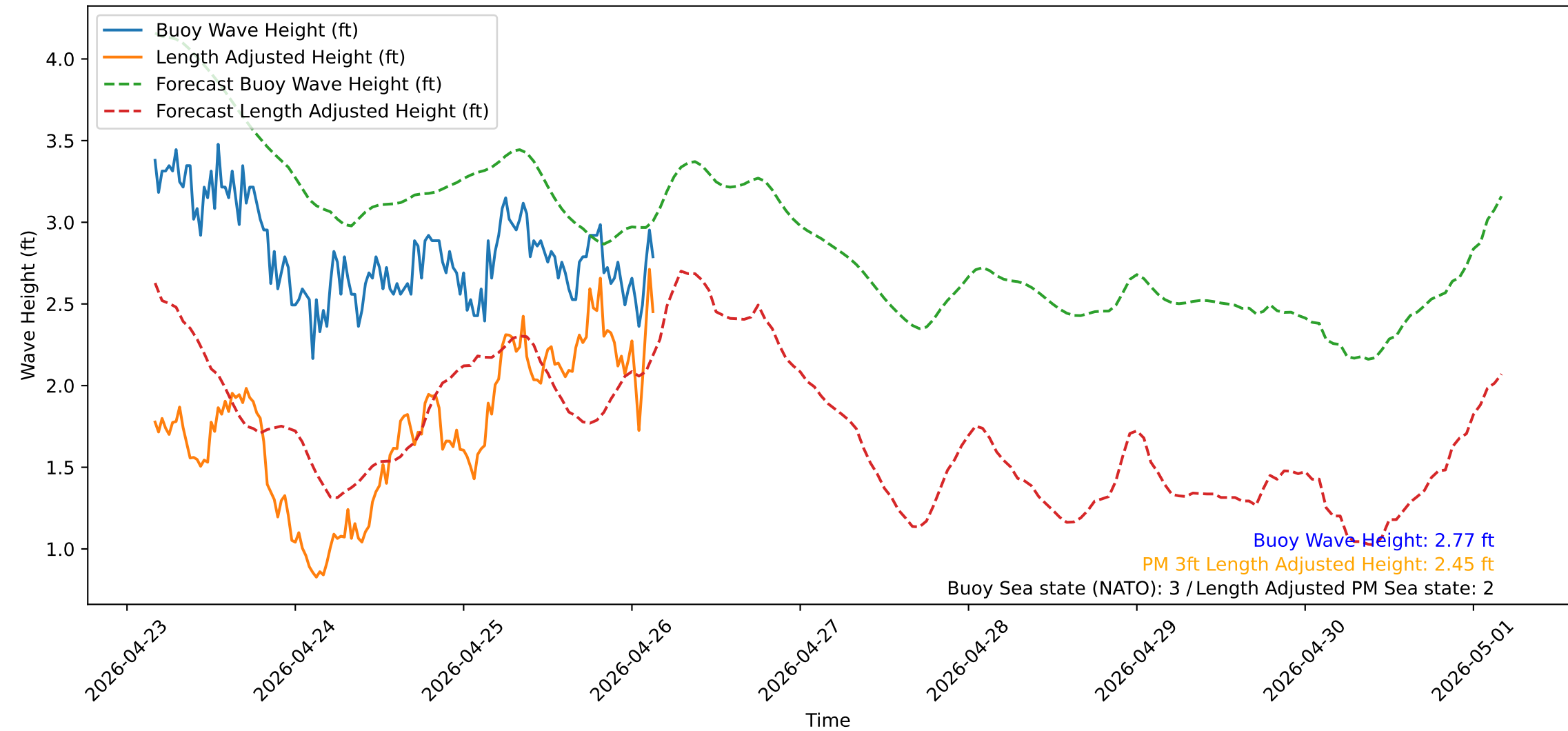
Wave Heights over Time for Red Beach at 2026-04-26 03:50:51
