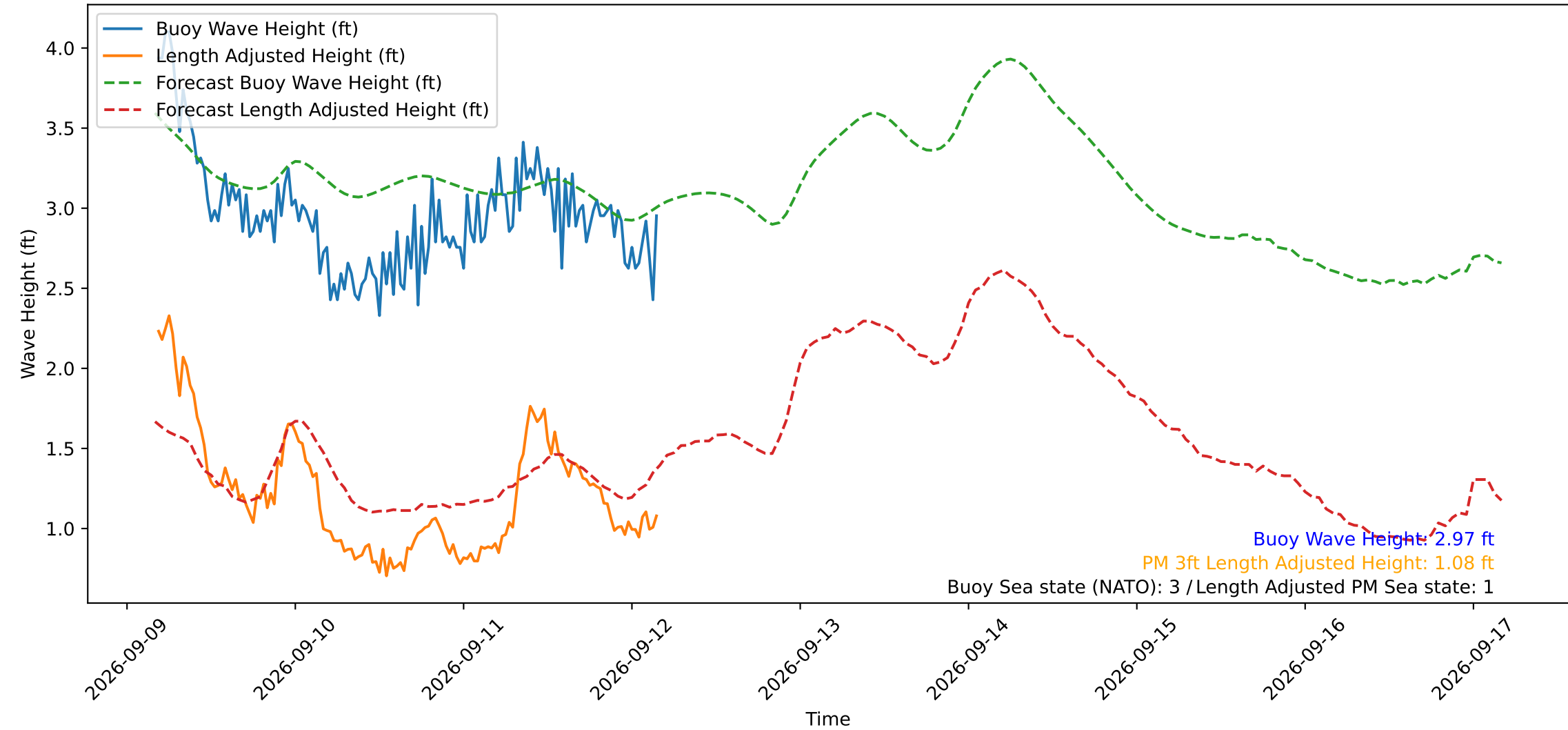
Wave Heights over Time for Red Beach at 2026-09-12 04:20:51
