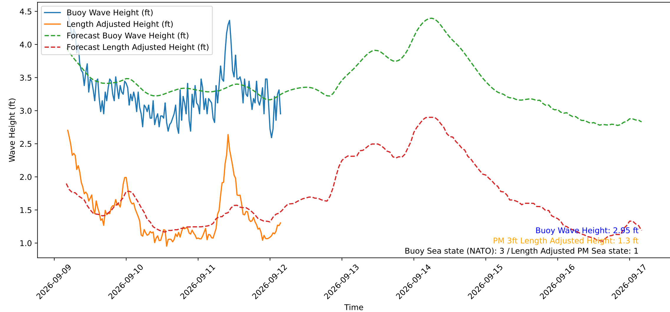
Wave Heights over Time for Oceanside Harbor at 2026-09-12 04:20:30
