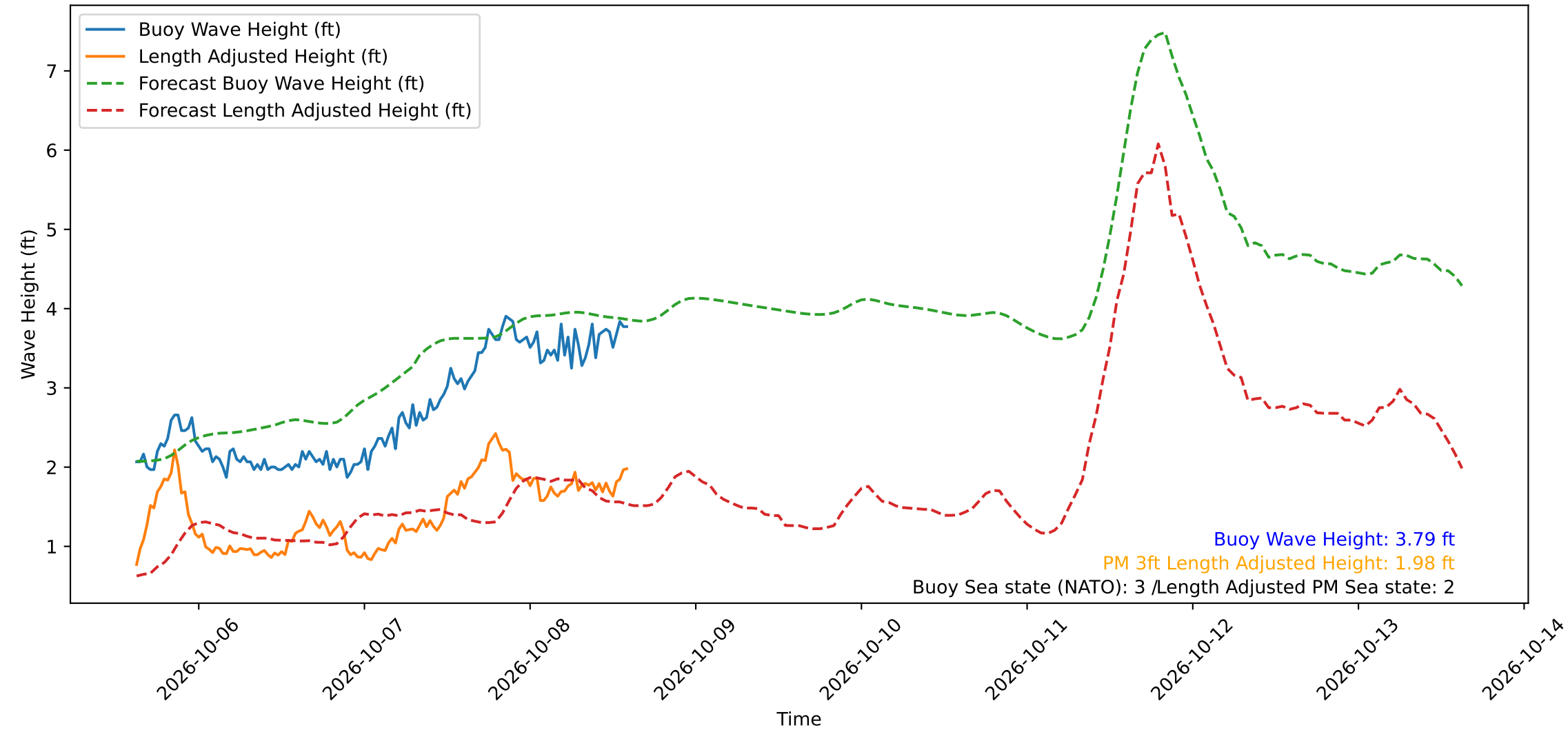
Wave Heights over Time for Red Beach at 2026-10-08 14:40:49
