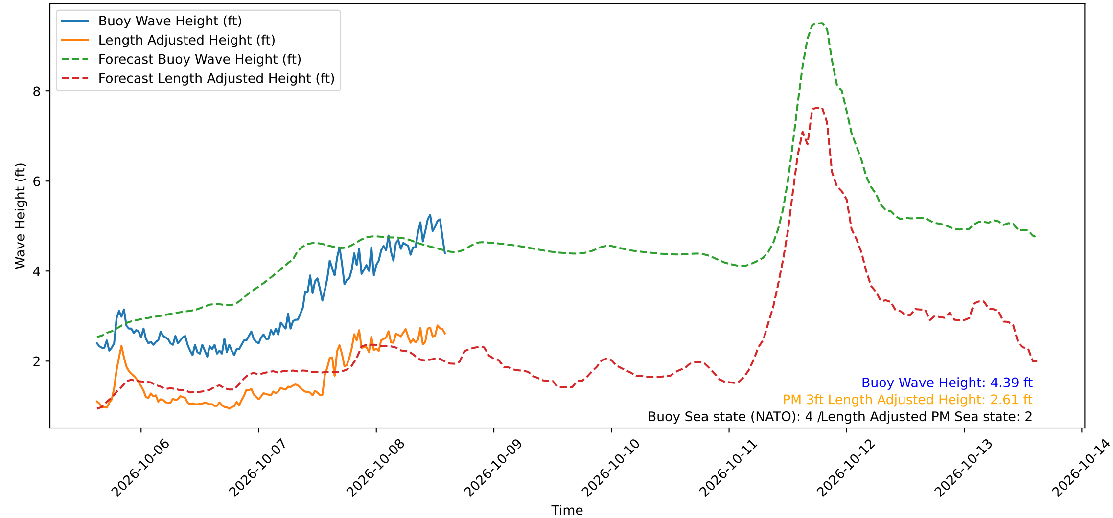
Wave Heights over Time for Green Beach at 2026-10-08 14:41:11
