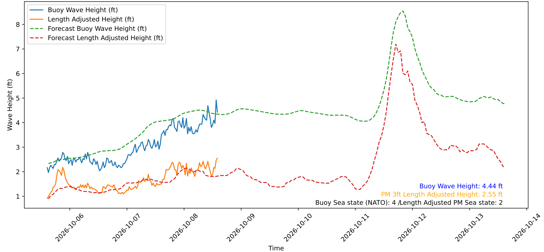
Wave Heights over Time for Oceanside Harbor at 2026-10-08 14:40:29
