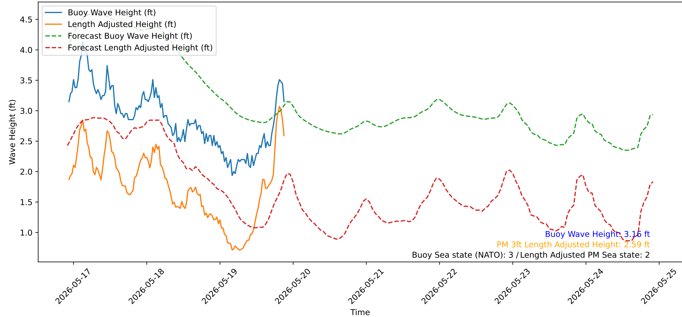
Wave Heights over Time for Red Beach at 2026-05-19 22:00:51
