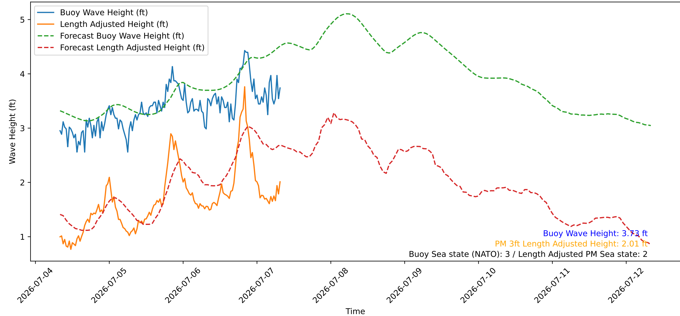
Wave Heights over Time for Green Beach at 2026-07-07 08:11:08
