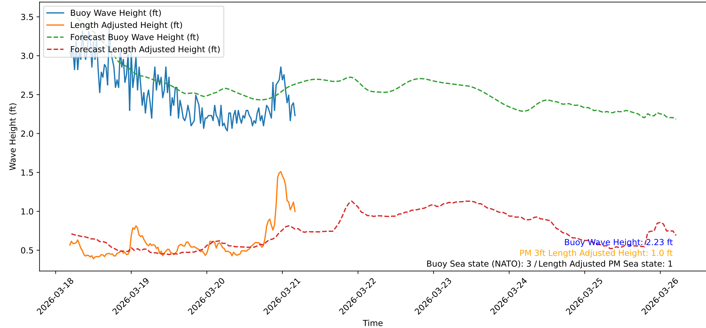
Wave Heights over Time for Green Beach at 2026-03-21 04:41:11
