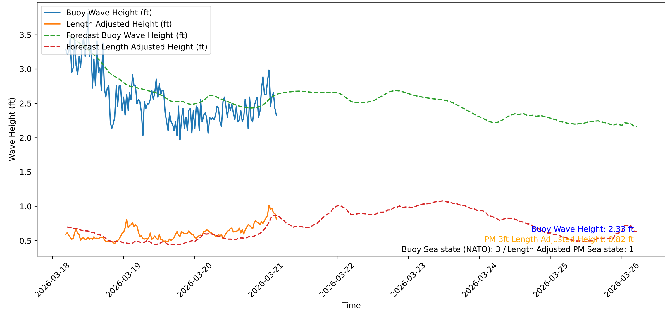
Wave Heights over Time for Oceanside Harbor at 2026-03-21 04:40:32
