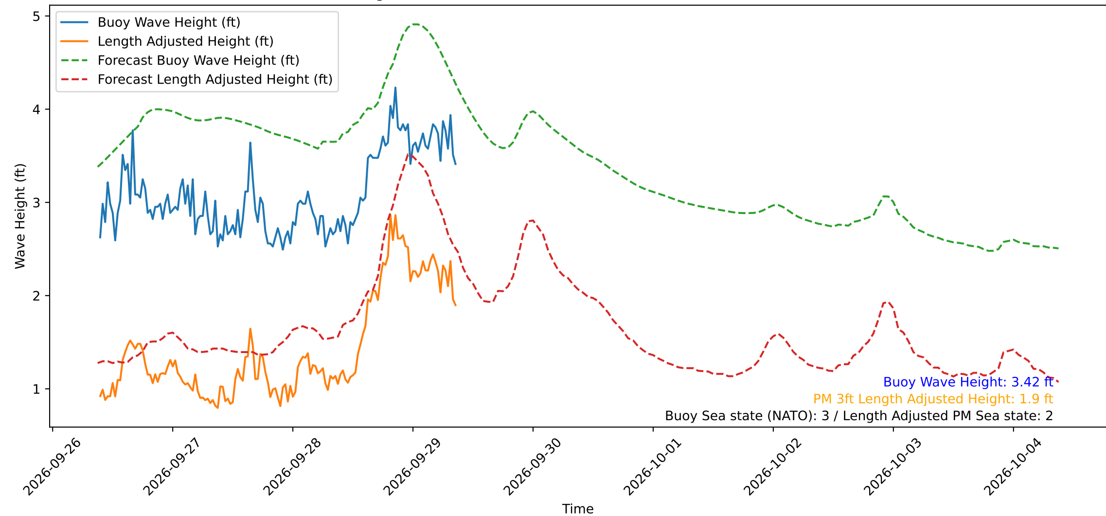
Wave Heights over Time for Oceanside Harbor at 2026-09-29 09:20:29
