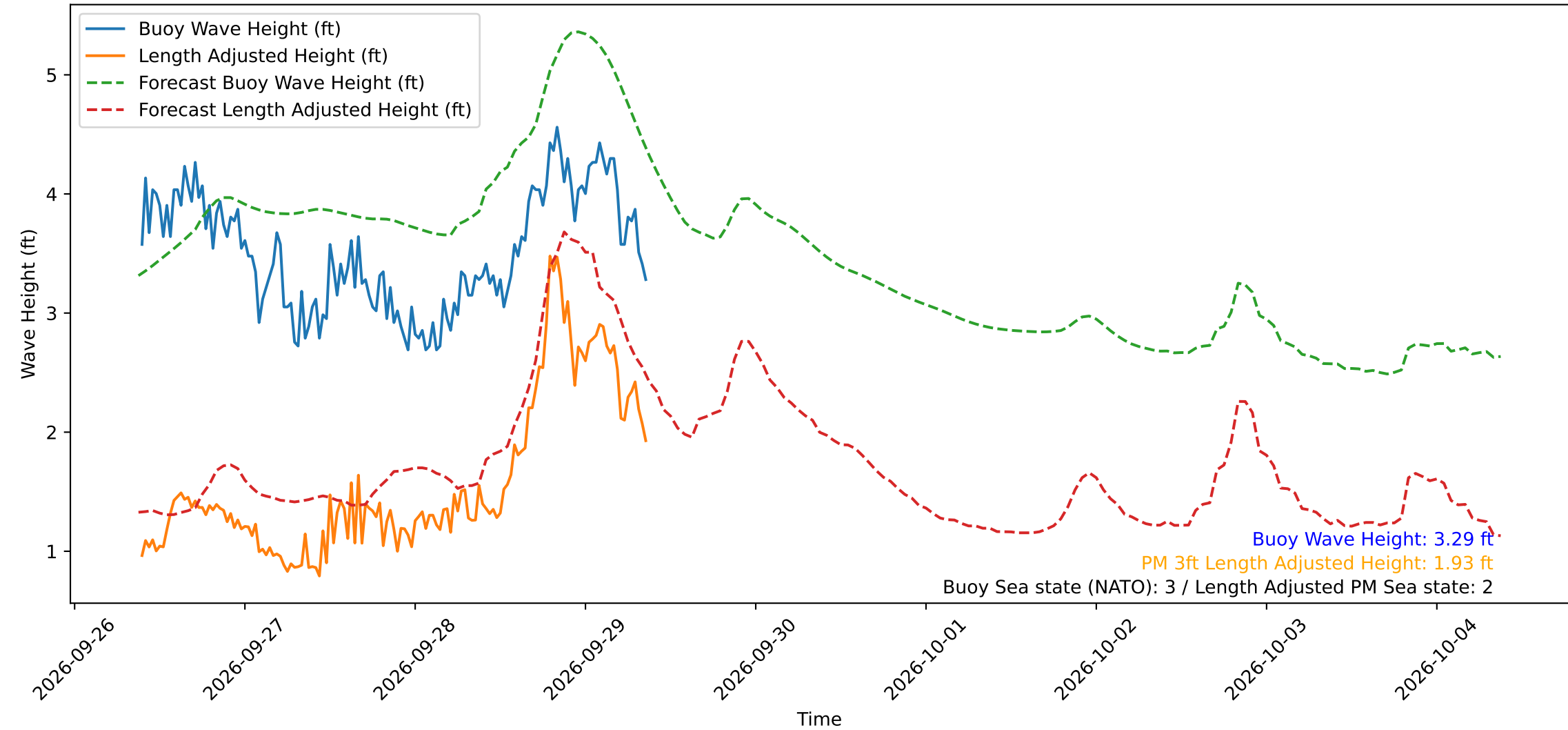
Wave Heights over Time for Green Beach at 2026-09-29 09:21:17
