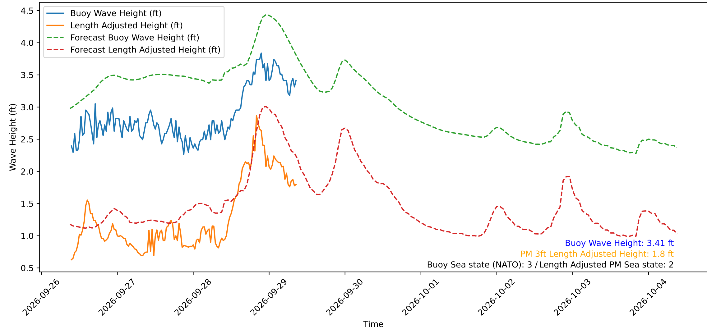
Wave Heights over Time for Red Beach at 2026-09-29 09:20:50
