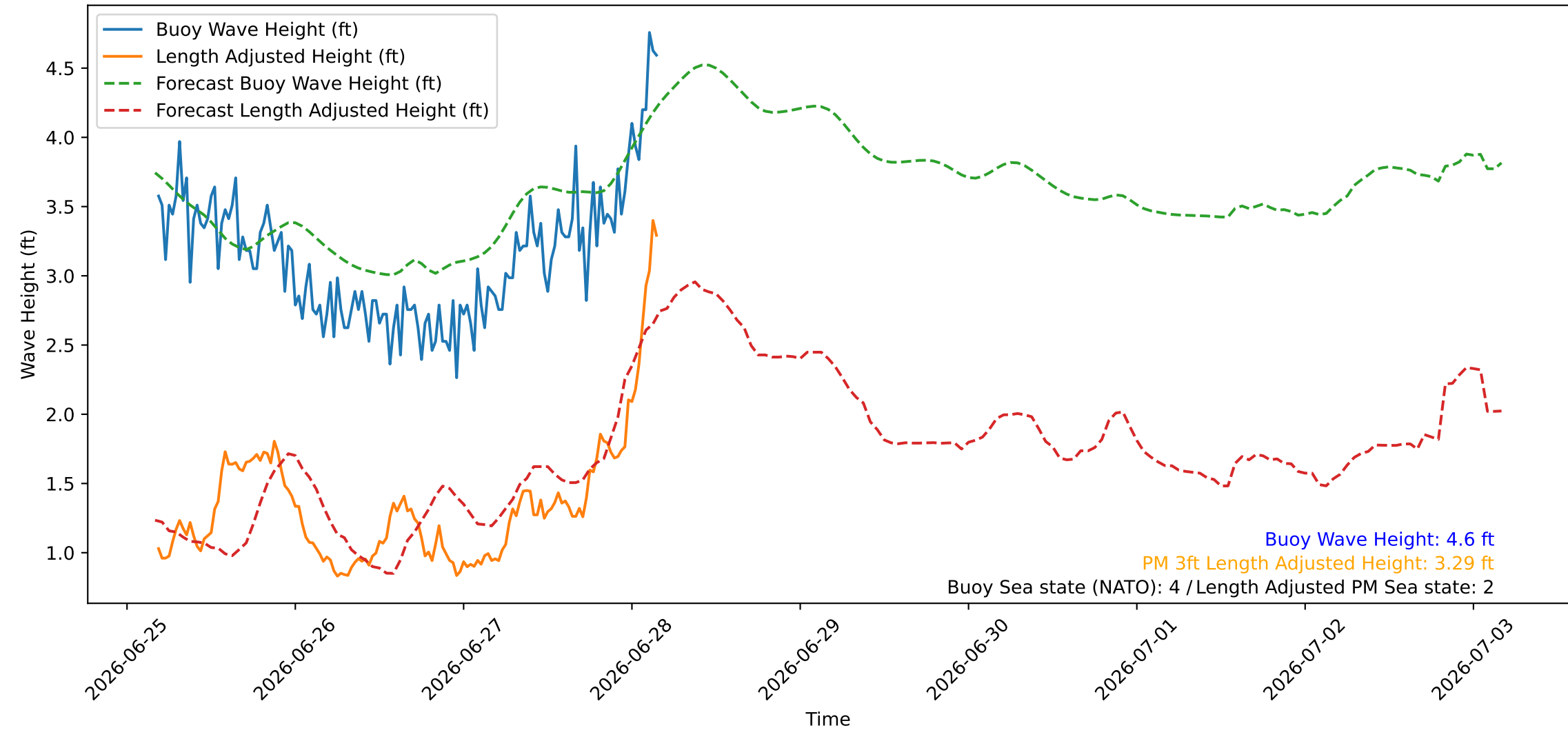
Wave Heights over Time for Green Beach at 2026-06-28 04:21:09
