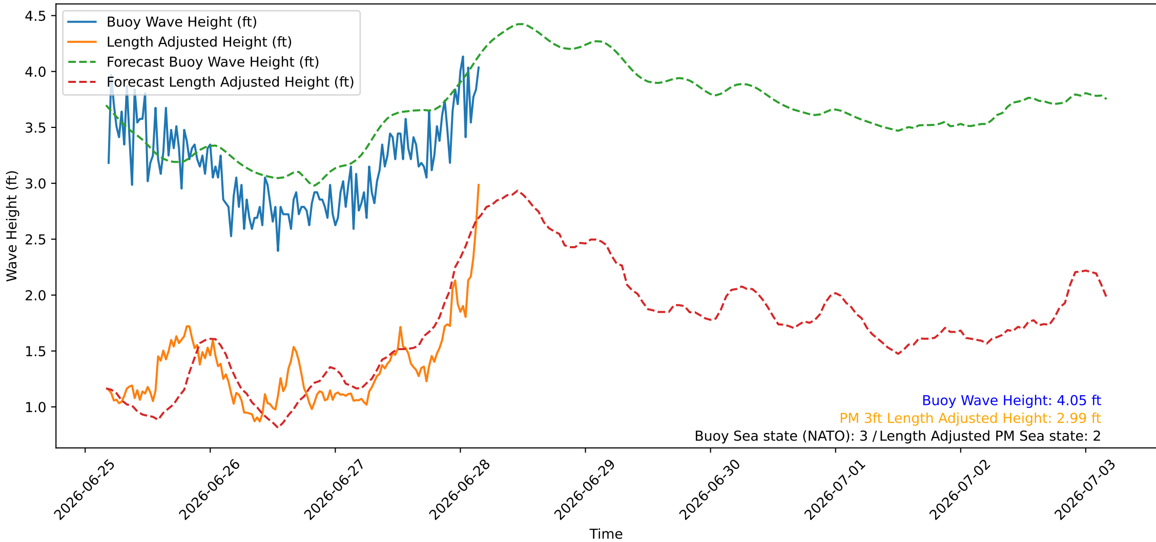
Wave Heights over Time for Oceanside Harbor at 2026-06-28 04:20:26
