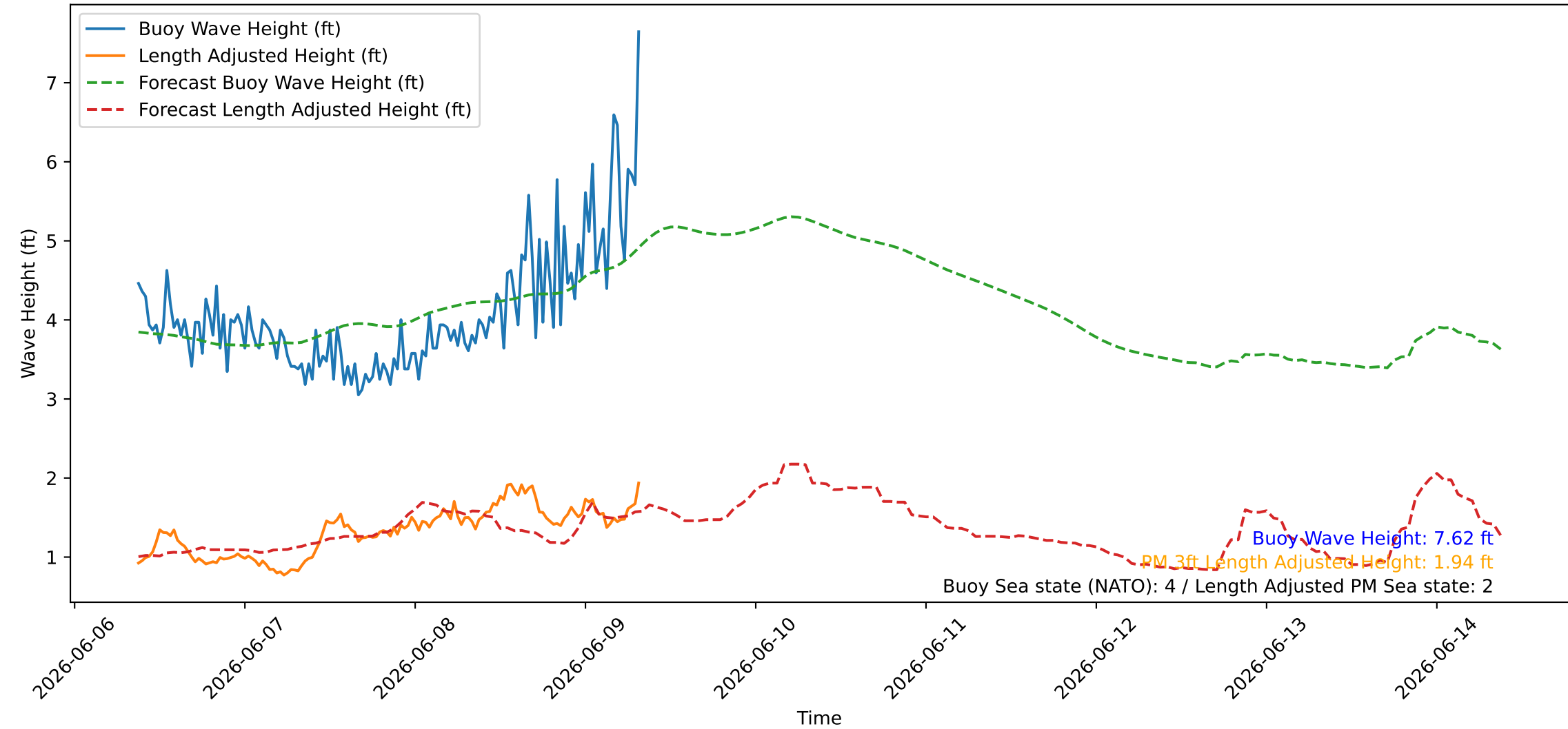
Wave Heights over Time for Red Beach at 2026-06-09 08:30:45
