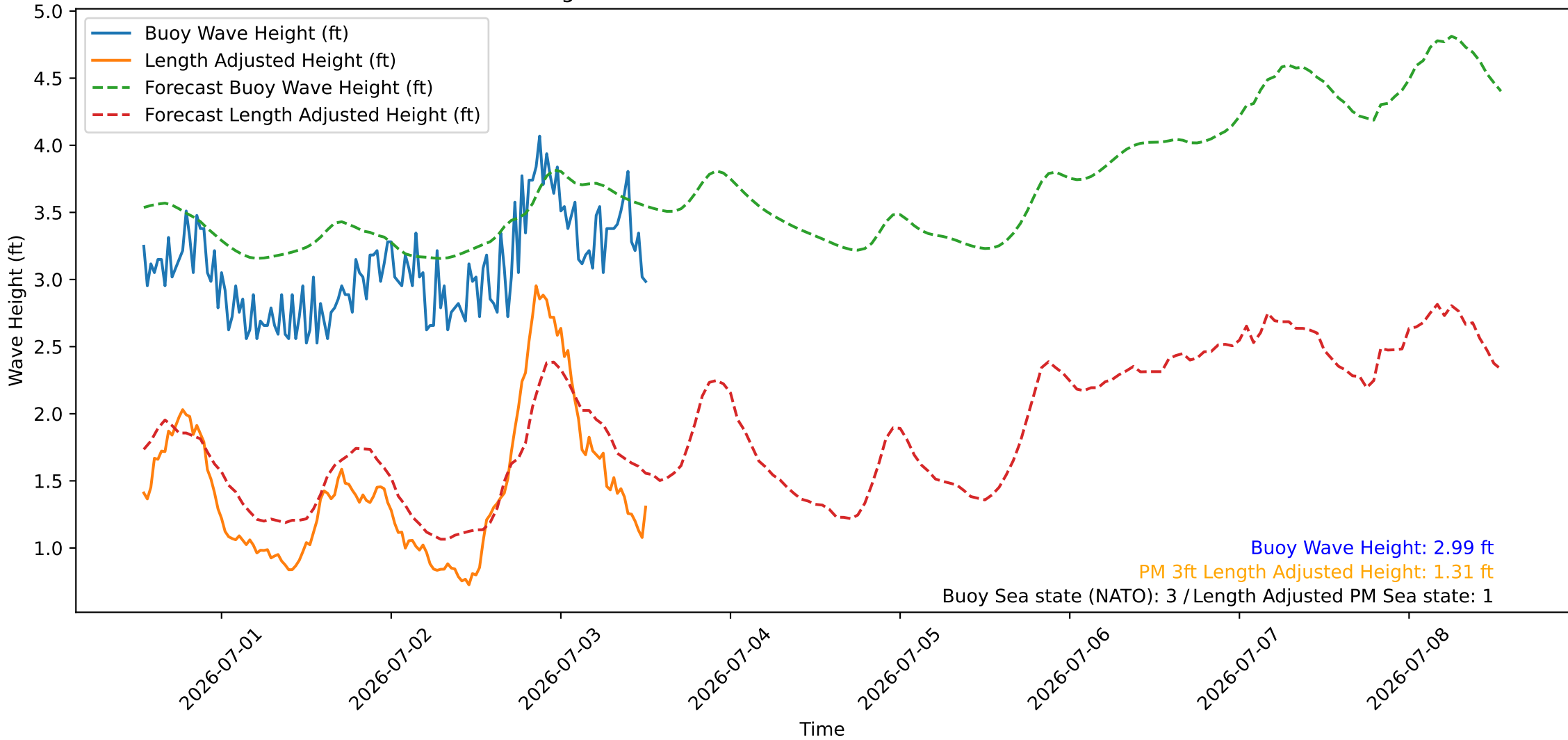
Wave Heights over Time for Green Beach at 2026-07-03 12:51:09
