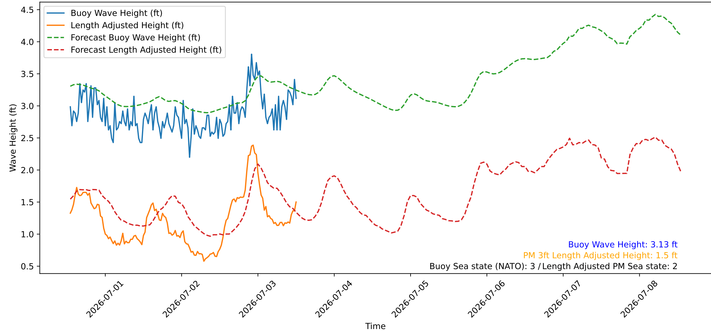
Wave Heights over Time for Red Beach at 2026-07-03 12:50:47
