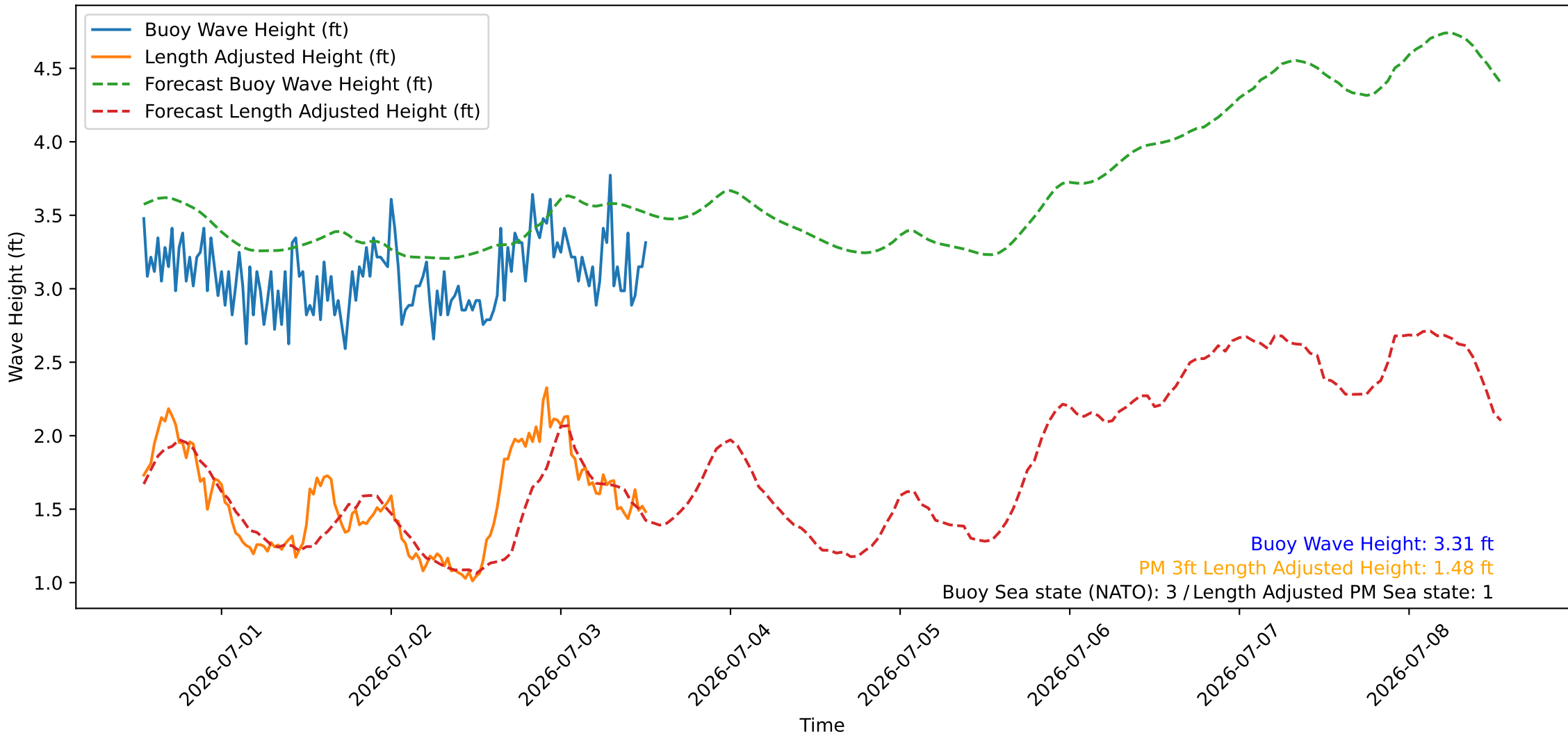
Wave Heights over Time for Oceanside Harbor at 2026-07-03 12:50:26
