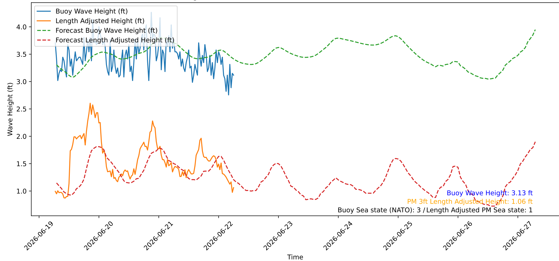
Wave Heights over Time for Oceanside Harbor at 2026-06-22 06:40:26
