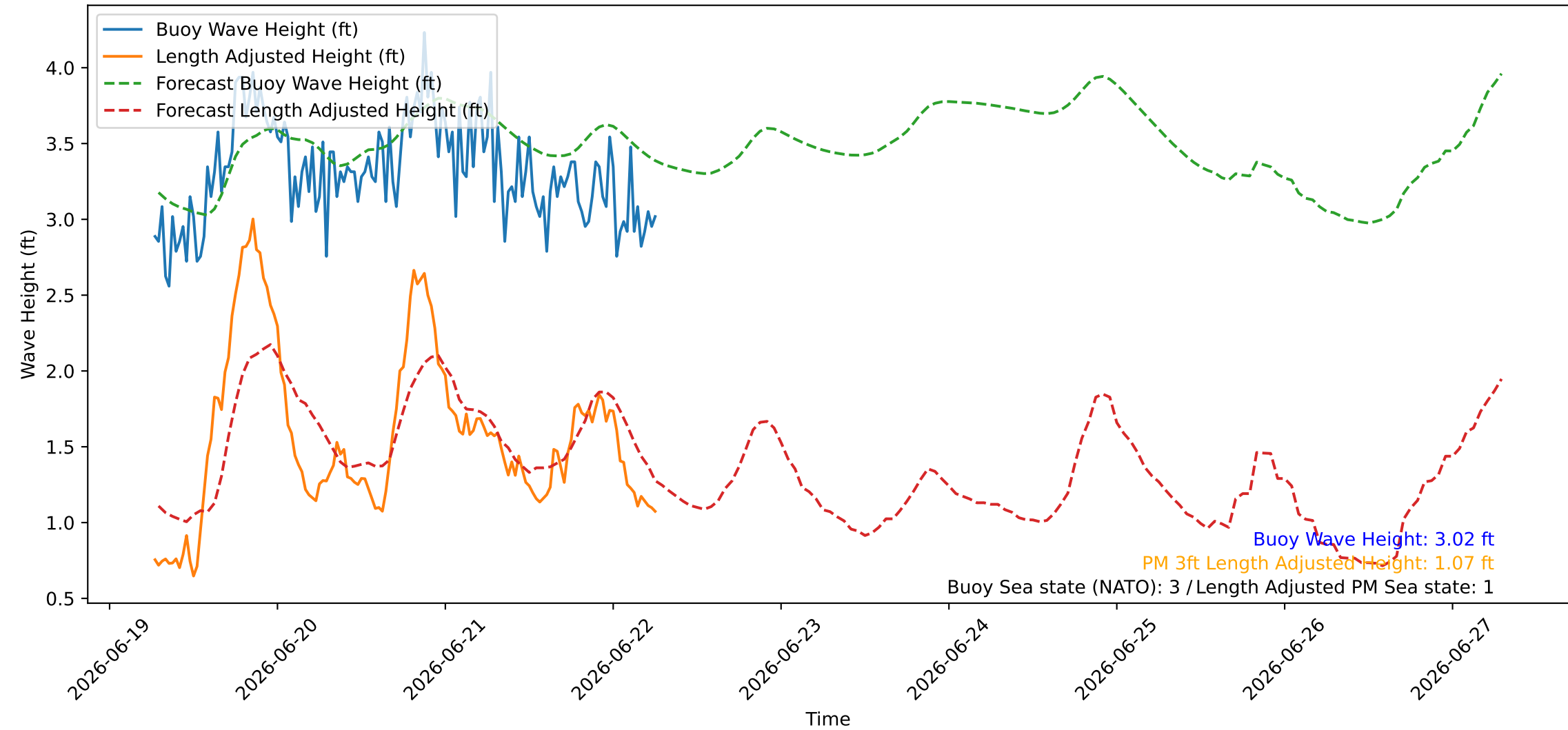
Wave Heights over Time for Green Beach at 2026-06-22 06:41:08
