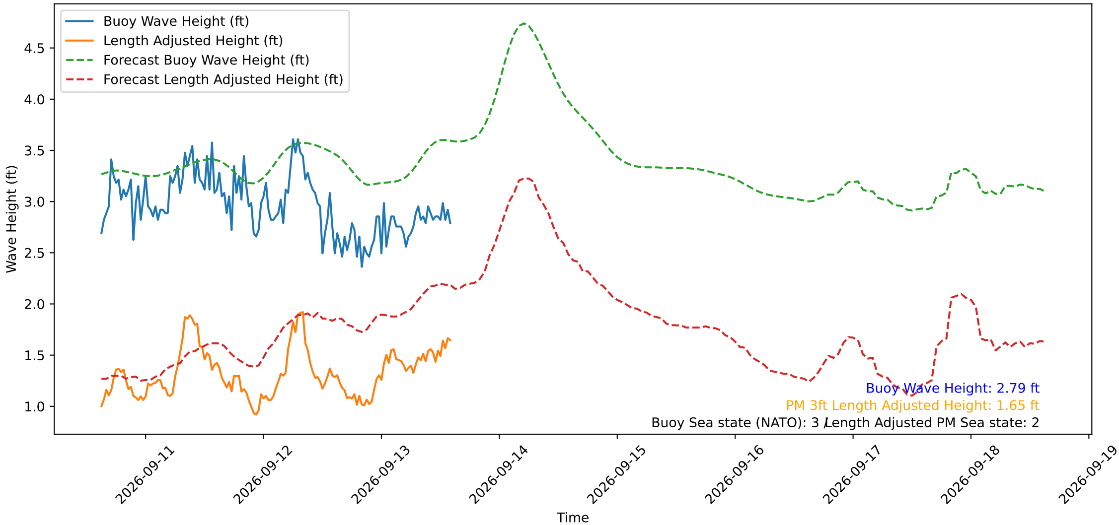
Wave Heights over Time for Green Beach at 2026-09-13 14:41:11
