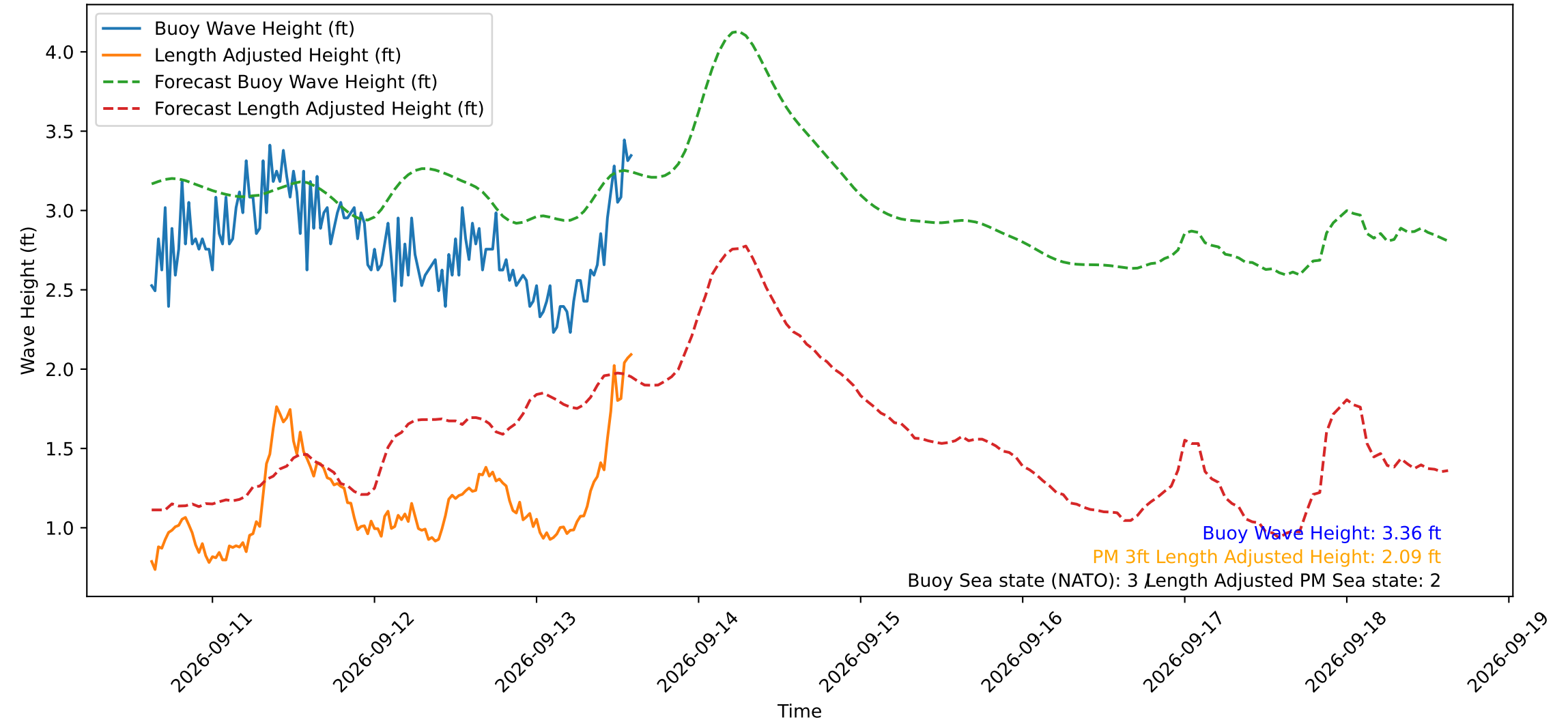
Wave Heights over Time for Red Beach at 2026-09-13 14:40:48
