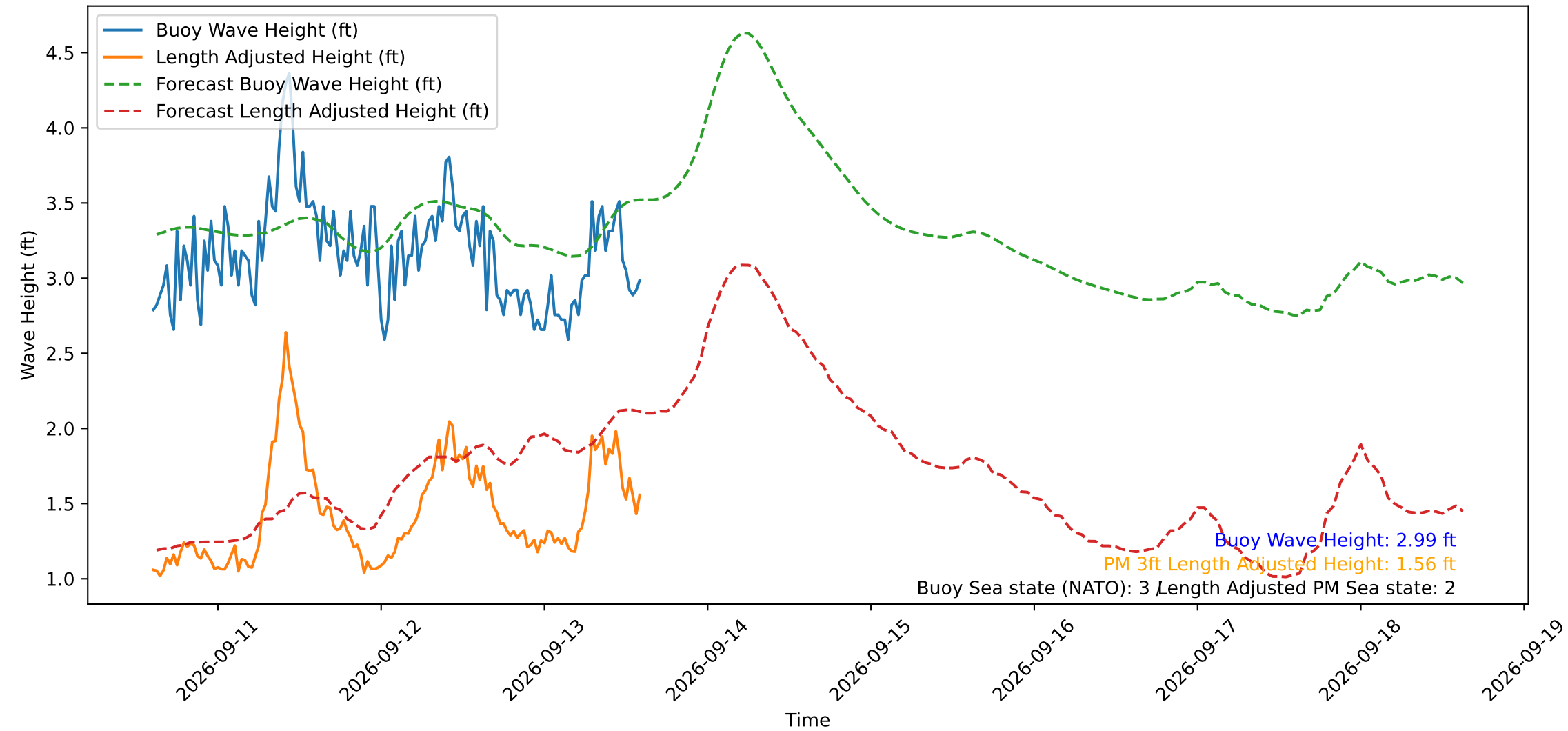
Wave Heights over Time for Oceanside Harbor at 2026-09-13 14:40:29
