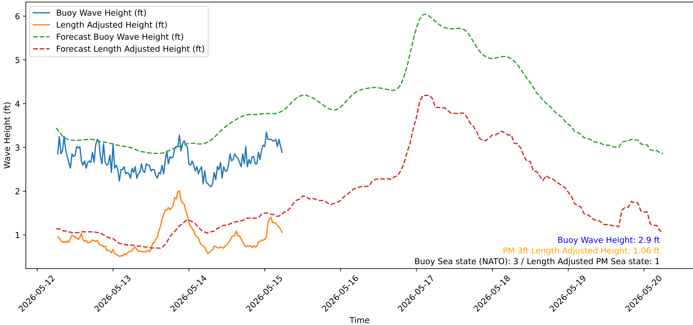
Wave Heights over Time for Green Beach at 2026-05-15 06:21:15
