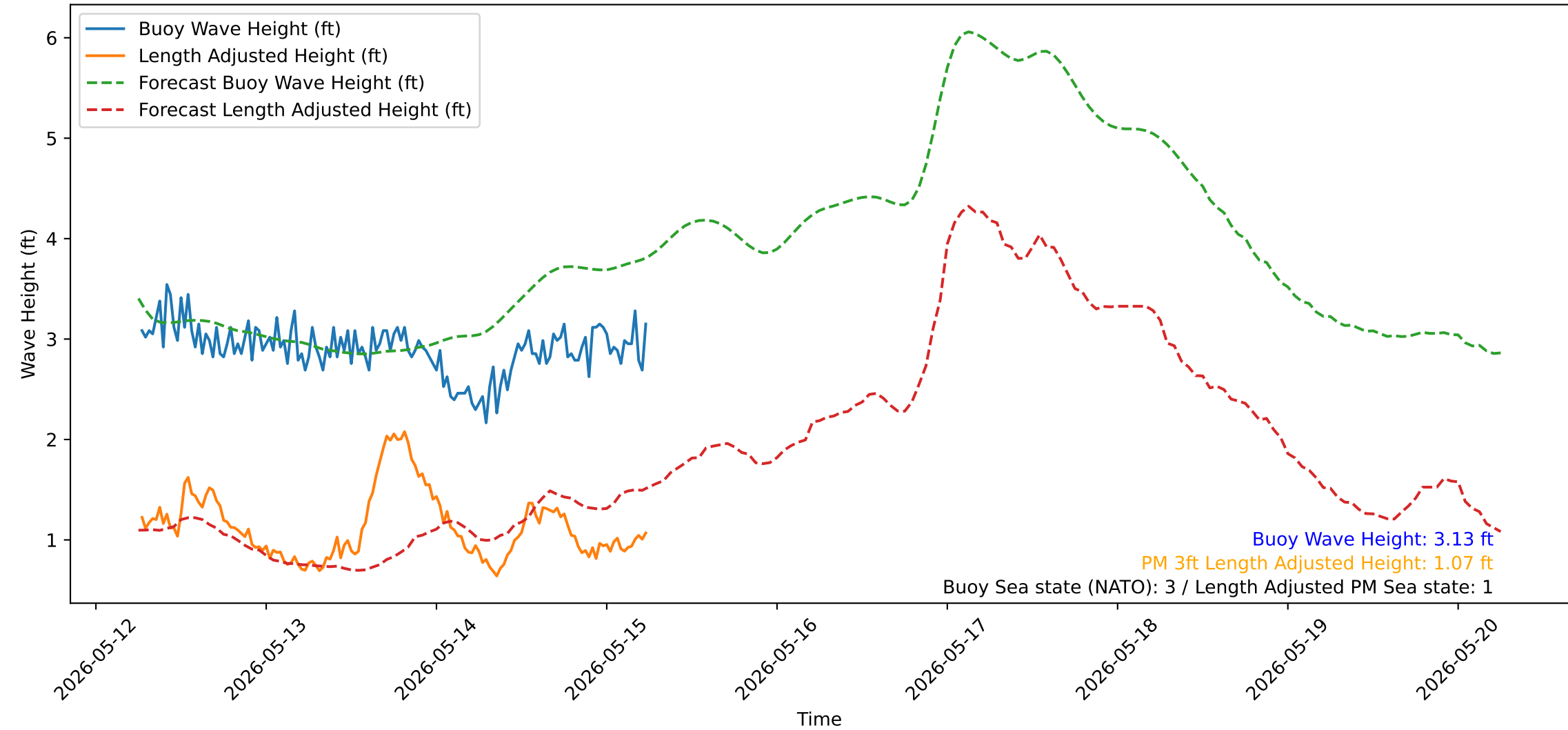
Wave Heights over Time for Oceanside Harbor at 2026-05-15 06:20:31
