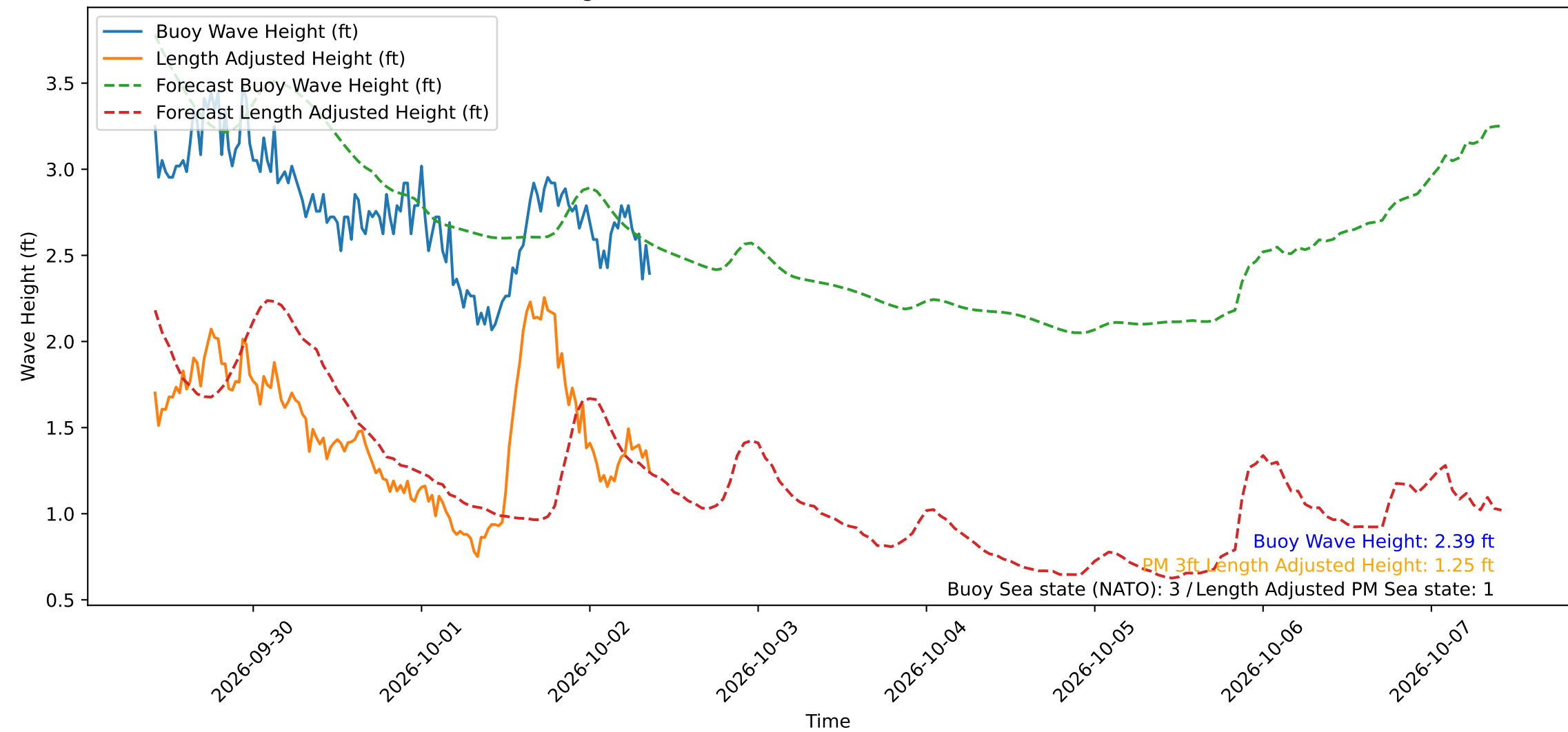
Wave Heights over Time for Red Beach at 2026-10-02 09:30:49
