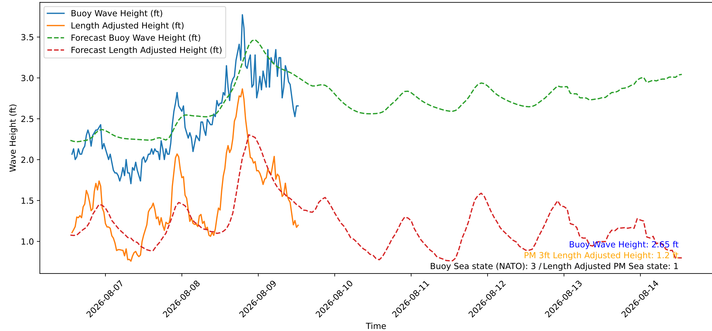
Wave Heights over Time for Green Beach at 2026-08-09 13:21:10
