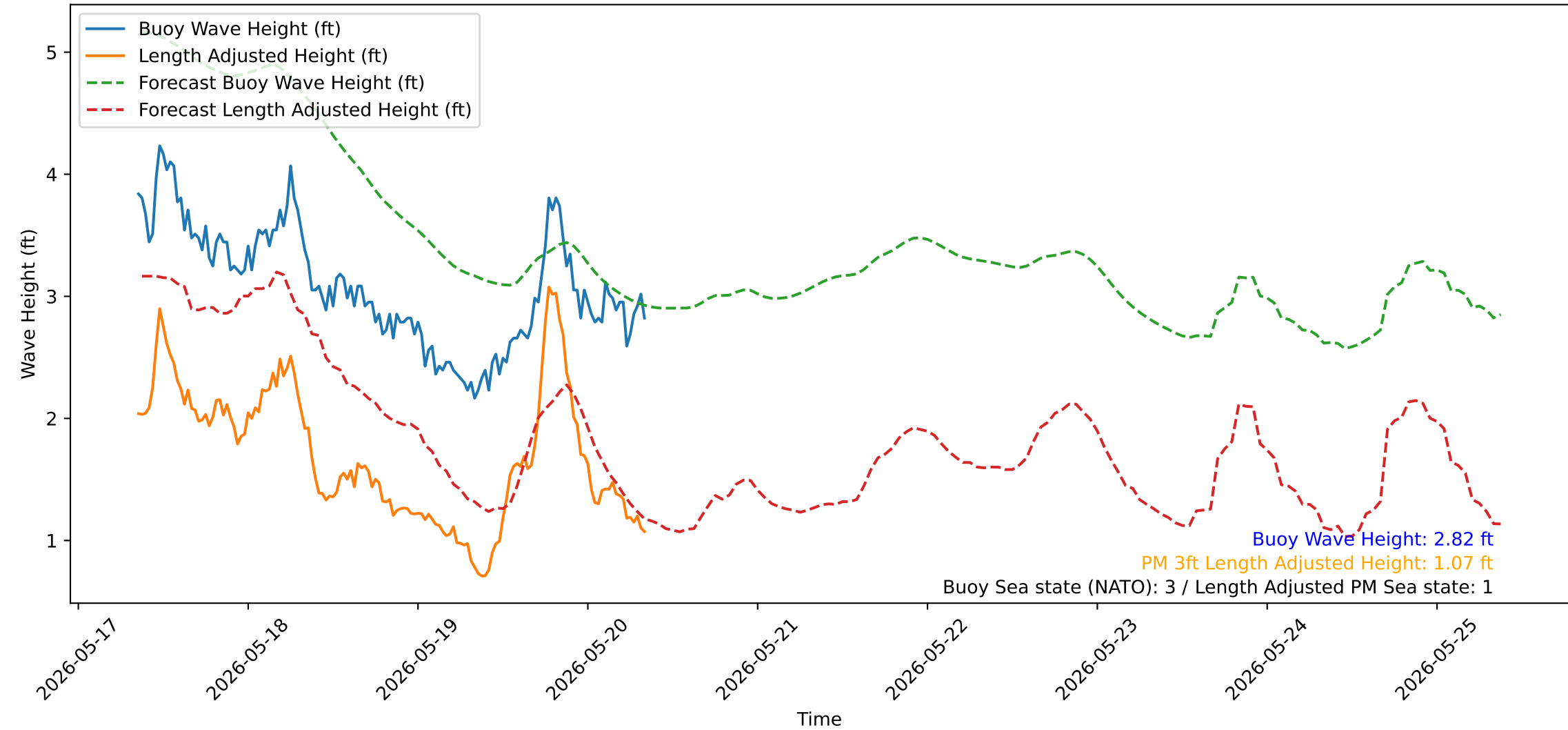
Wave Heights over Time for Green Beach at 2026-05-20 08:41:14
