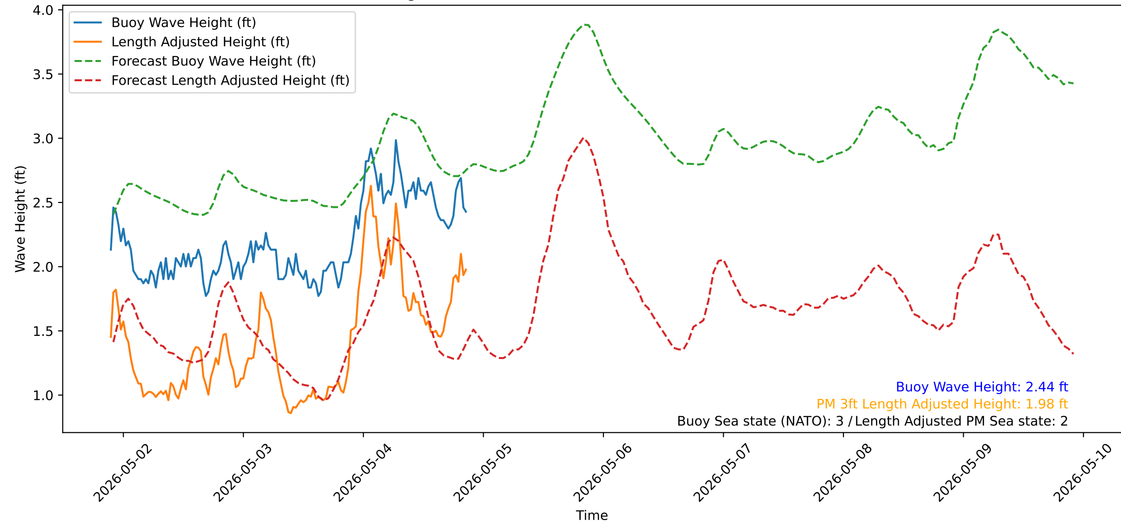
Wave Heights over Time for Green Beach at 2026-05-04 21:31:12
