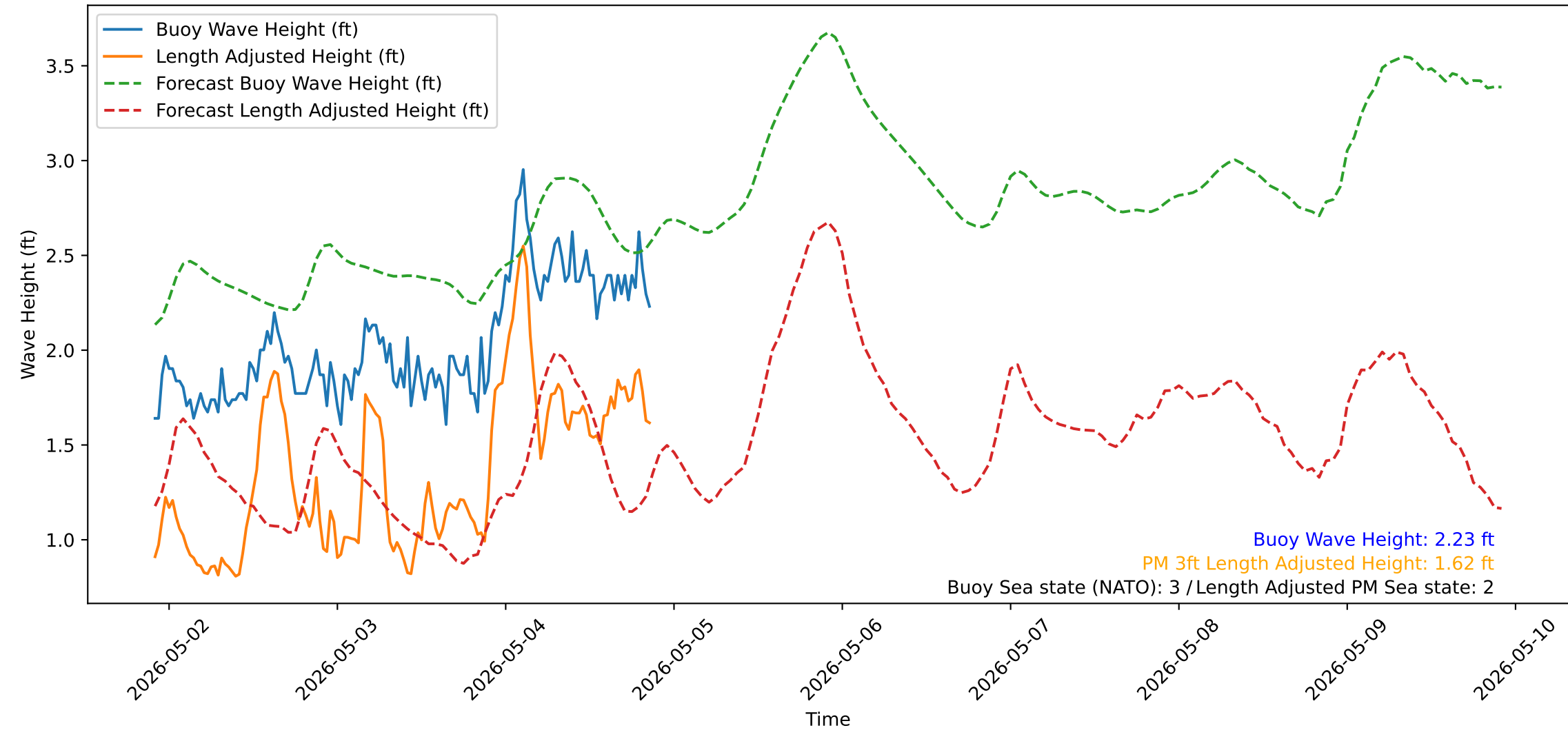
Wave Heights over Time for Red Beach at 2026-05-04 21:30:50
