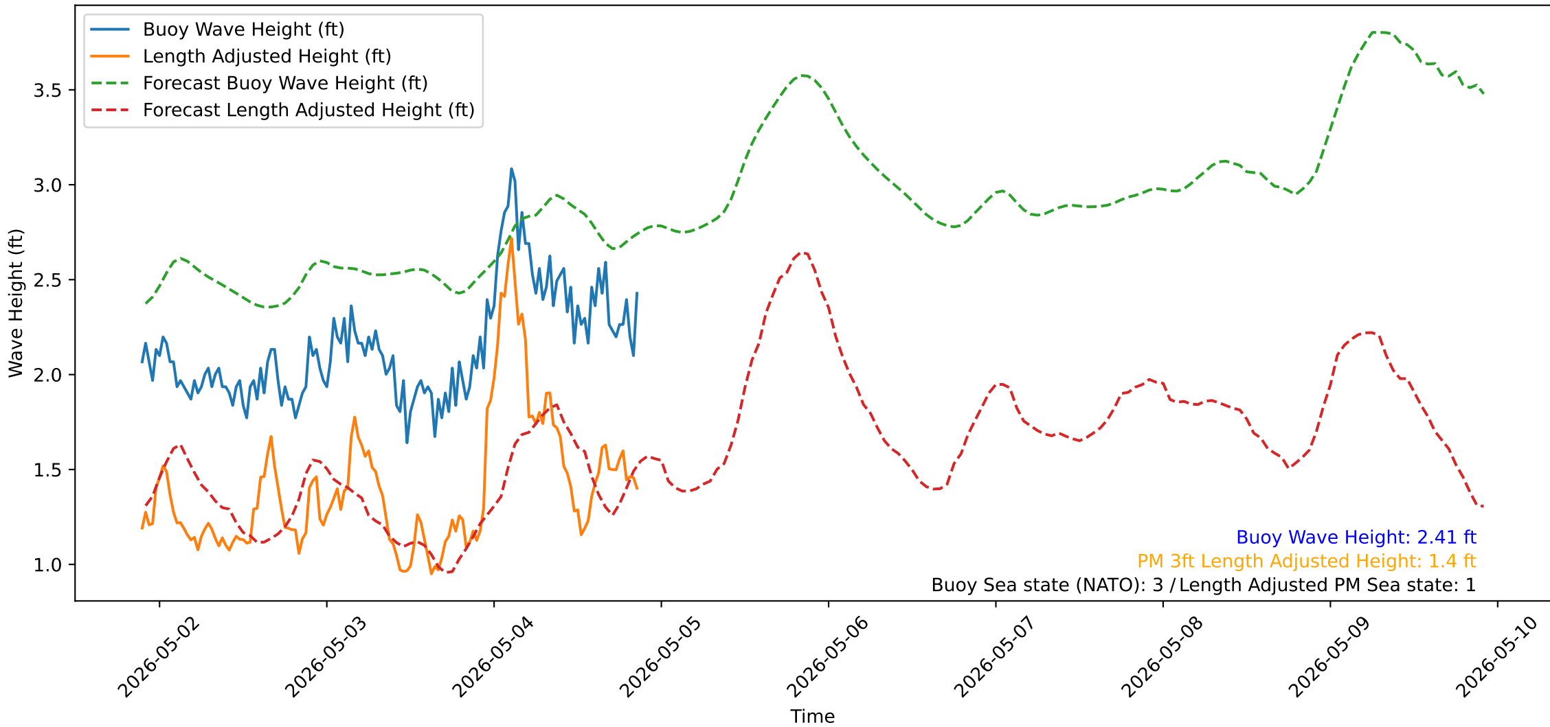
Wave Heights over Time for Oceanside Harbor at 2026-05-04 21:30:31
