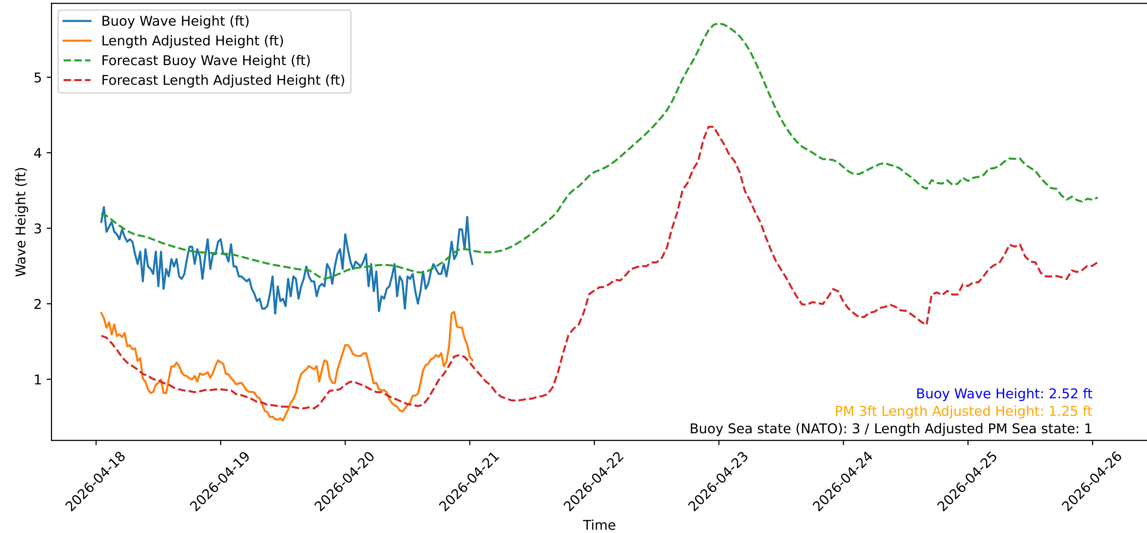
Wave Heights over Time for Green Beach at 2026-04-21 01:11:12
