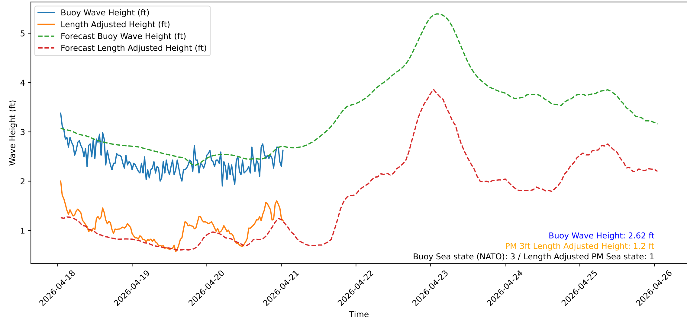
Wave Heights over Time for Oceanside Harbor at 2026-04-21 01:10:31
