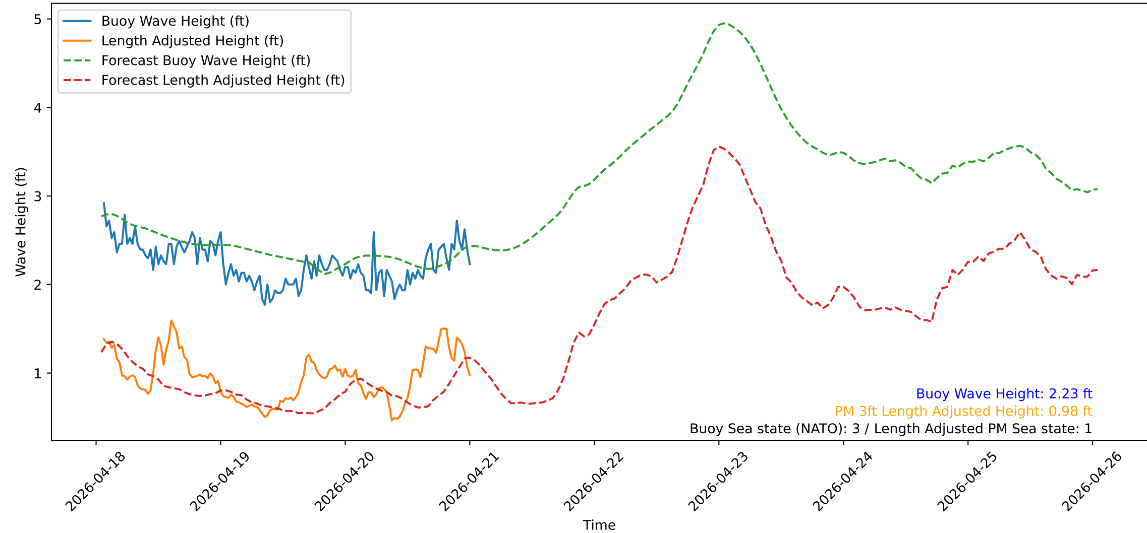
Wave Heights over Time for Red Beach at 2026-04-21 01:10:50
