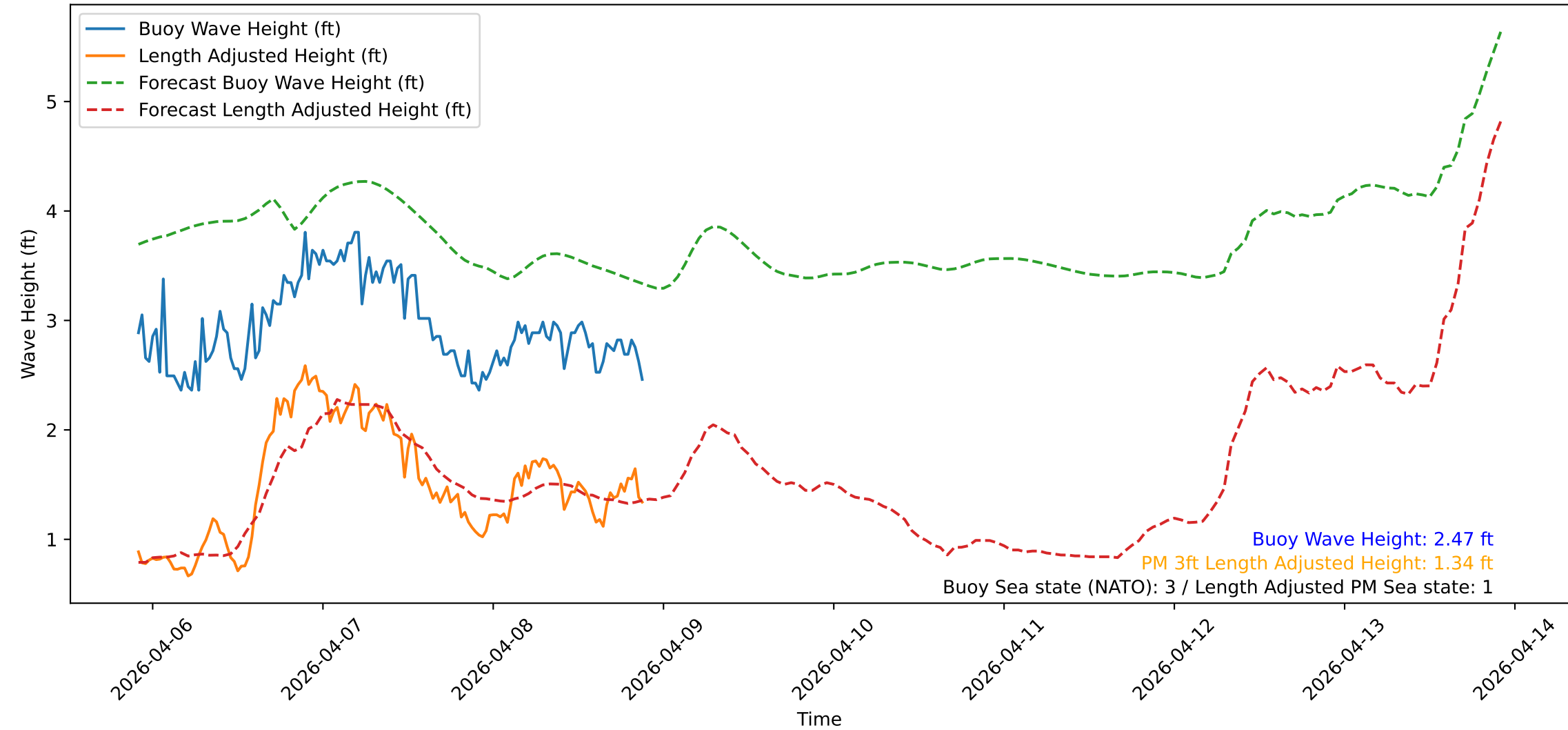
Wave Heights over Time for Green Beach at 2026-04-08 22:01:10
