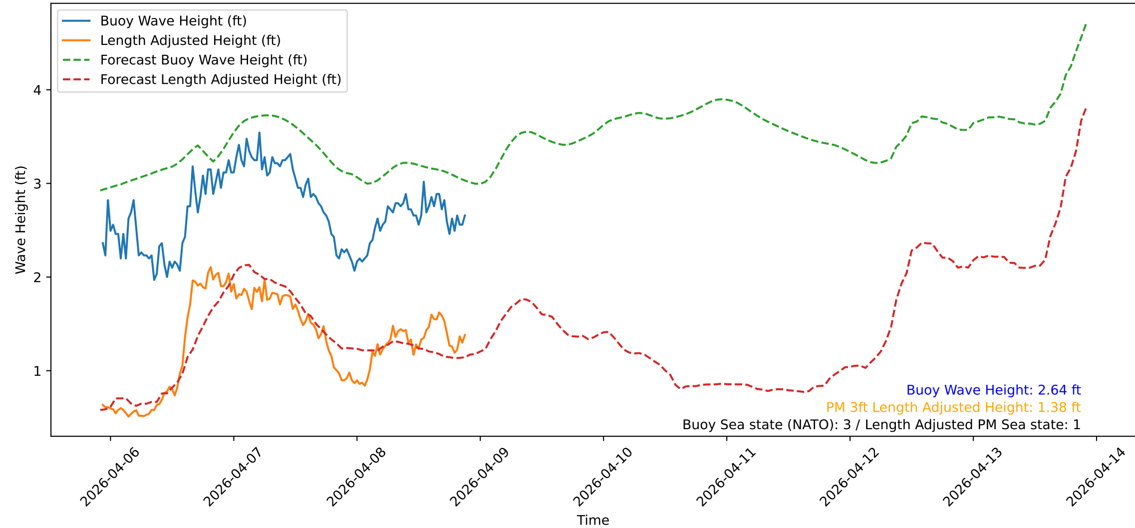
Wave Heights over Time for Red Beach at 2026-04-08 22:00:48
