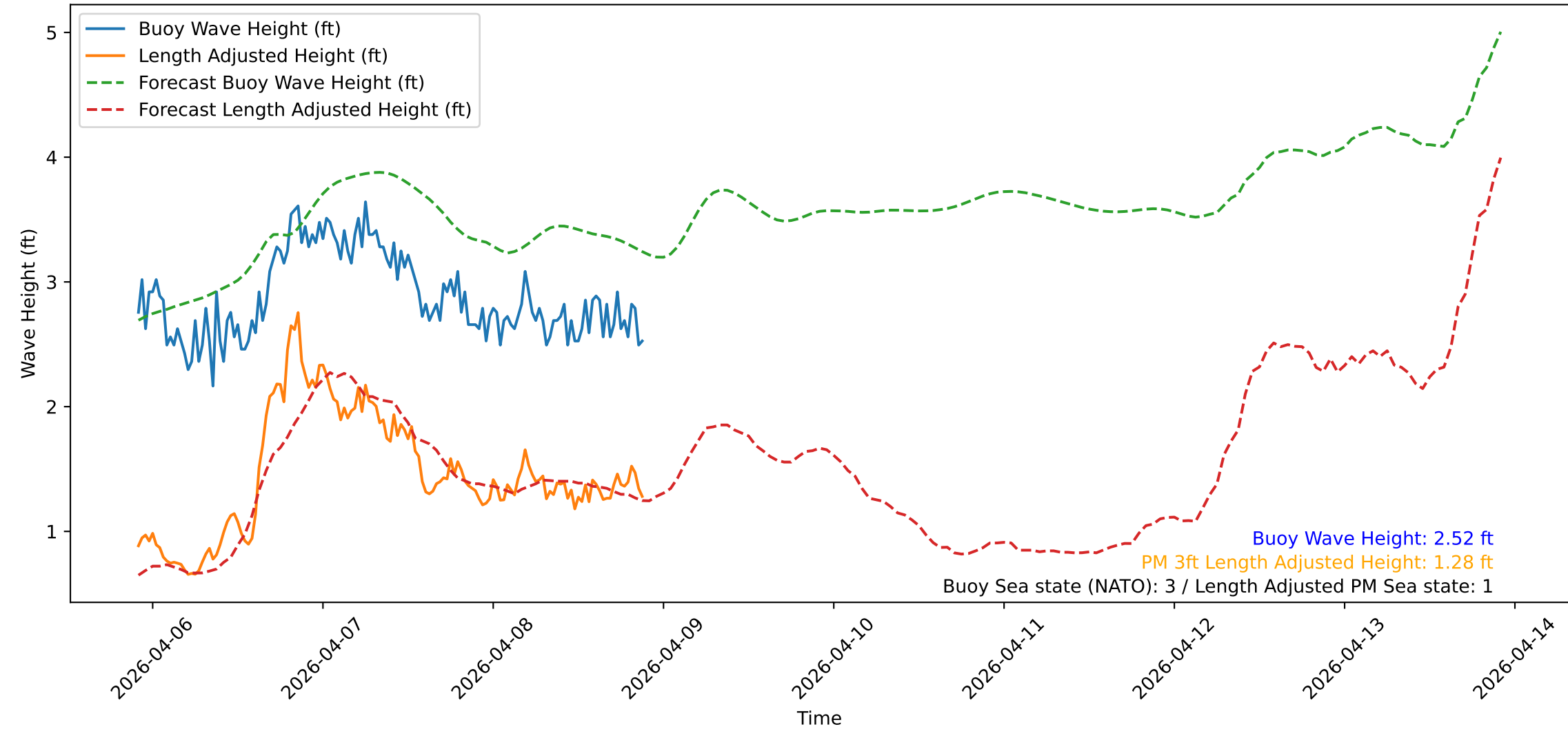
Wave Heights over Time for Oceanside Harbor at 2026-04-08 22:00:32
