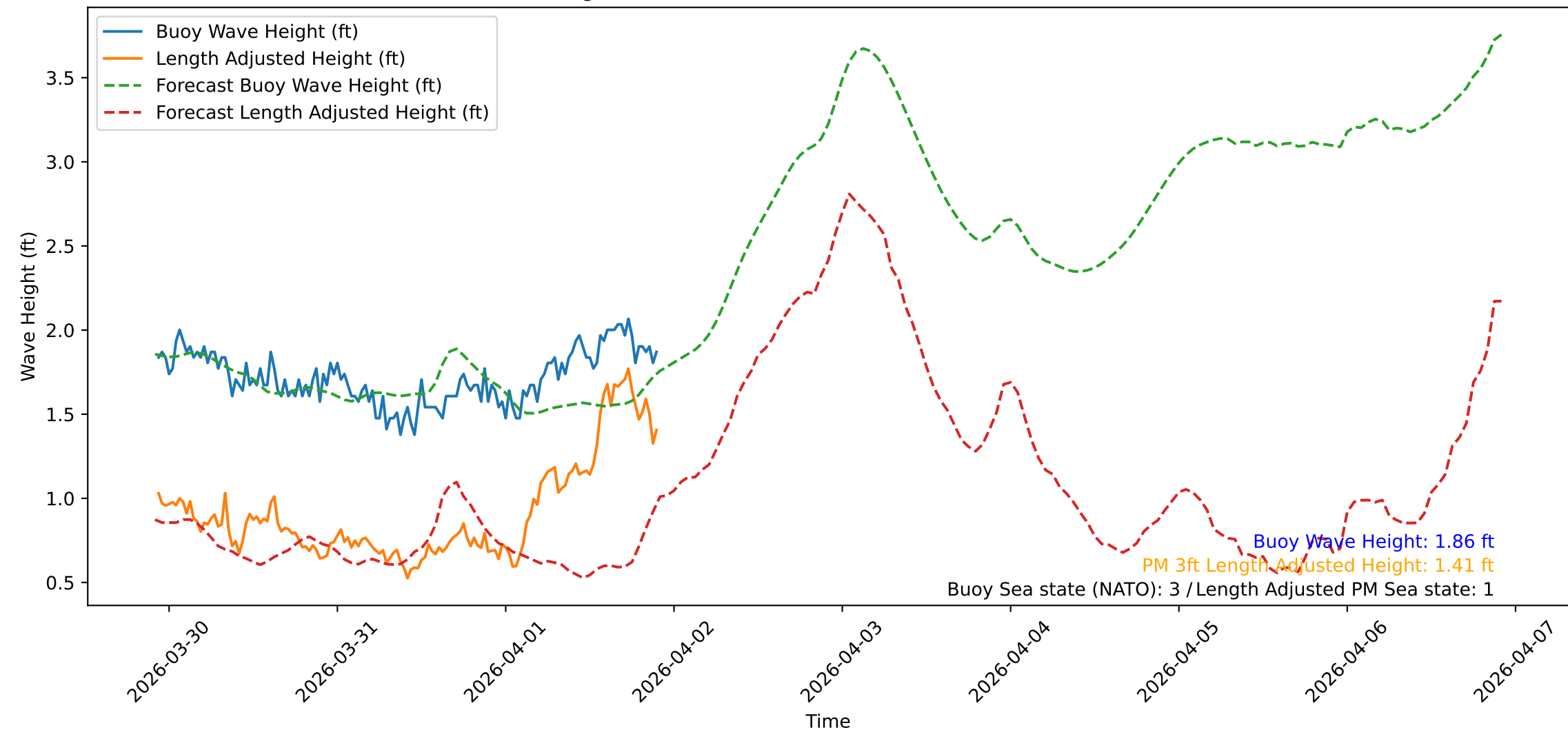
Wave Heights over Time for Red Beach at 2026-04-01 22:10:46
