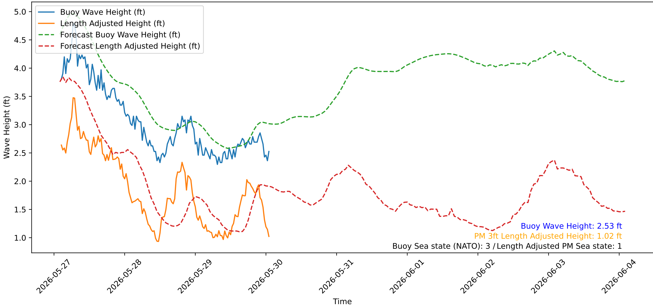
Wave Heights over Time for Red Beach at 2026-05-30 02:00:42
