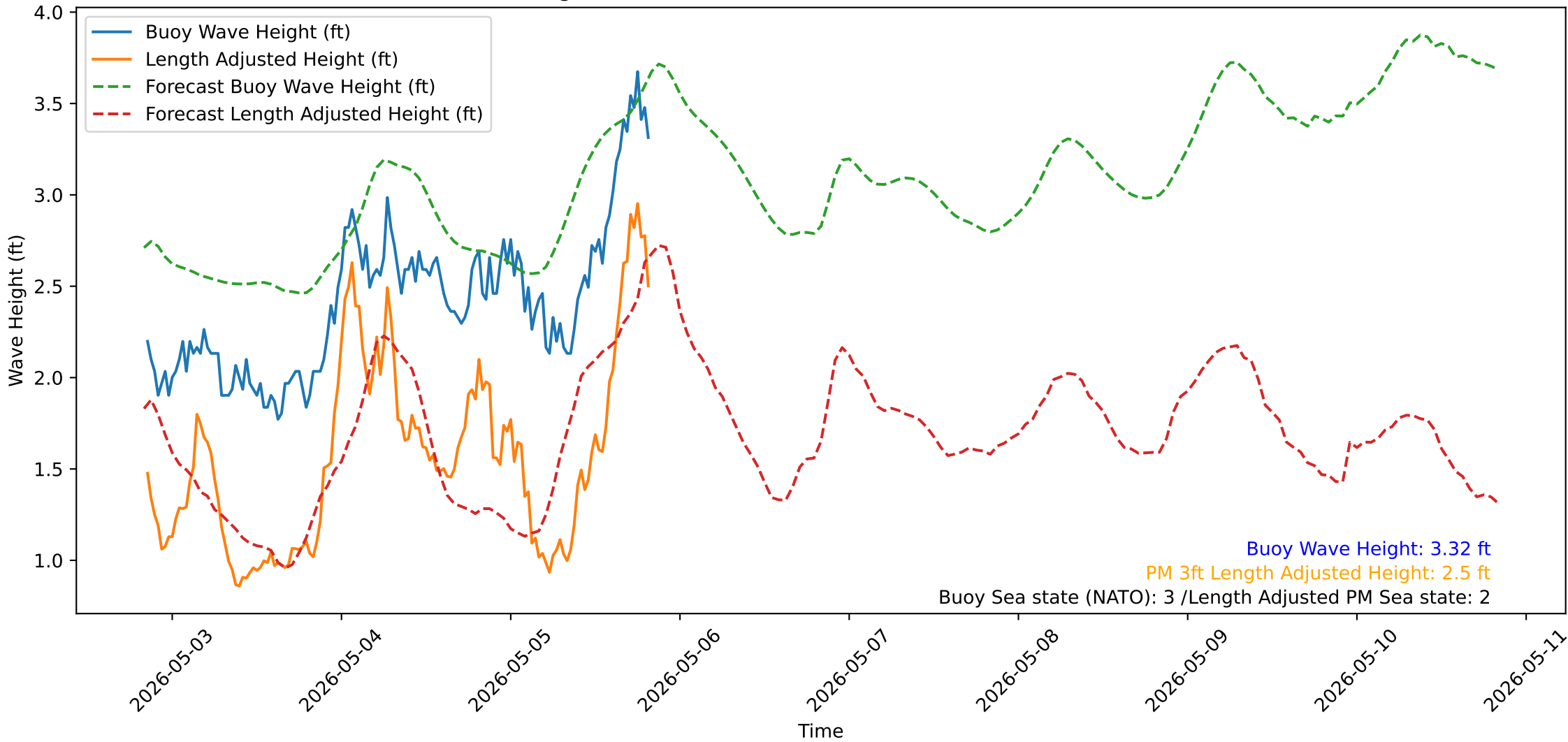
Wave Heights over Time for Green Beach at 2026-05-05 20:21:14
