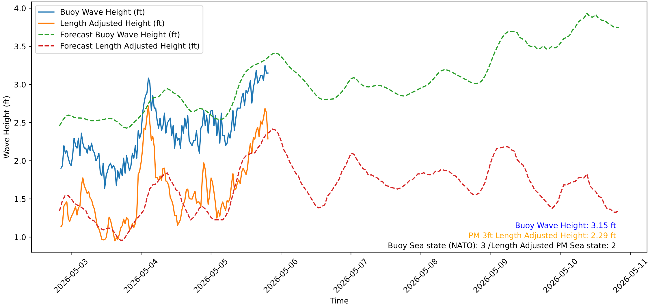
Wave Heights over Time for Oceanside Harbor at 2026-05-05 20:20:32
