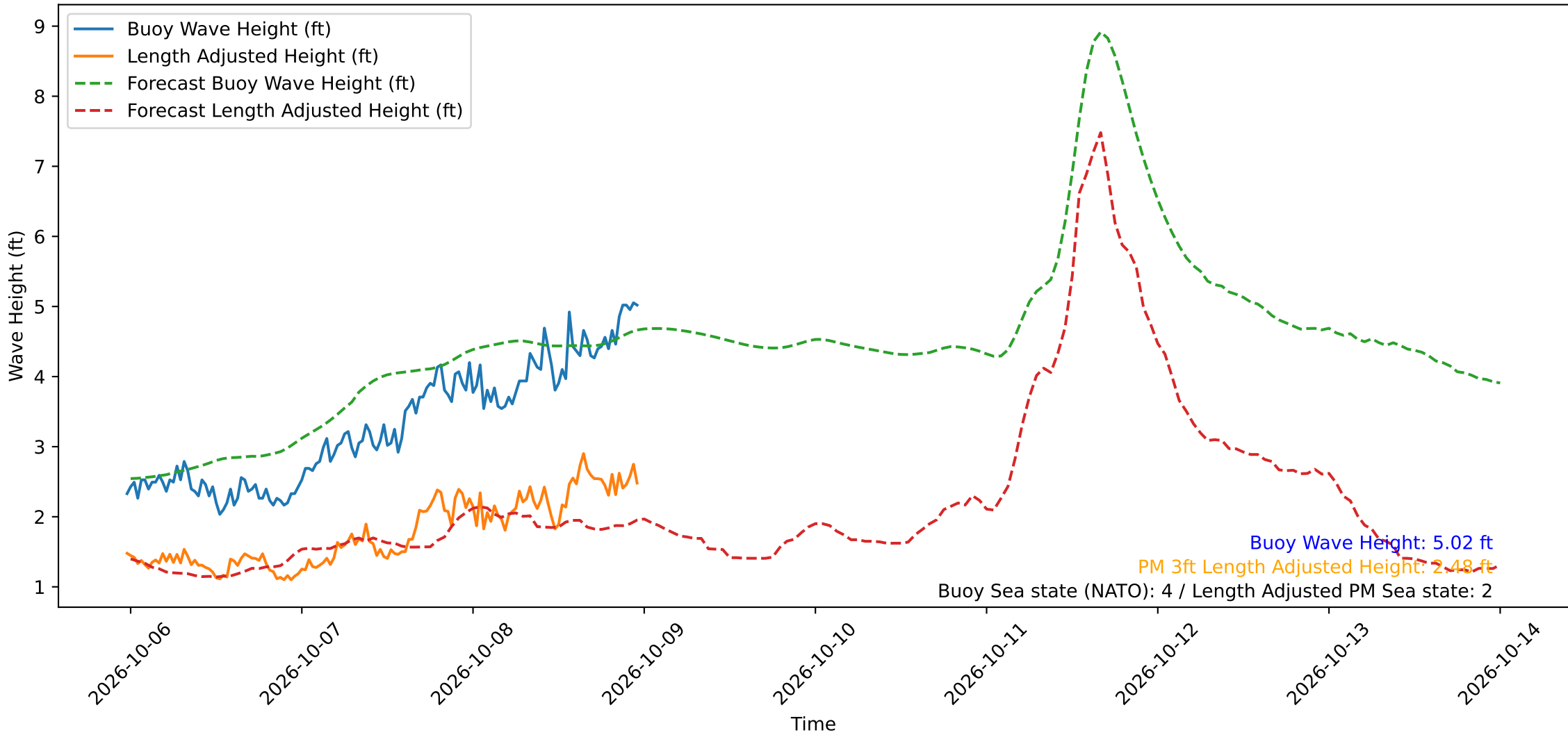
Wave Heights over Time for Oceanside Harbor at 2026-10-08 23:40:30
