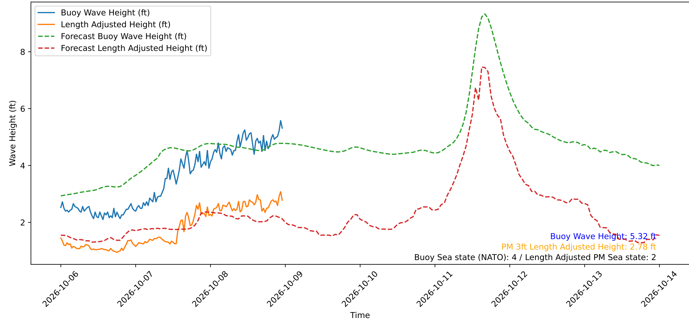
Wave Heights over Time for Green Beach at 2026-10-08 23:41:11
