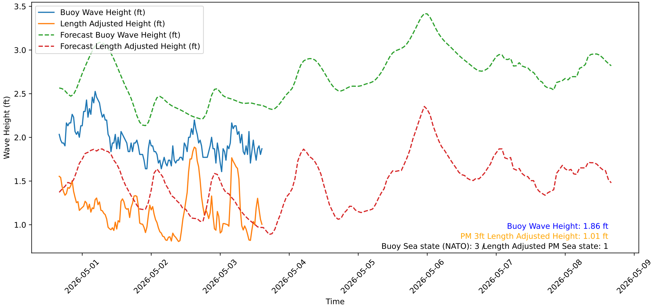
Wave Heights over Time for Red Beach at 2026-05-03 15:30:50
