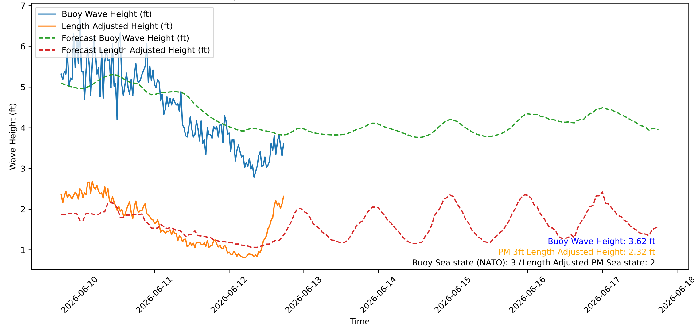
Wave Heights over Time for Oceanside Harbor at 2026-06-12 18:10:26
