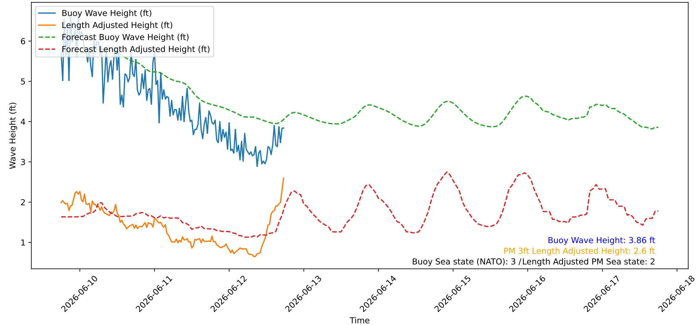
Wave Heights over Time for Green Beach at 2026-06-12 18:11:08
