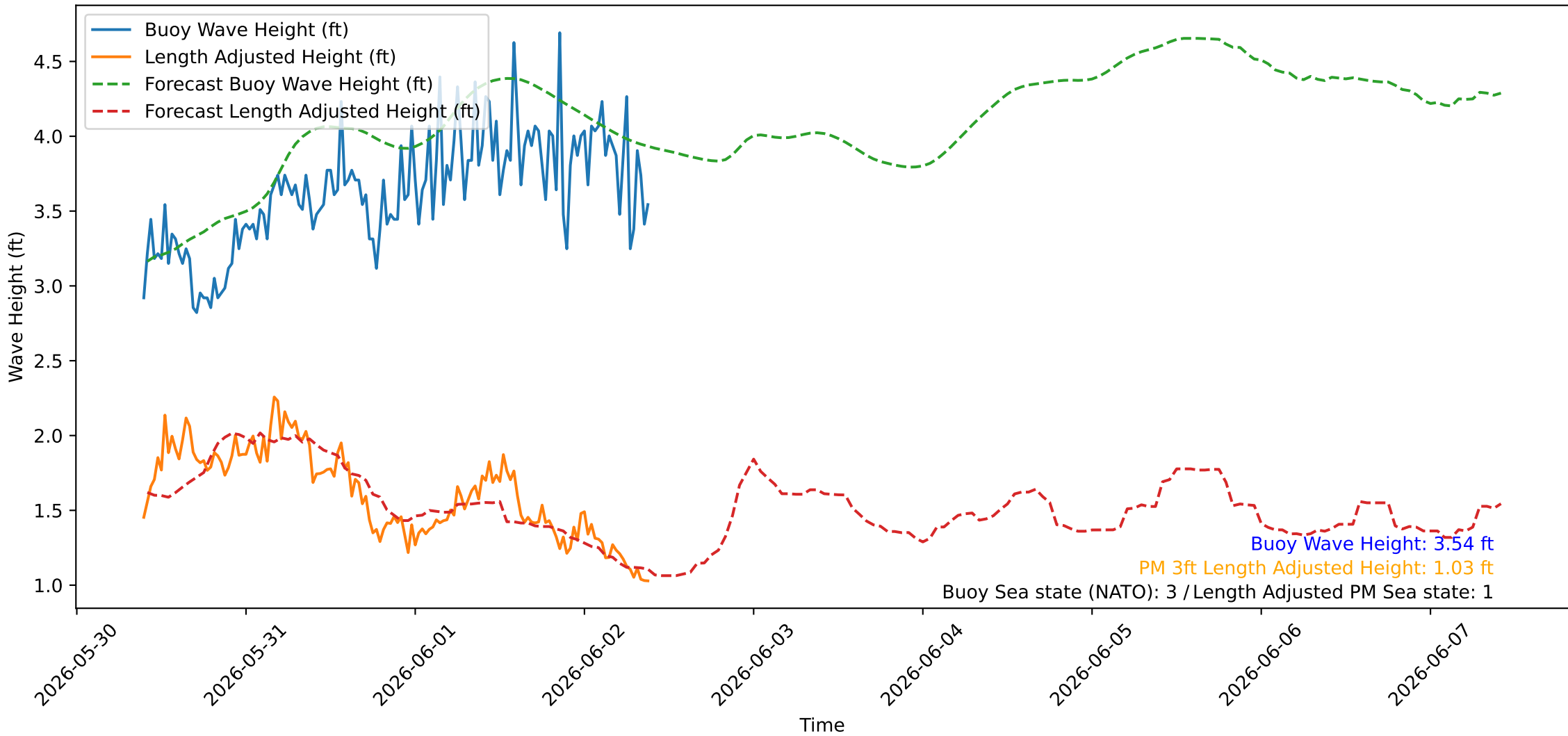
Wave Heights over Time for Oceanside Harbor at 2026-06-02 09:40:26
