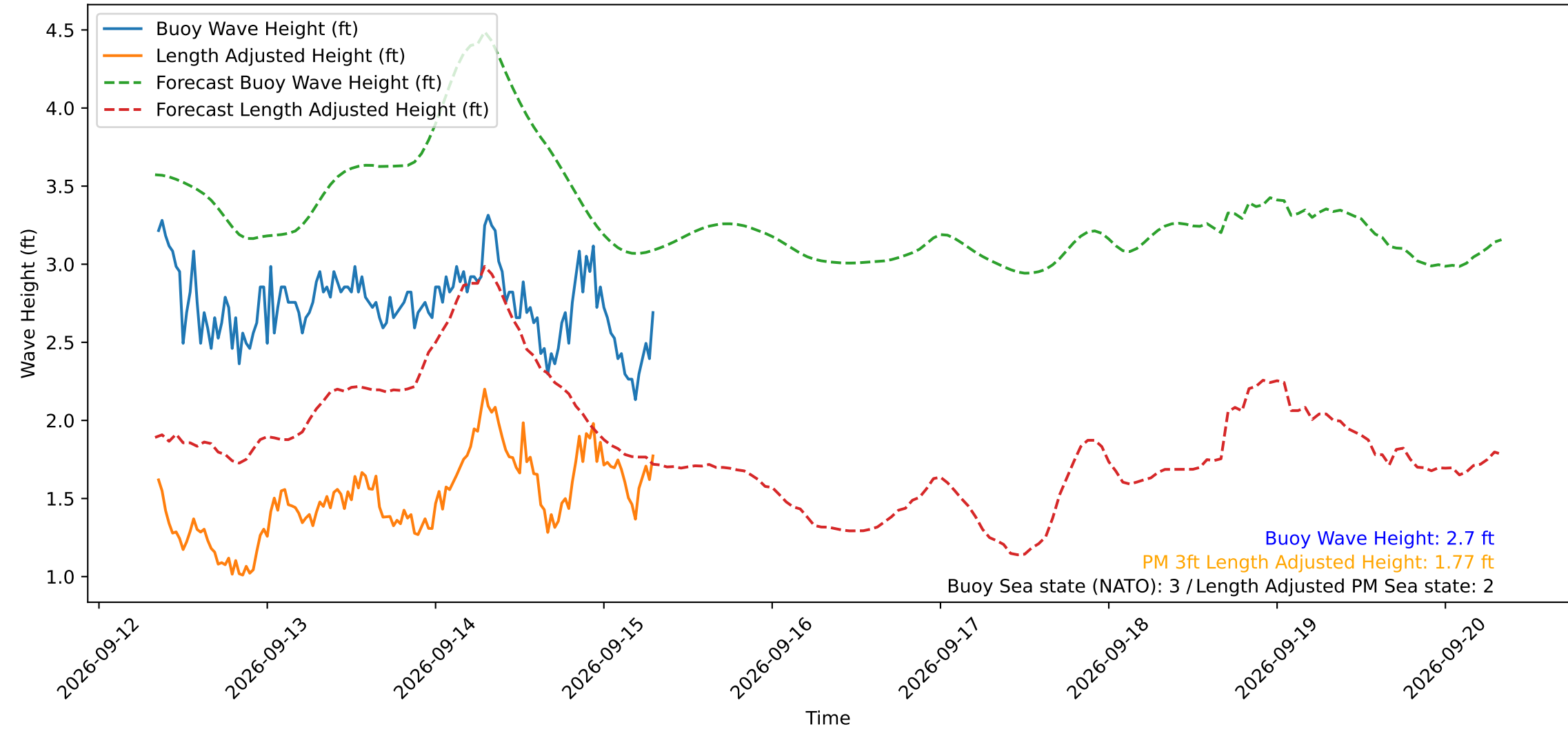
Wave Heights over Time for Green Beach at 2026-09-15 08:11:11
