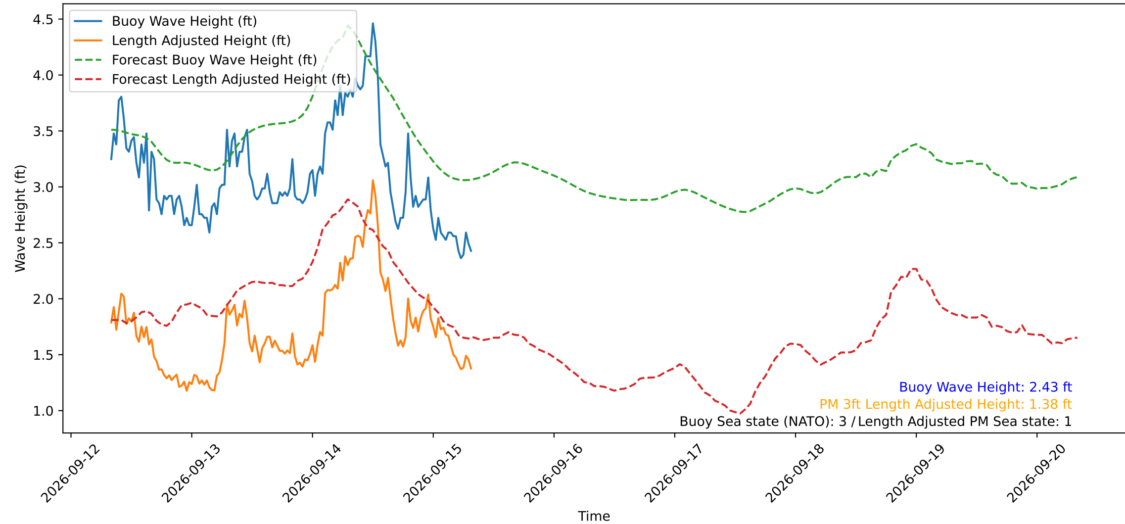
Wave Heights over Time for Oceanside Harbor at 2026-09-15 08:10:30
