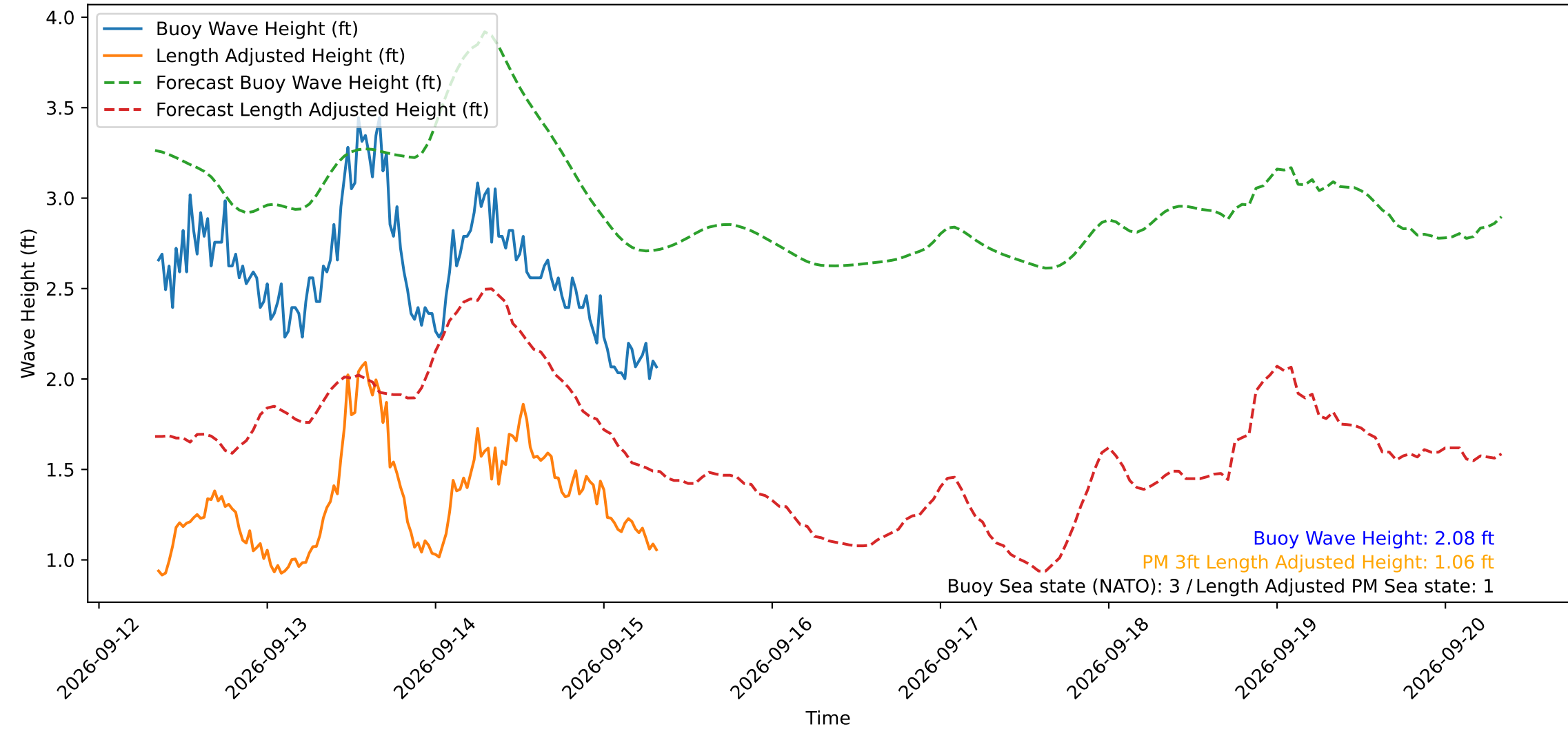
Wave Heights over Time for Red Beach at 2026-09-15 08:10:49
