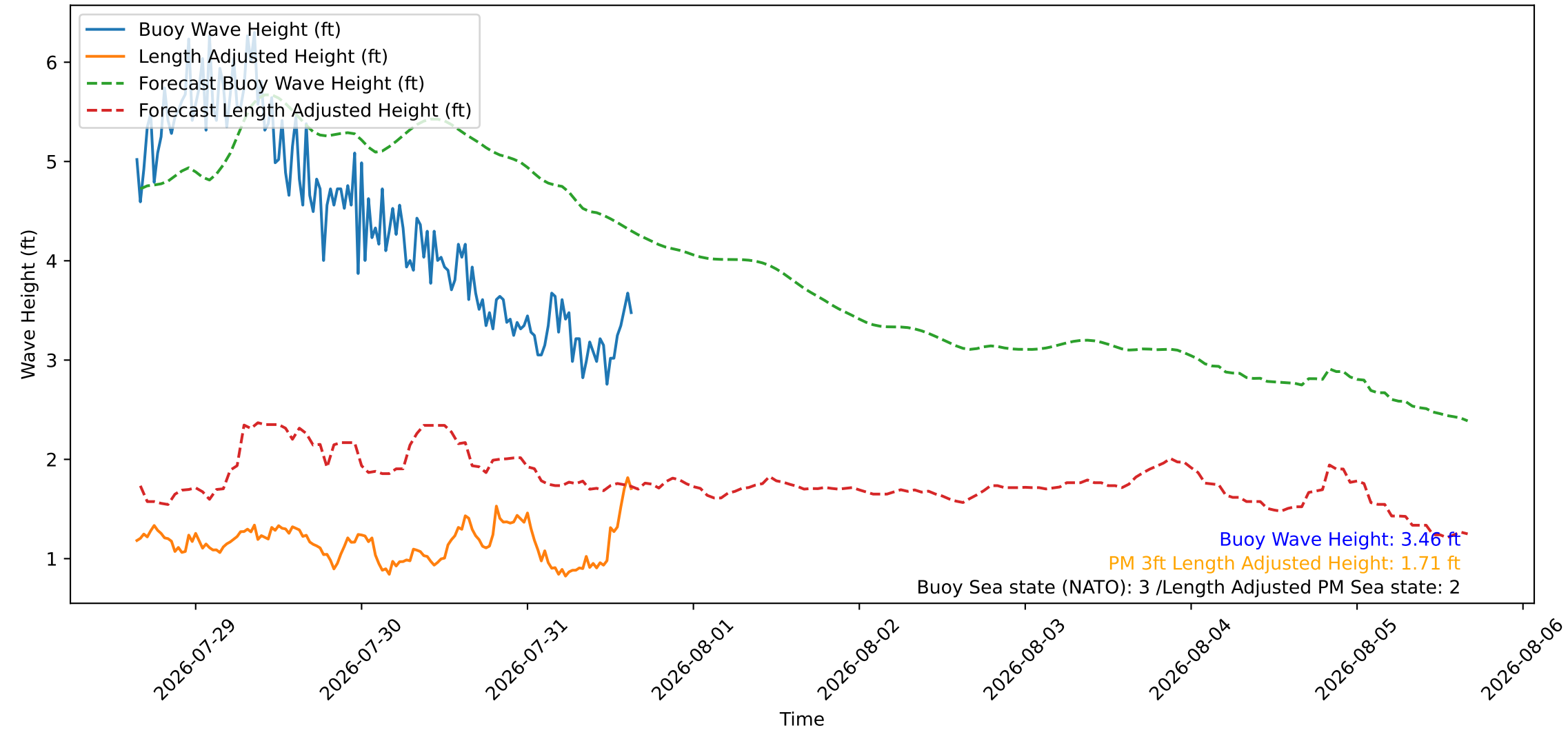
Wave Heights over Time for Green Beach at 2026-07-31 15:41:10
