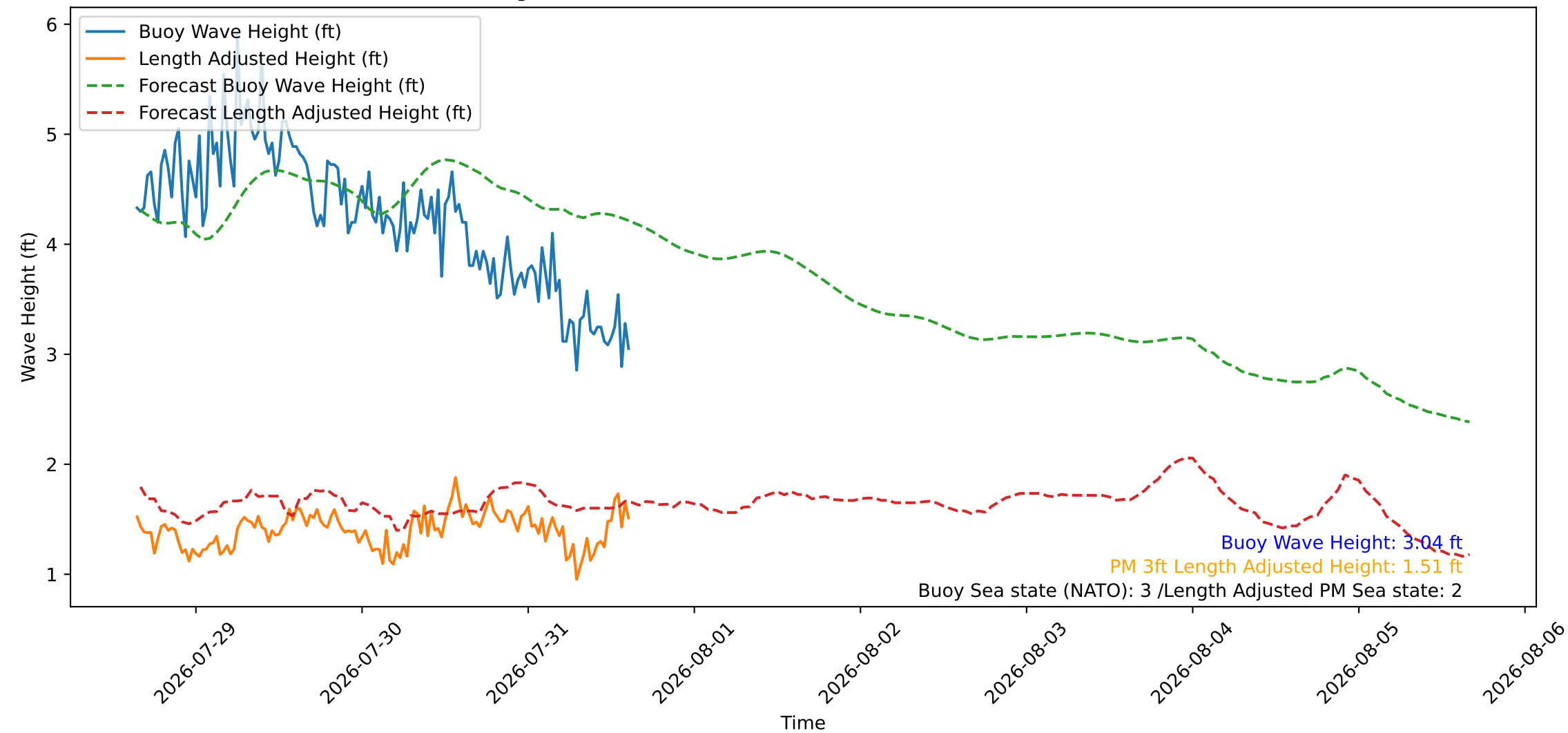
Wave Heights over Time for Oceanside Harbor at 2026-07-31 15:40:27
