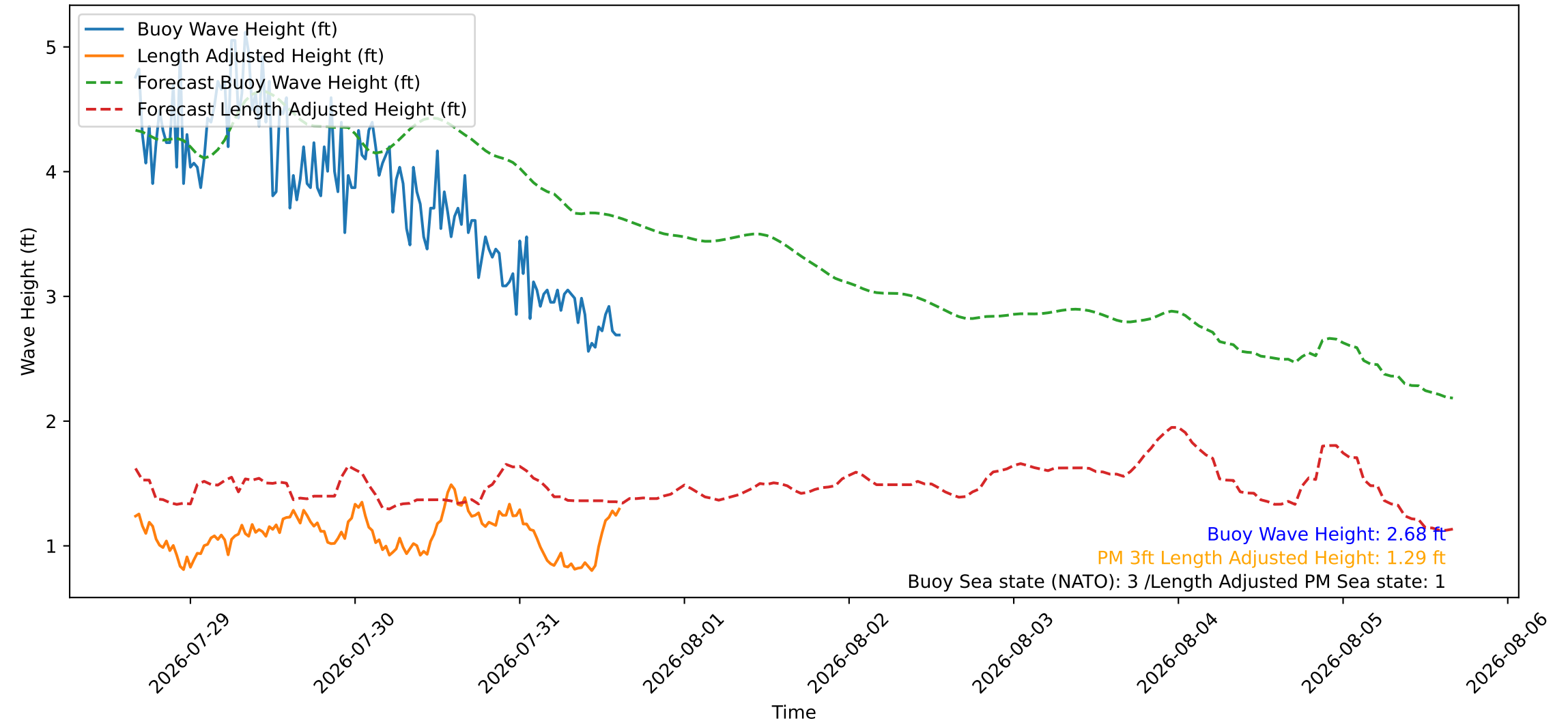
Wave Heights over Time for Red Beach at 2026-07-31 15:40:47
