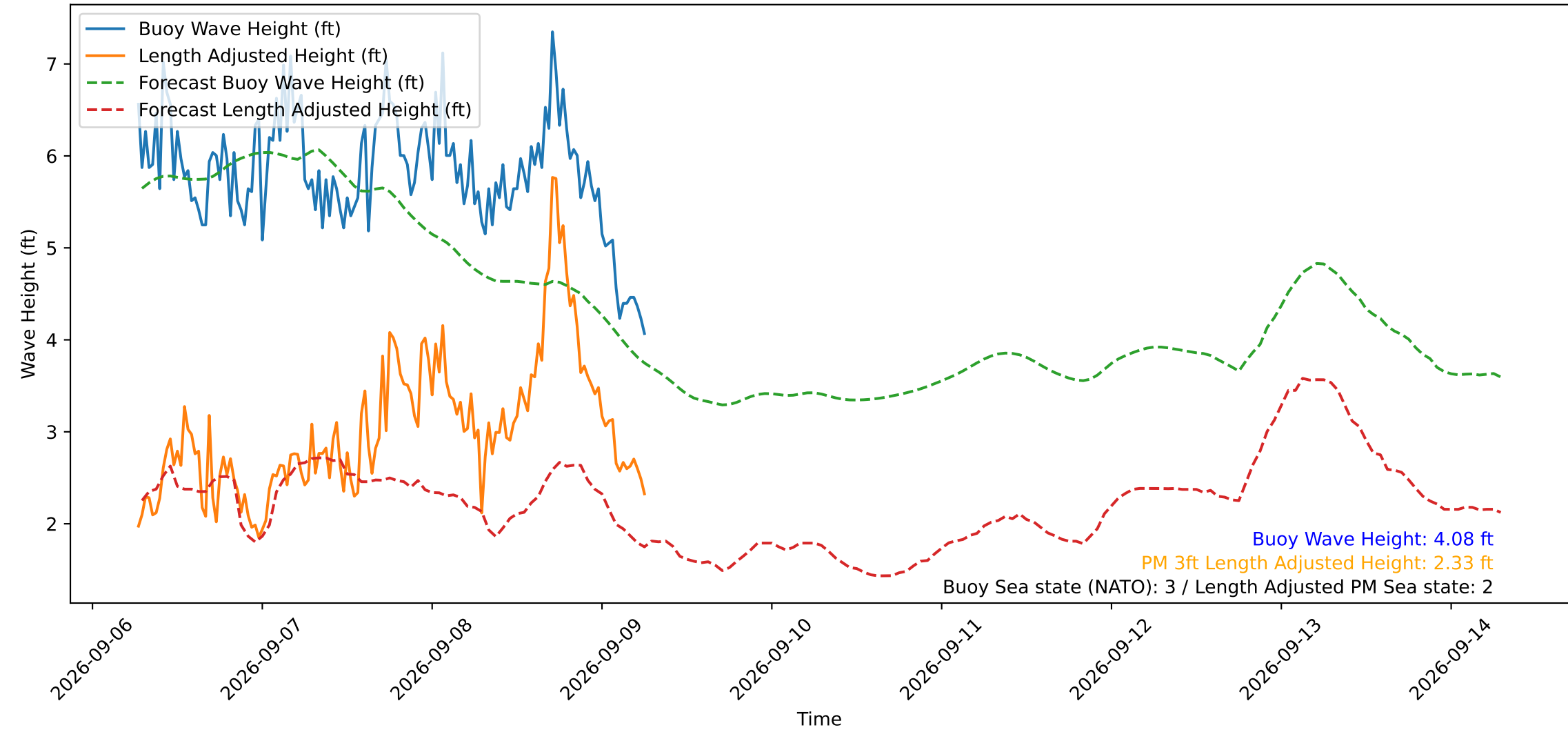
Wave Heights over Time for Oceanside Harbor at 2026-09-09 06:40:30
