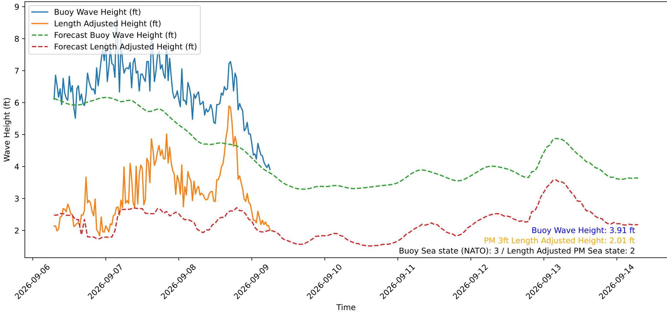
Wave Heights over Time for Green Beach at 2026-09-09 06:41:12
