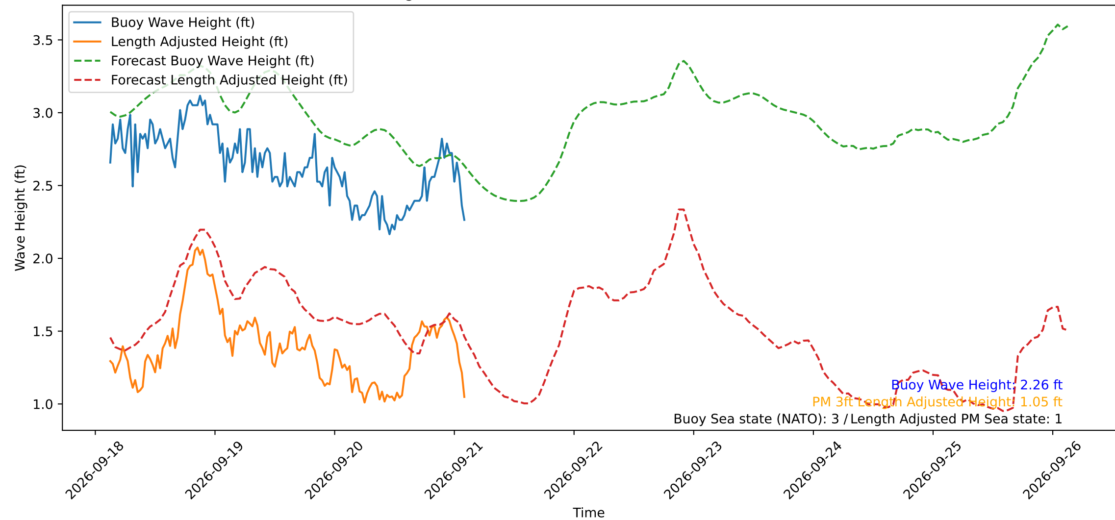
Wave Heights over Time for Green Beach at 2026-09-21 02:41:11
