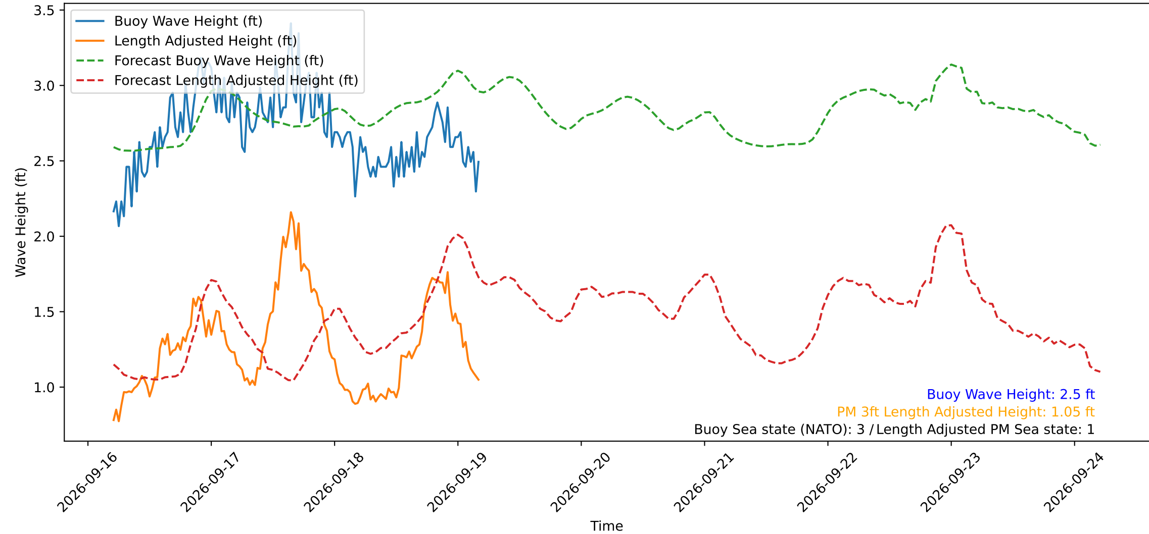
Wave Heights over Time for Red Beach at 2026-09-19 04:40:49
