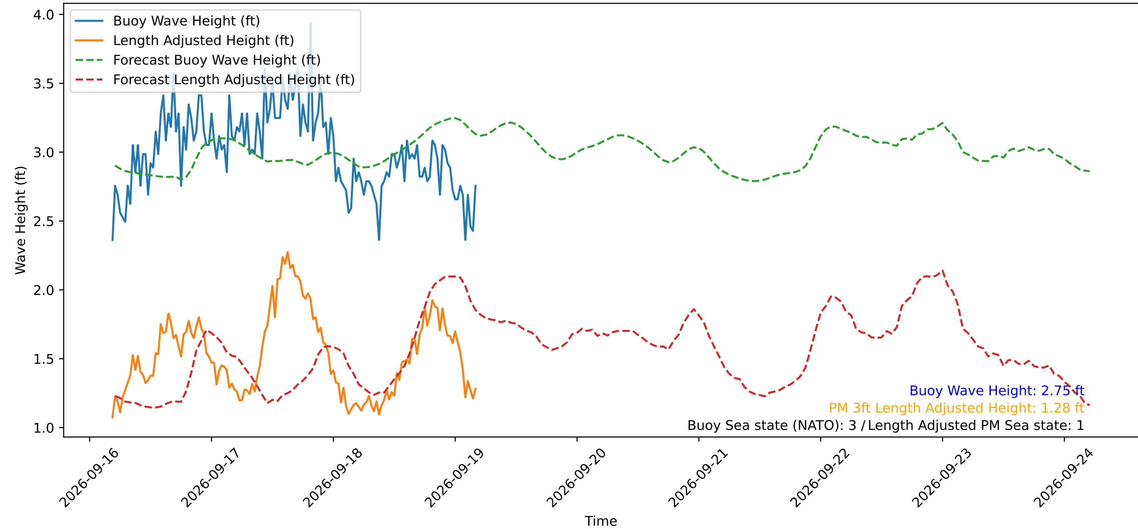
Wave Heights over Time for Oceanside Harbor at 2026-09-19 04:40:30
