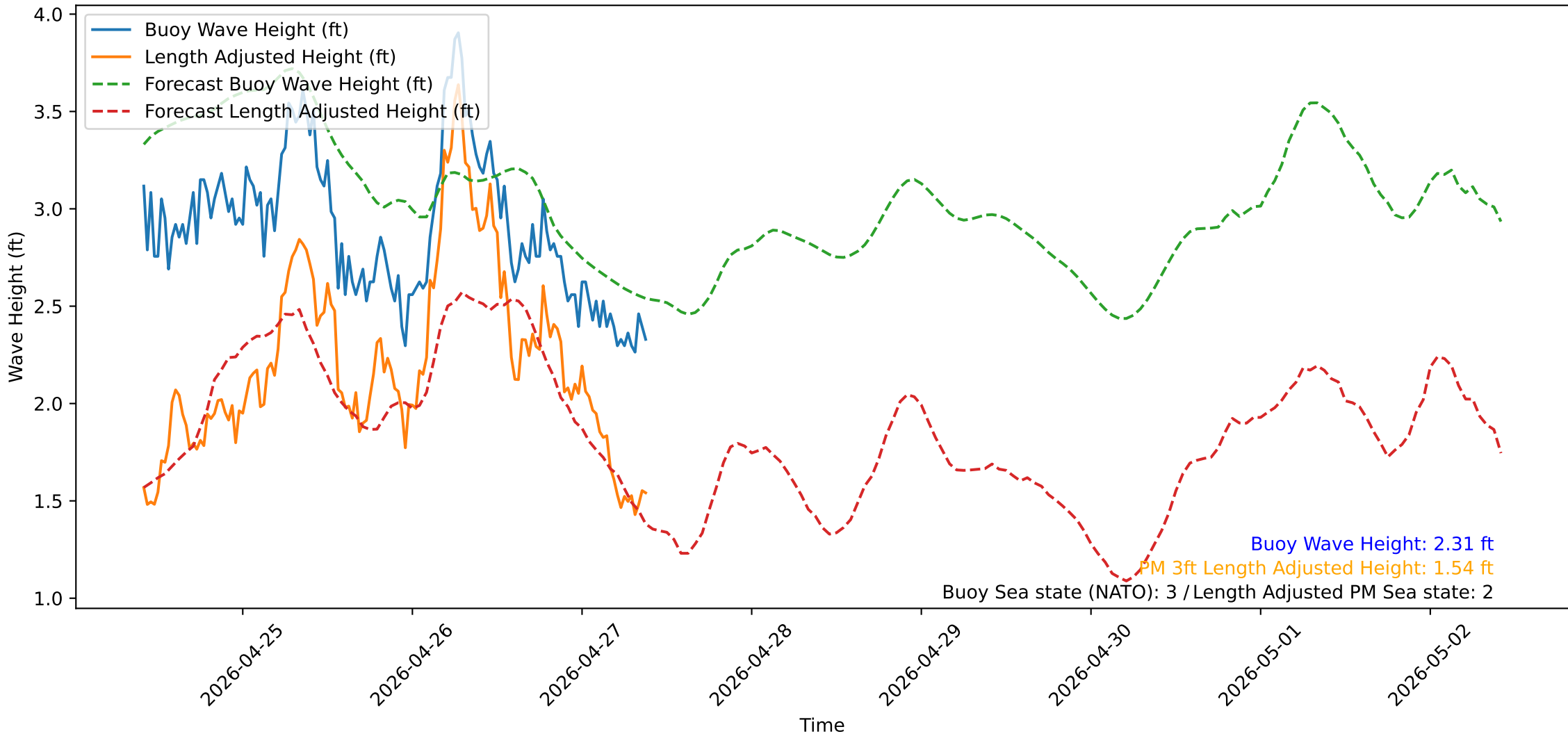
Wave Heights over Time for Oceanside Harbor at 2026-04-27 10:00:31
