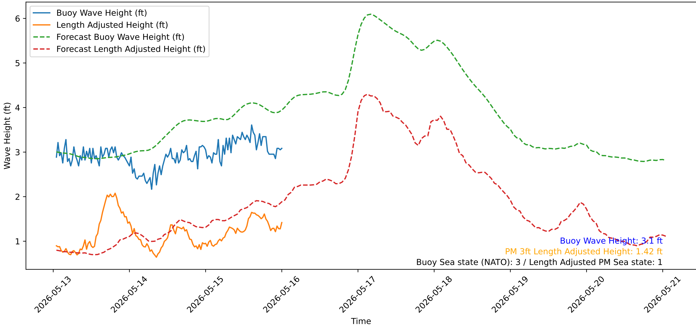
Wave Heights over Time for Oceanside Harbor at 2026-05-16 00:50:31
