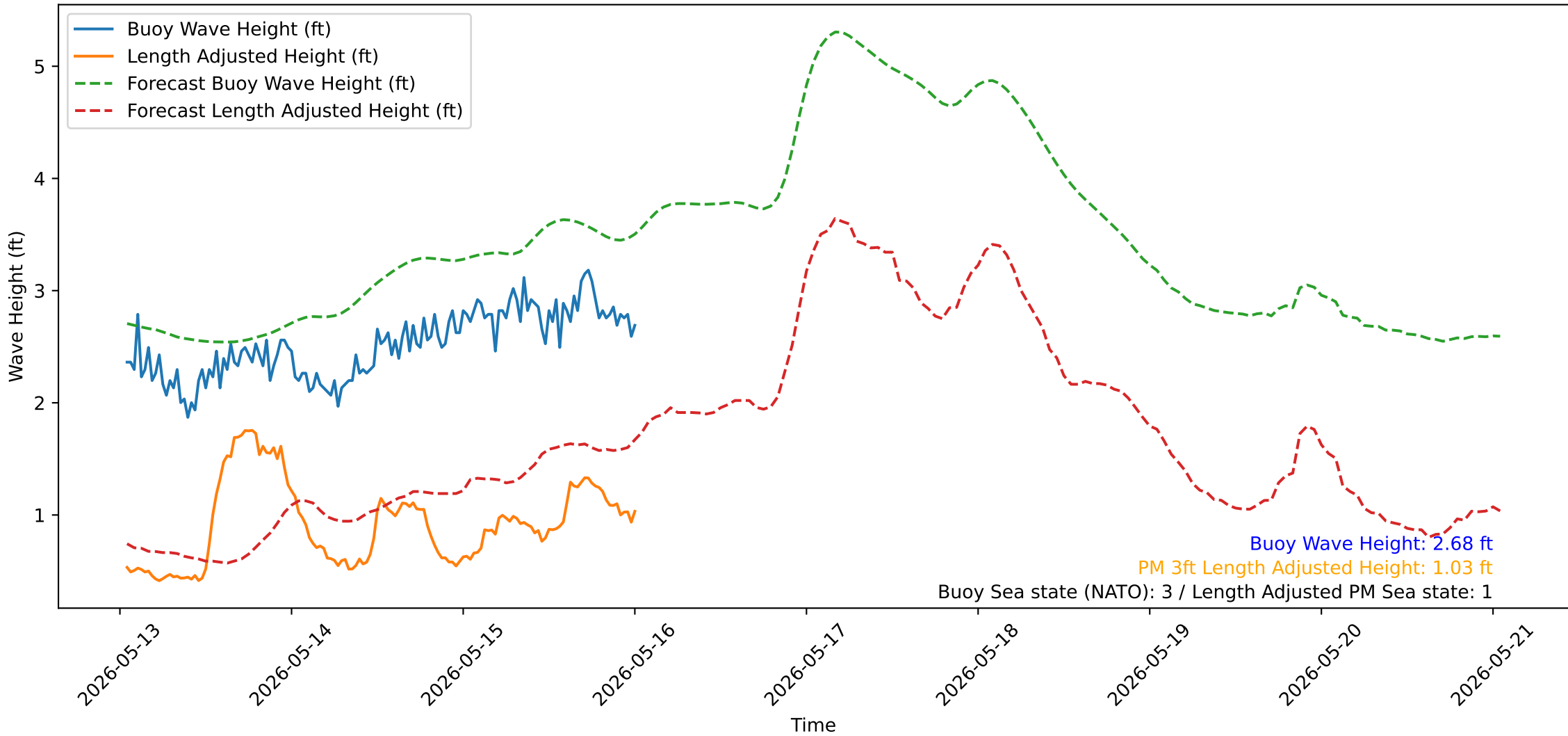
Wave Heights over Time for Red Beach at 2026-05-16 00:50:52
