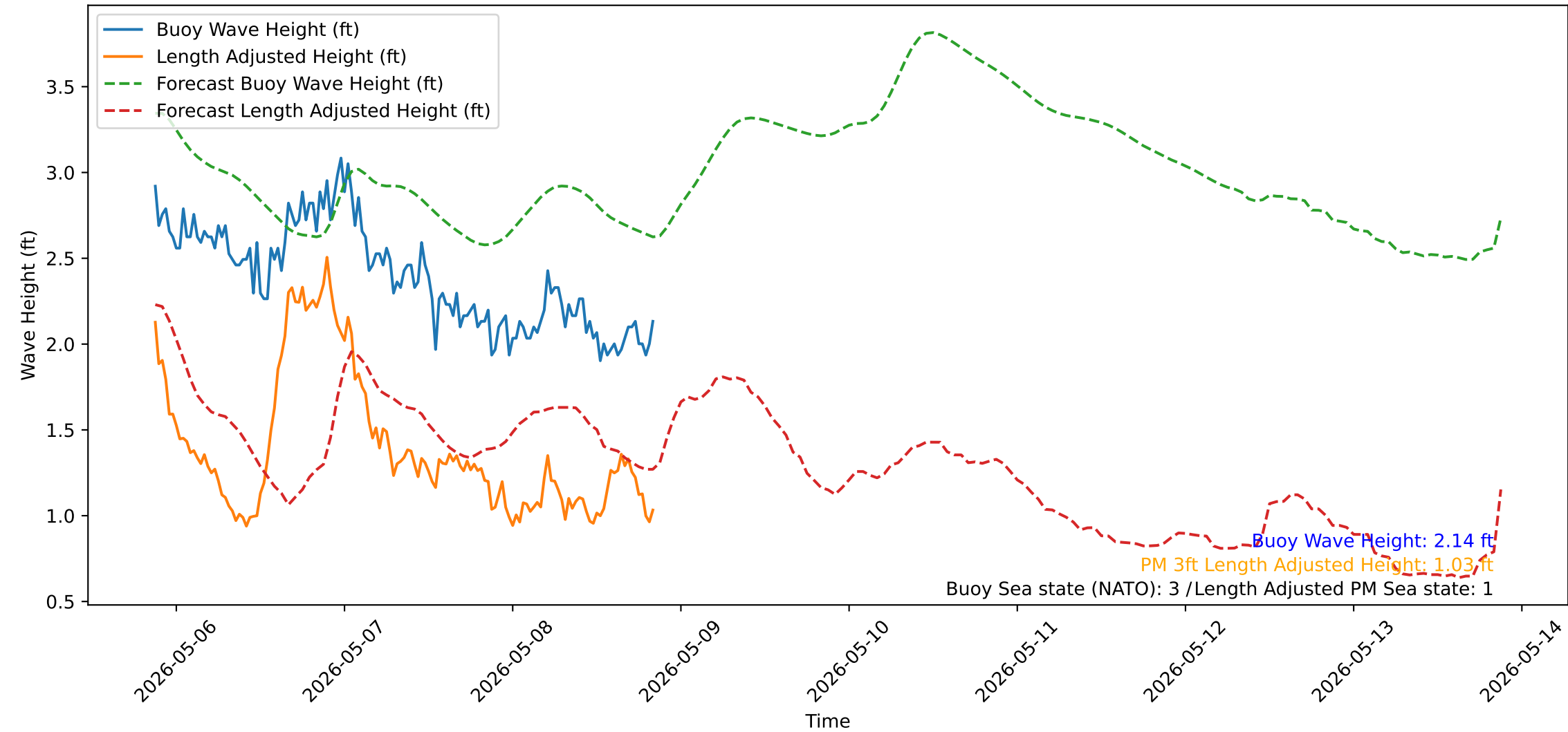
Wave Heights over Time for Red Beach at 2026-05-08 20:50:51
