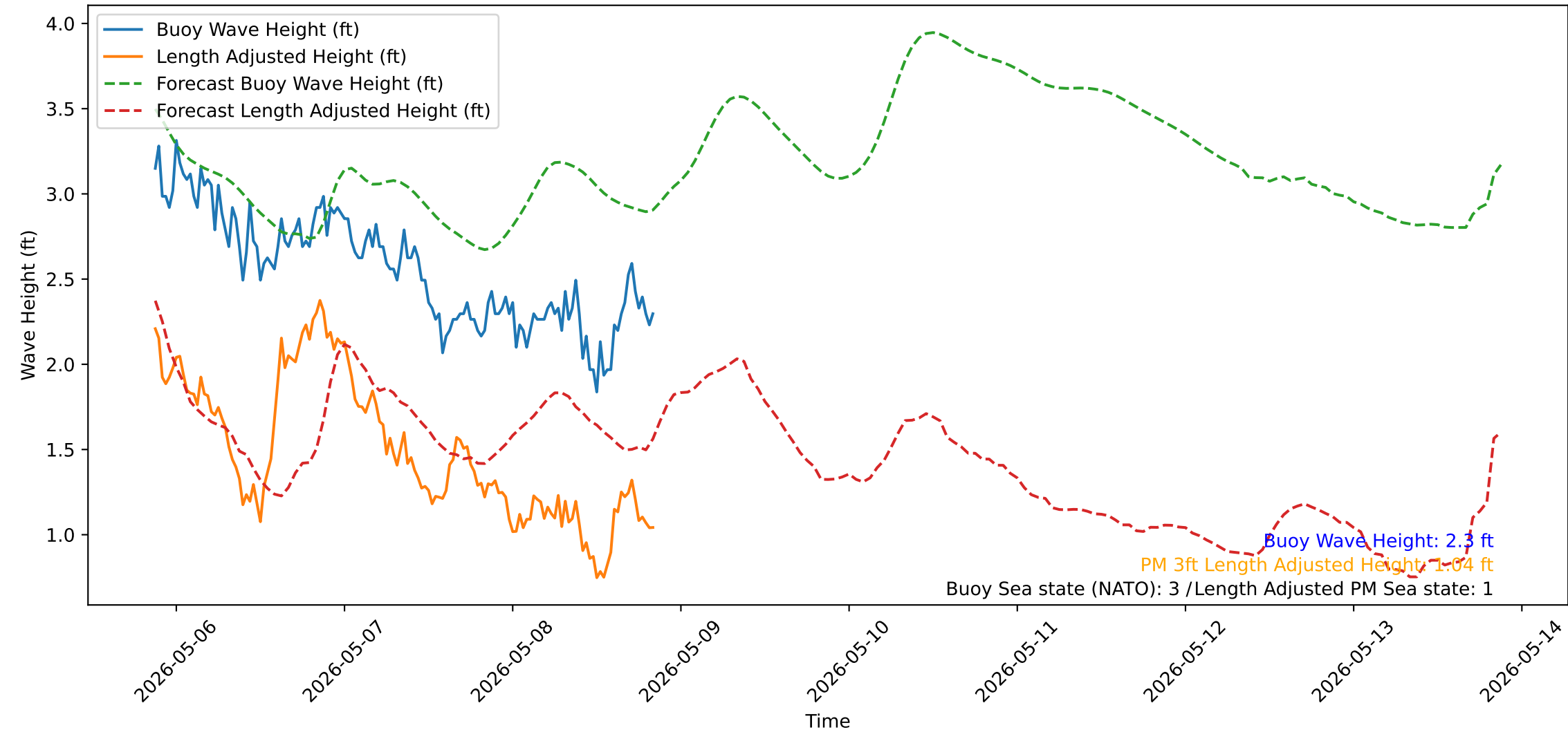
Wave Heights over Time for Green Beach at 2026-05-08 20:51:14
