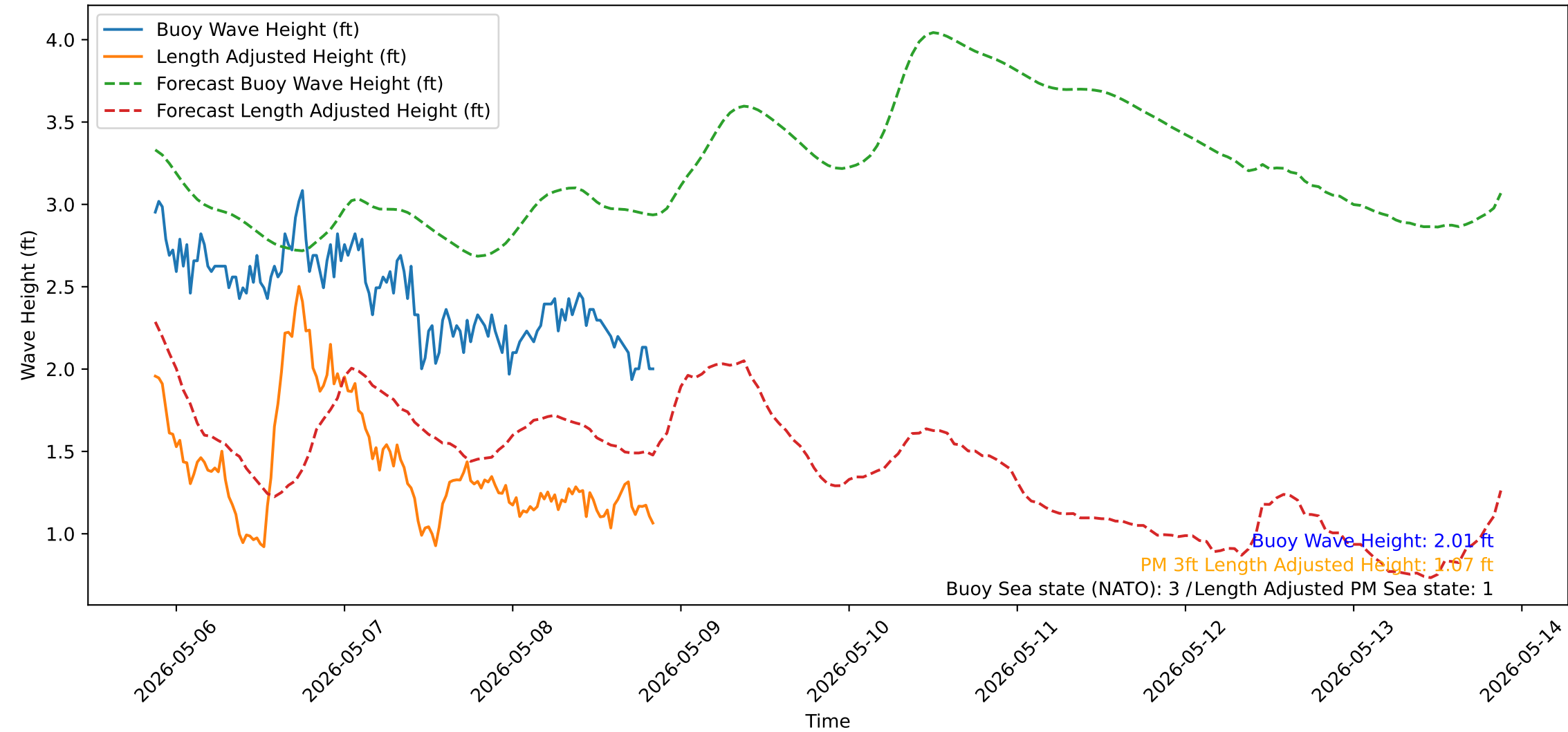
Wave Heights over Time for Oceanside Harbor at 2026-05-08 20:50:31
