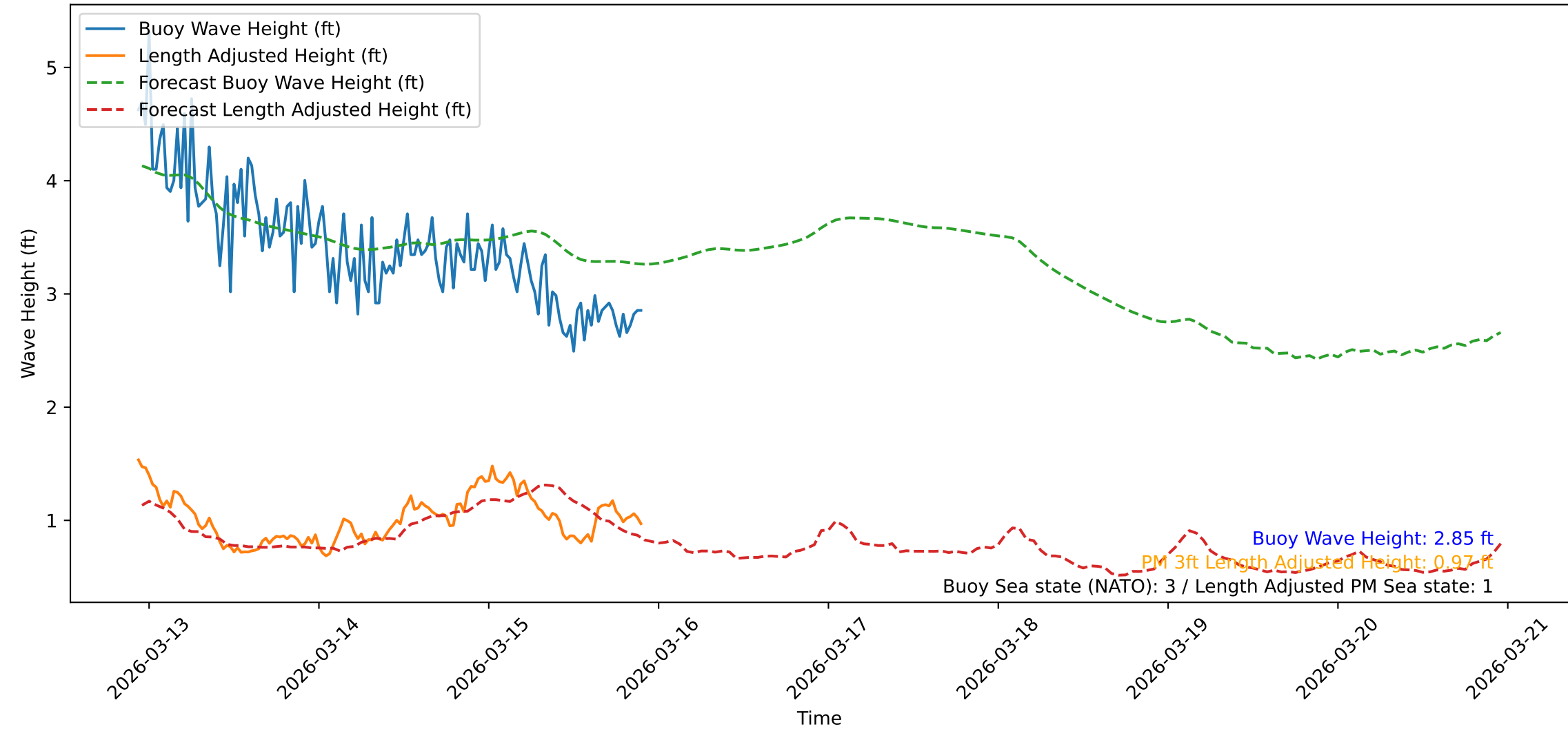
Wave Heights over Time for Oceanside Harbor at 2026-03-15 22:30:39
