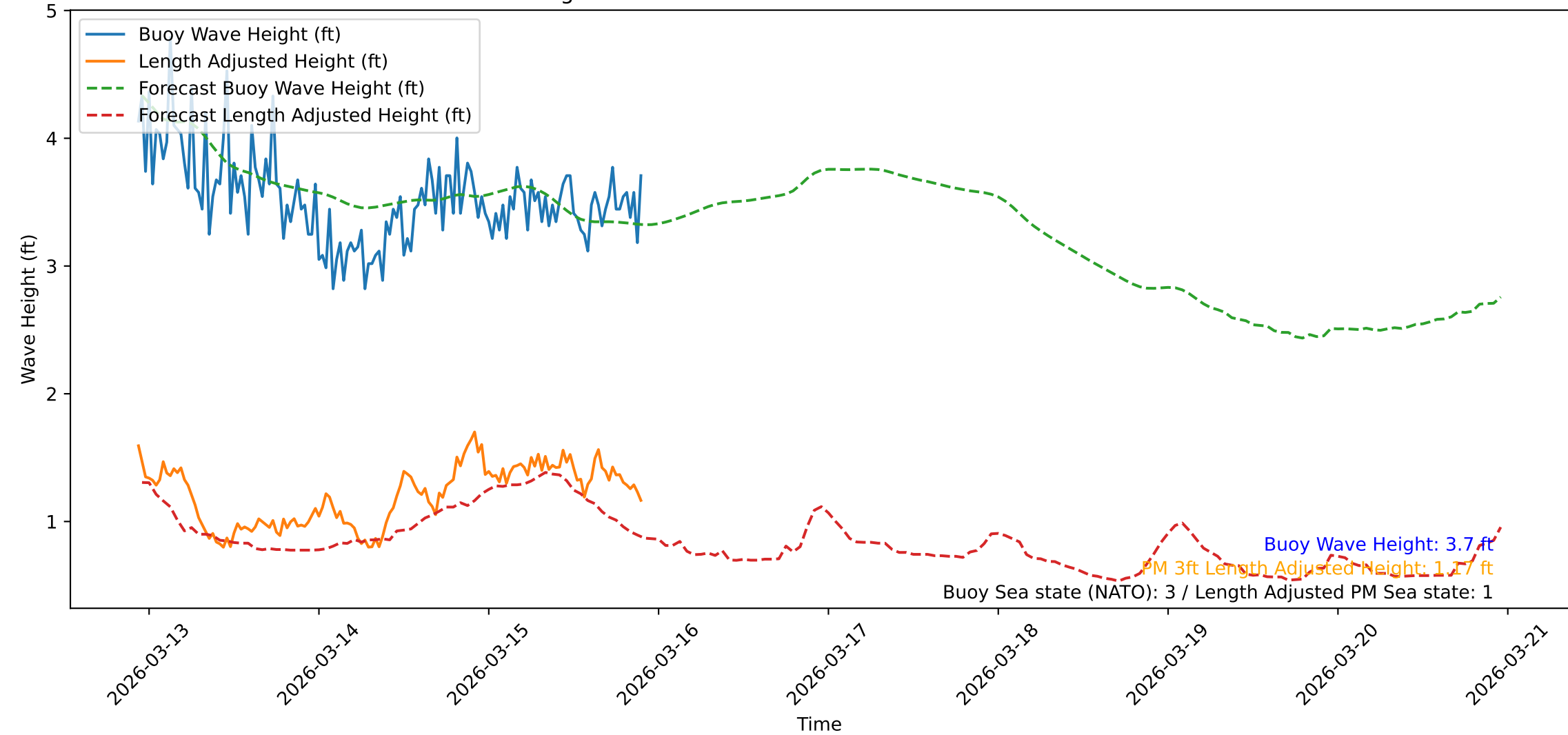
Wave Heights over Time for Green Beach at 2026-03-15 22:31:30
