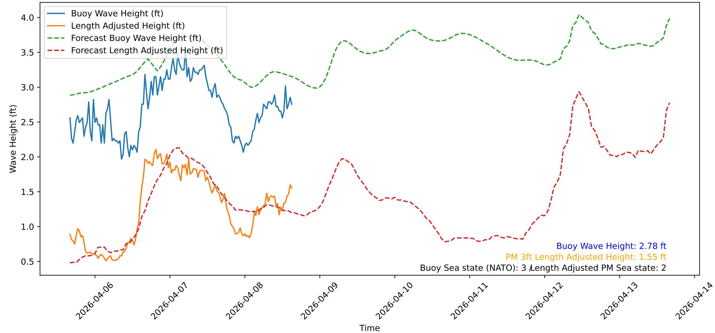
Wave Heights over Time for Red Beach at 2026-04-08 15:50:47
