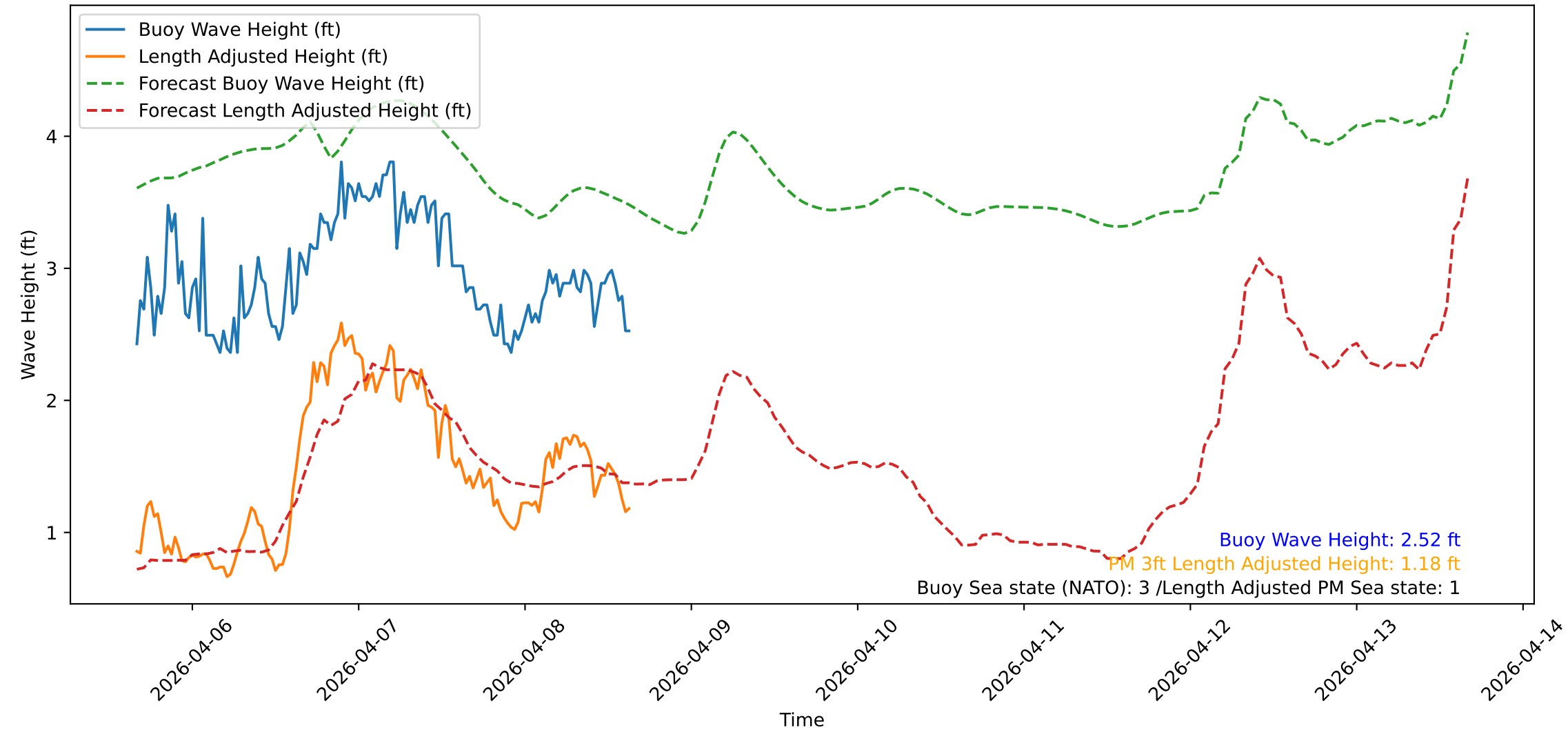
Wave Heights over Time for Green Beach at 2026-04-08 15:51:10
