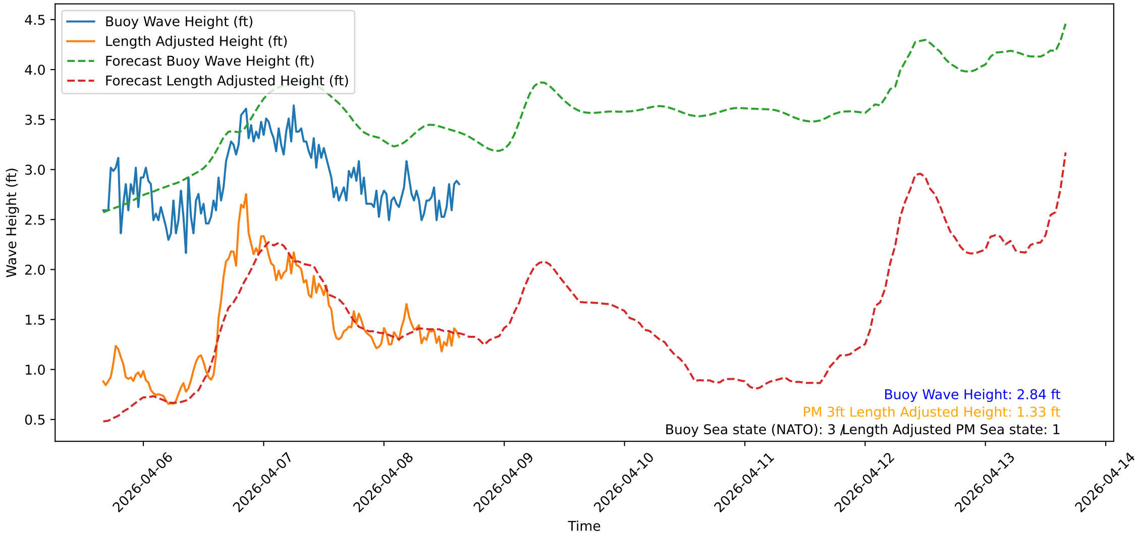
Wave Heights over Time for Oceanside Harbor at 2026-04-08 15:50:31
