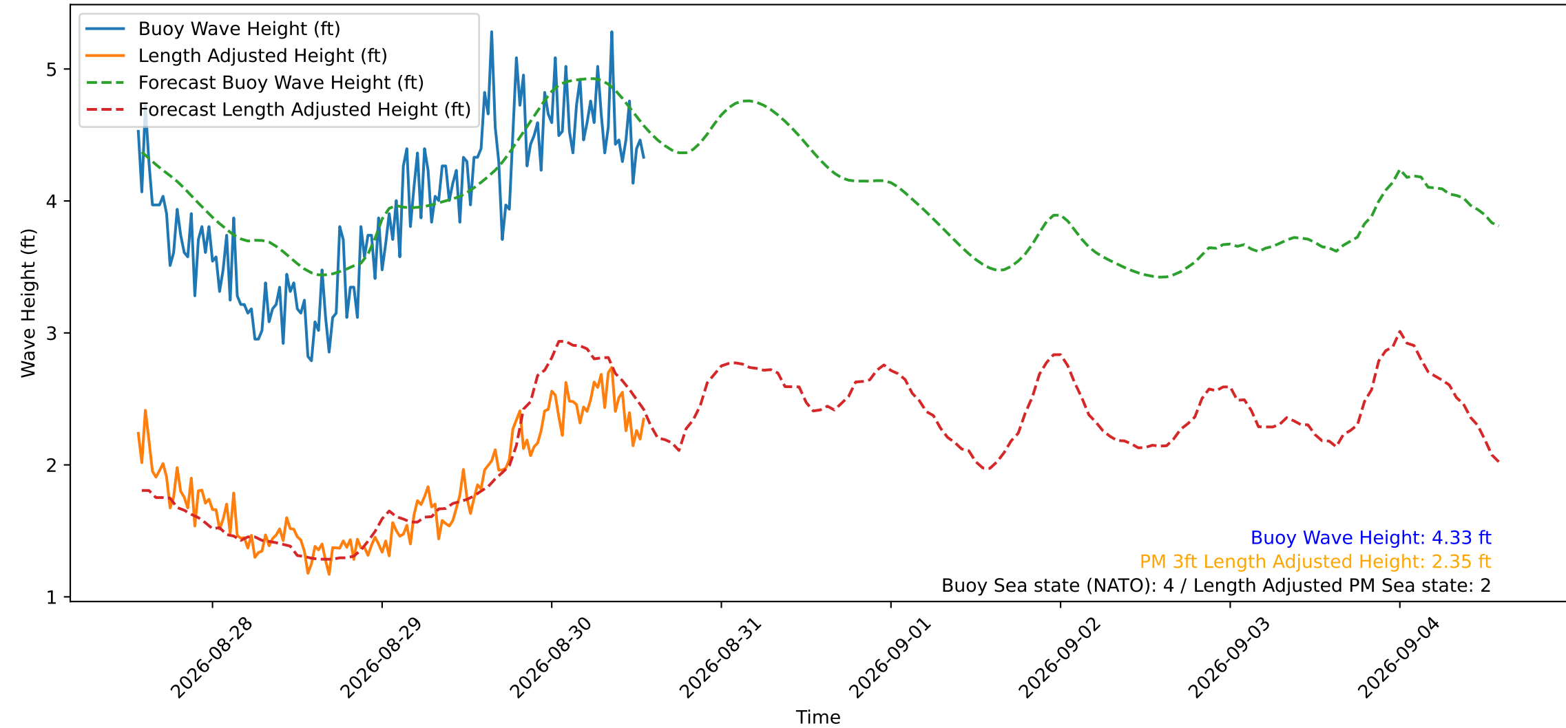
Wave Heights over Time for Oceanside Harbor at 2026-08-30 13:40:30
