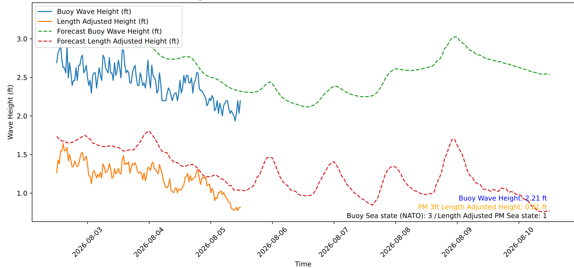
Wave Heights over Time for Oceanside Harbor at 2026-08-05 12:00:27
