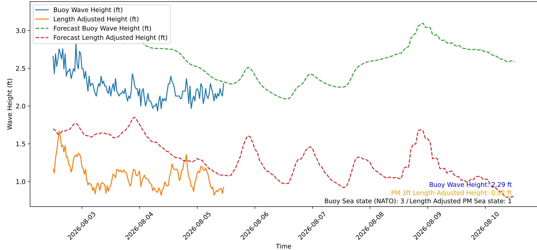
Wave Heights over Time for Green Beach at 2026-08-05 12:01:09
