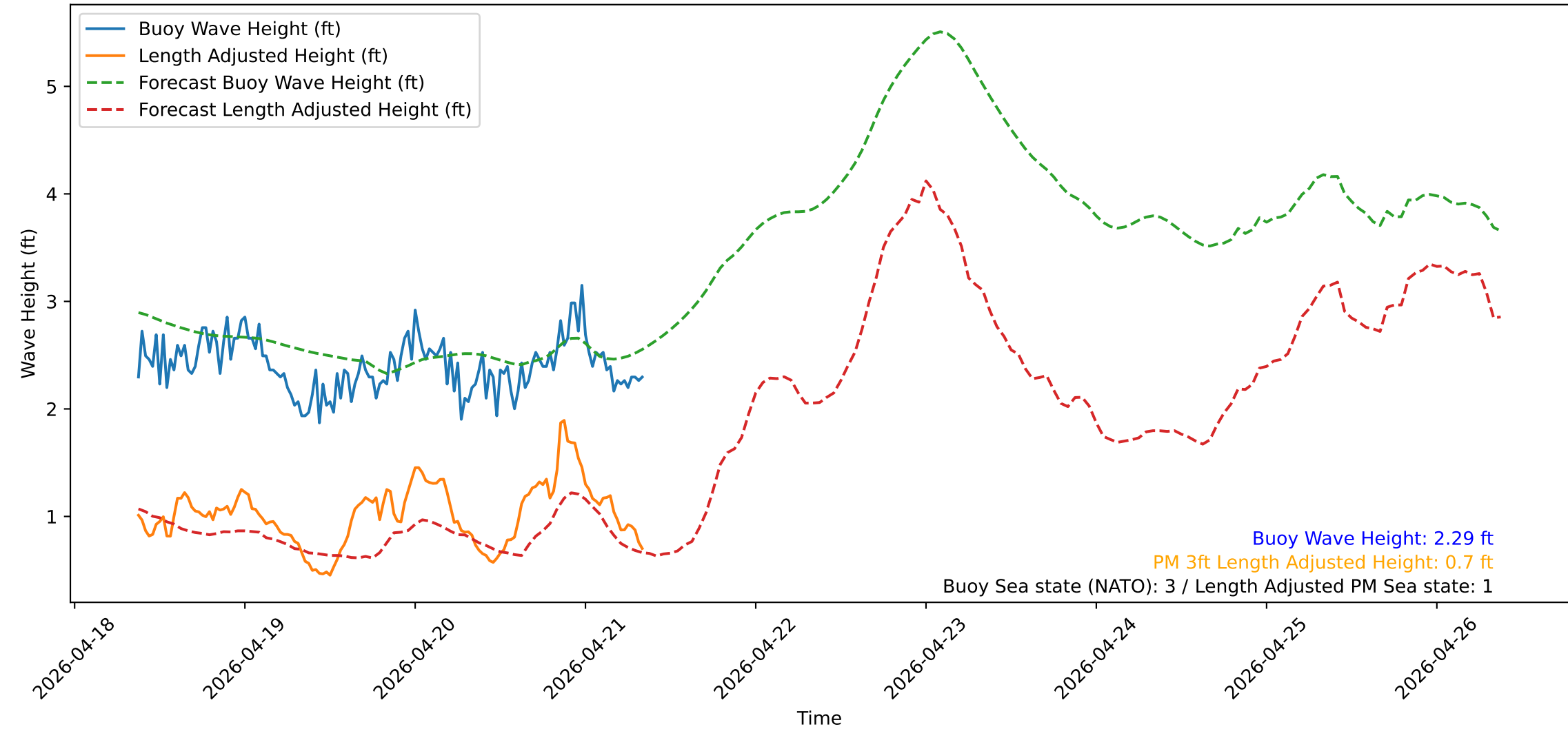
Wave Heights over Time for Green Beach at 2026-04-21 08:51:15
