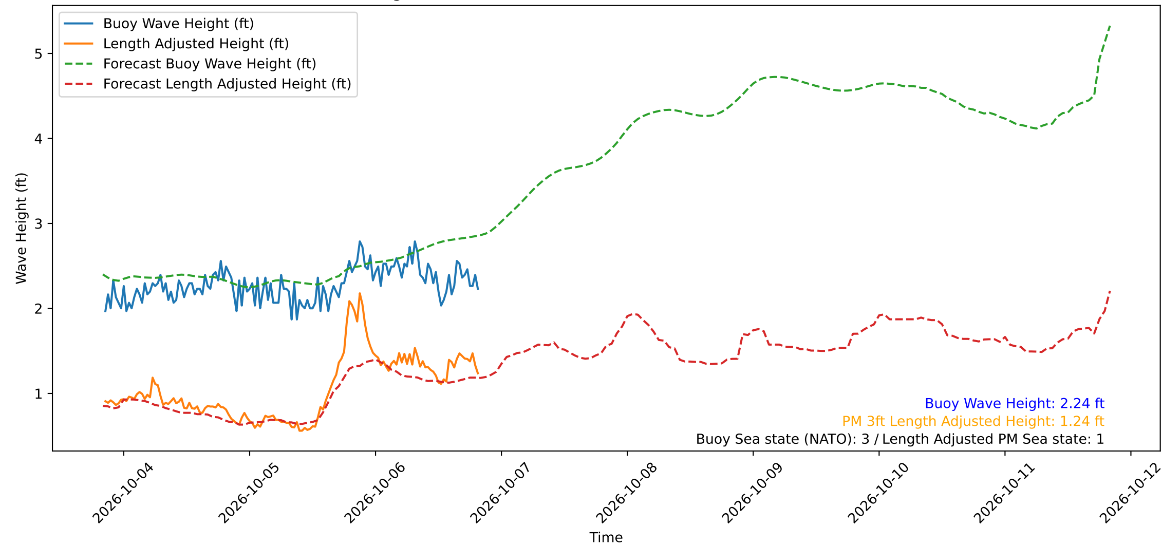
Wave Heights over Time for Oceanside Harbor at 2026-10-06 20:20:29
